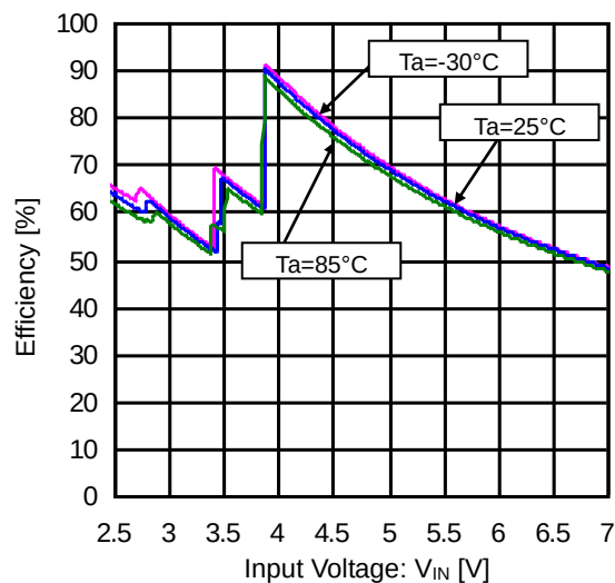
Figure 6. Efficiency vs Input Voltage (20mA x 6 Lights)
