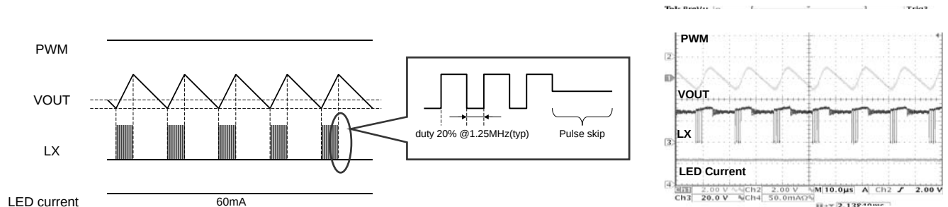
Figure 30. Pulse-skip
