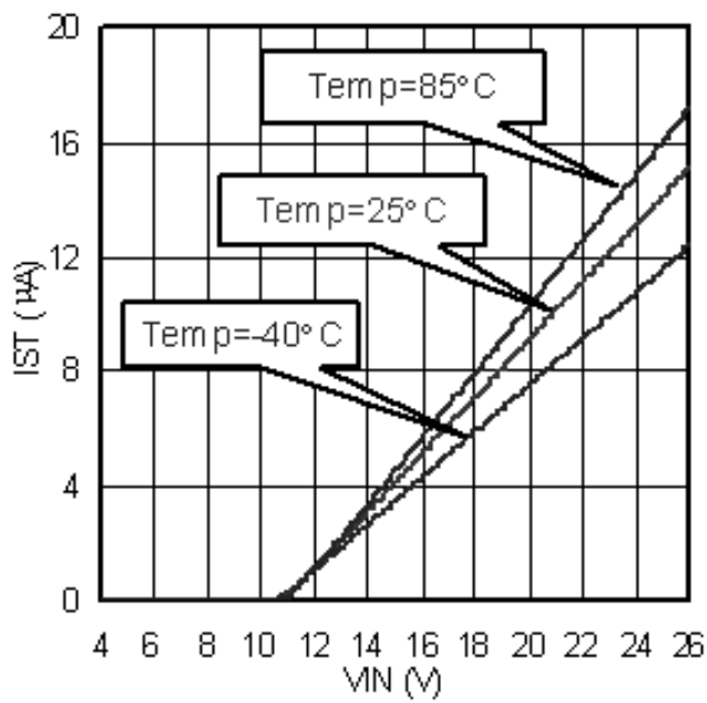
Figure 5. Quiescent Current
