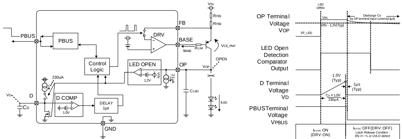
Figure 18. LED Open Detection Timing Chart
