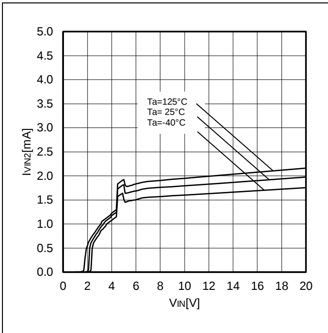
Figure 1. I_{VIN2} vs V_{IN}
