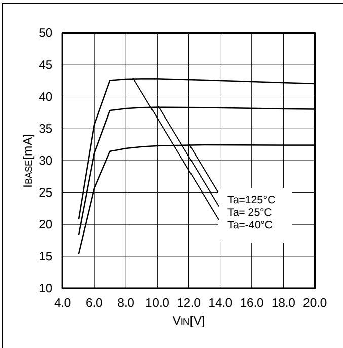
Figure 9. I_{BASE} VS V_{IN}
