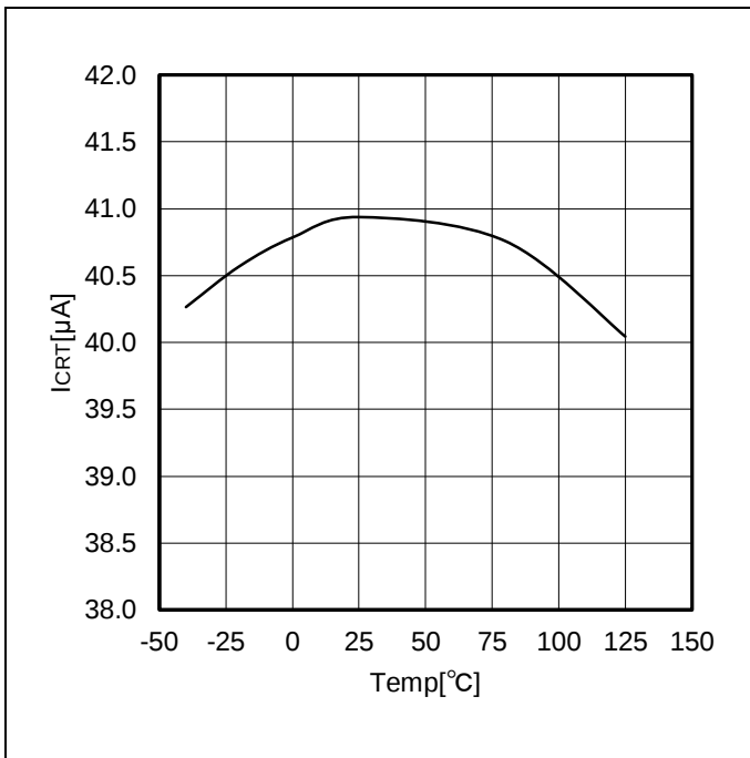
Figure 11. I_{CRT} VS Temp
