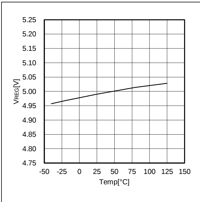
Figure 3. V_{REG} vs Temp
