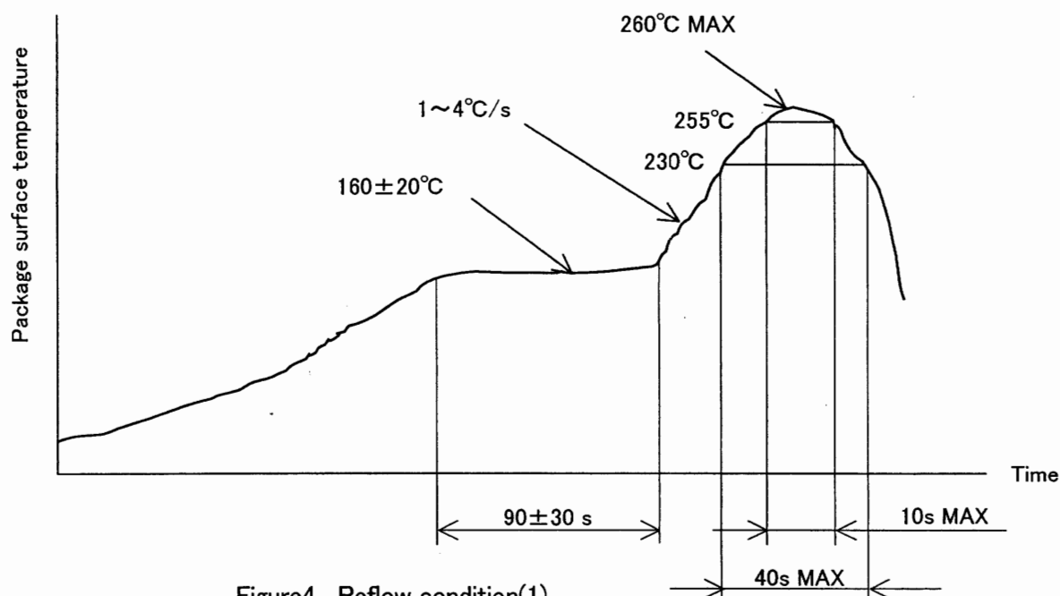
Figure4. Reflow condition(1)
