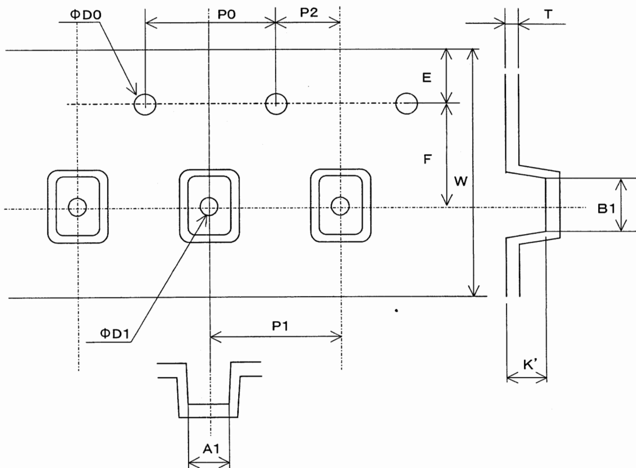
Figure8. Taping dimensions
