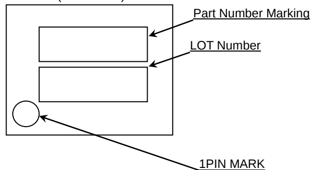
SOP16 (TOP VIEW)
