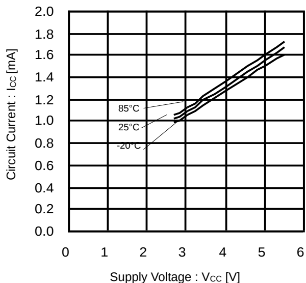
Figure 3. Circuit Current vs Supply Voltage (Active Current Consumption)
