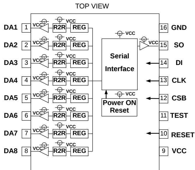
Figure 1. BH2226FV/BH2226F
