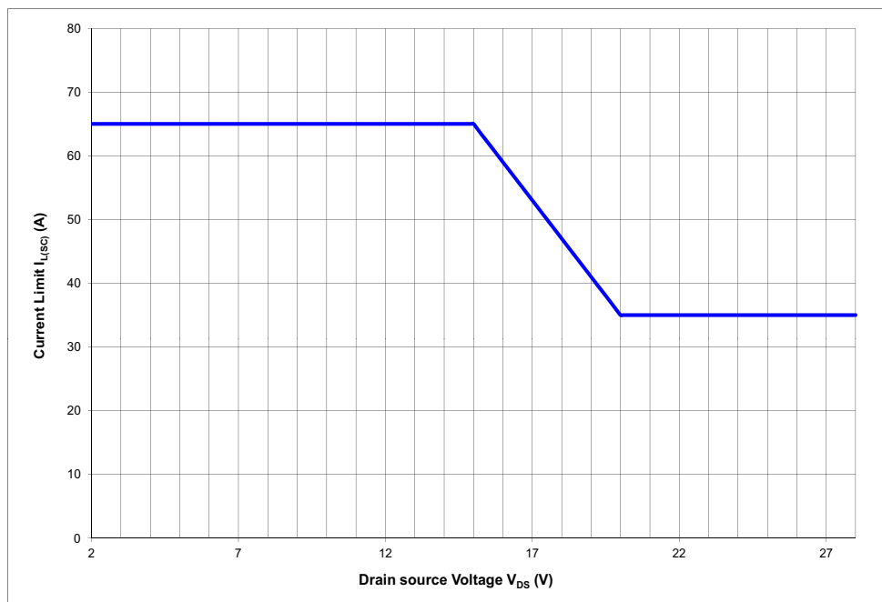
Figure 18 Current Limitation (typical behavior)
