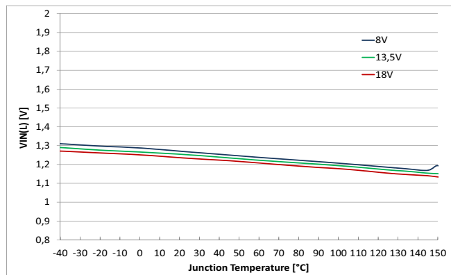
Figure 49 Input Voltage Threshold V_{IN(L)} = f(T_J; V_S)
