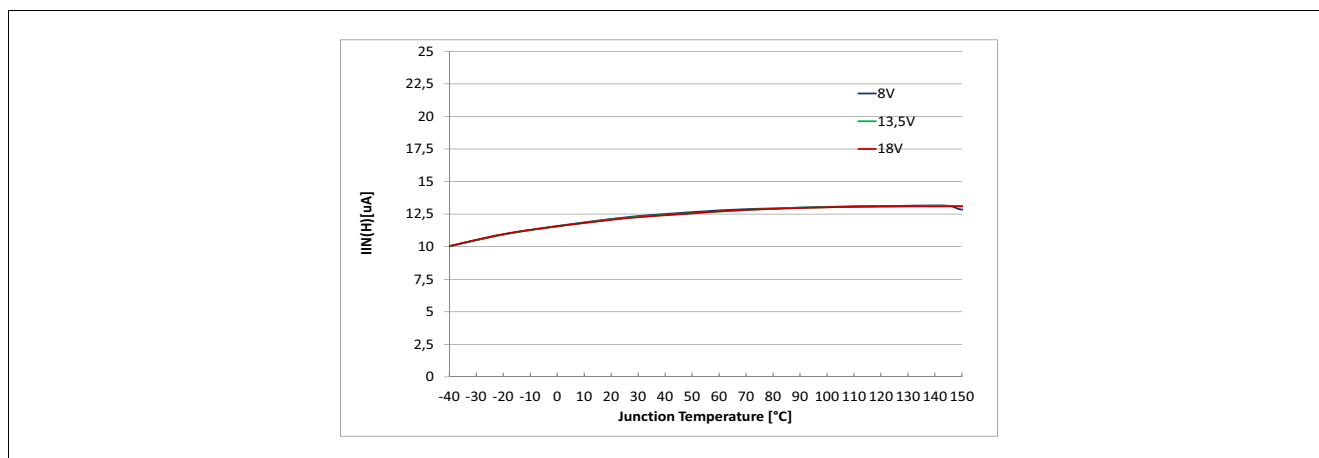
Figure 52 Input Current High Level I_{IN(H)} = f(T_J; V_S)
