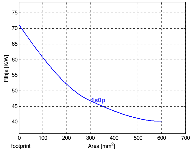
Figure 7 Typical Thermal Impedance. PCB set up 1s0p
