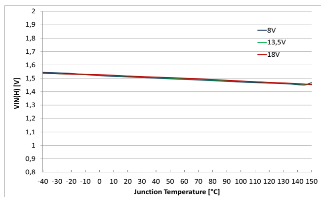
Figure 50 Input Voltage Threshold V_{IN(H)} = f(T_J; V_S)
