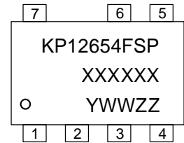
SOP-7
