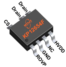
SOP-7
