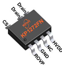
SOP-7
