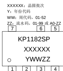
SOP-7
