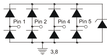
Device Schematic
