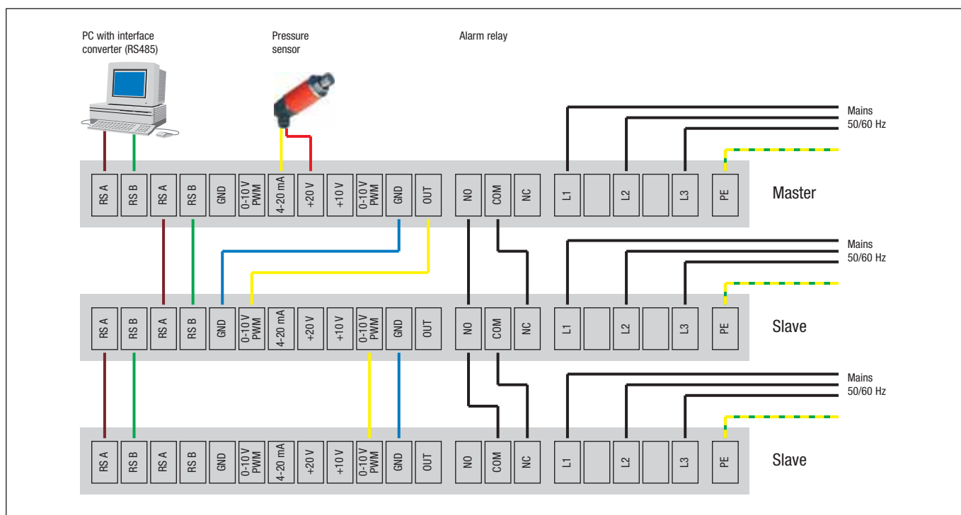
Connection diagram: Condensing pressure control with master-slave fans
