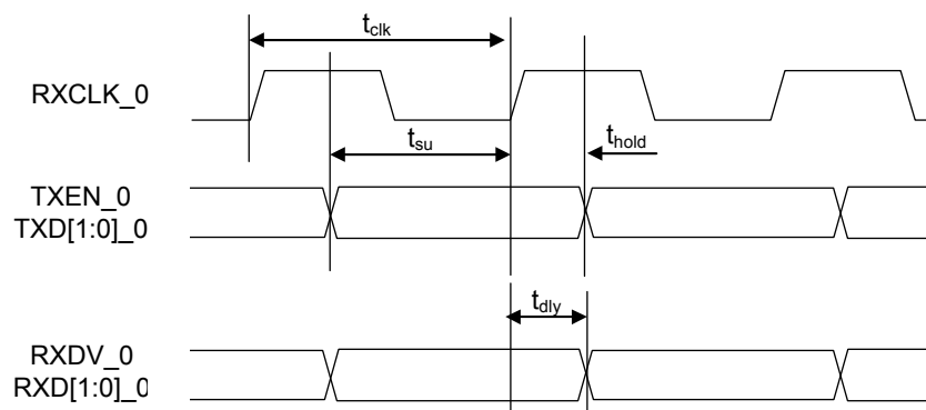
Figure 4-4 RMII timing
