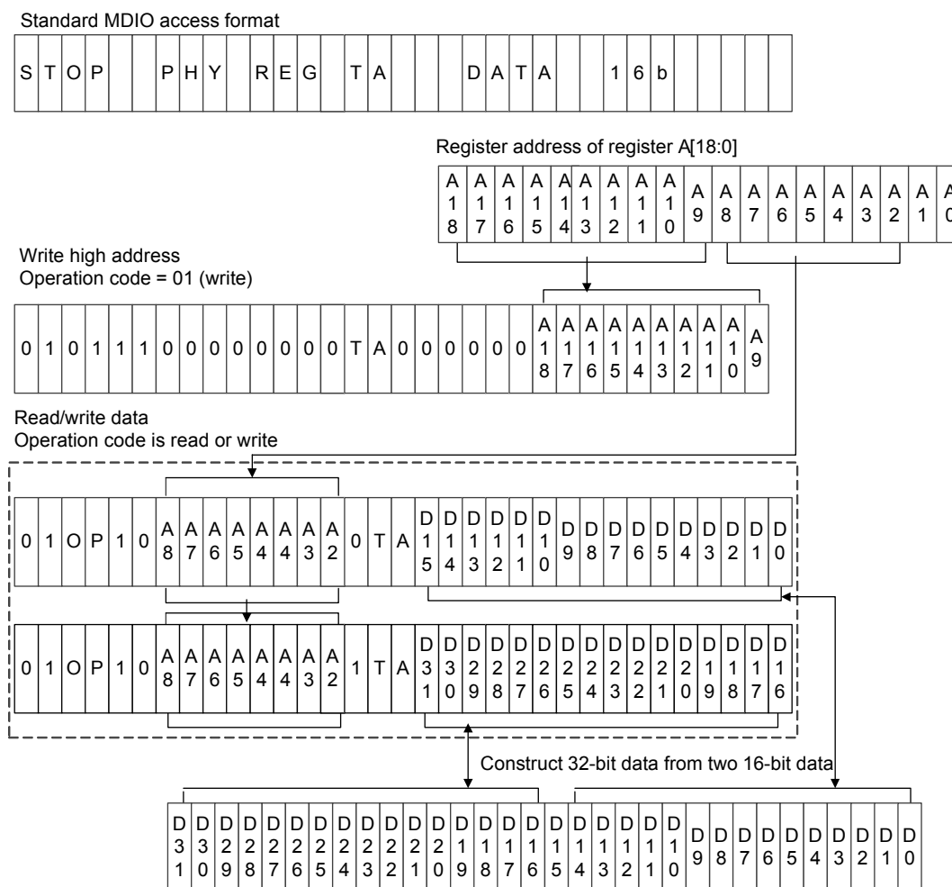
Figure 3-3 MDC/MDIO access format
