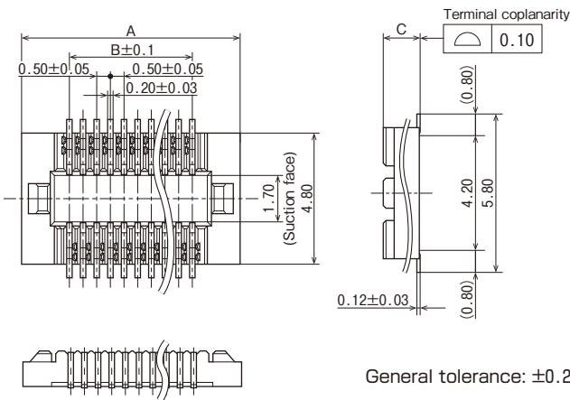
External dimensions
