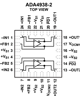
Figure 2. ADA4938-2 Functional Block Diagram
