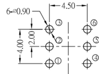
P.C.B.LAYOUT(TOP VIEW)
