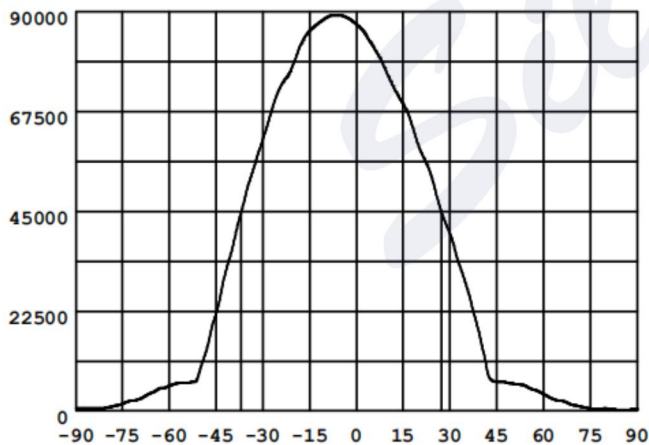
Luminous angle
