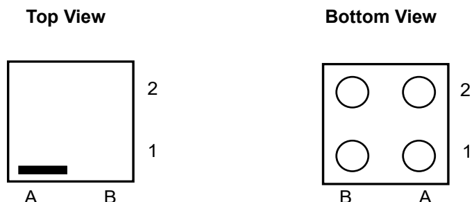
RP123Z (WLCSP-4-P8 / WLCSP-4-P12) Pin Configuration
