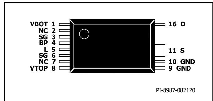
Figure 5. Pin Configuration.
