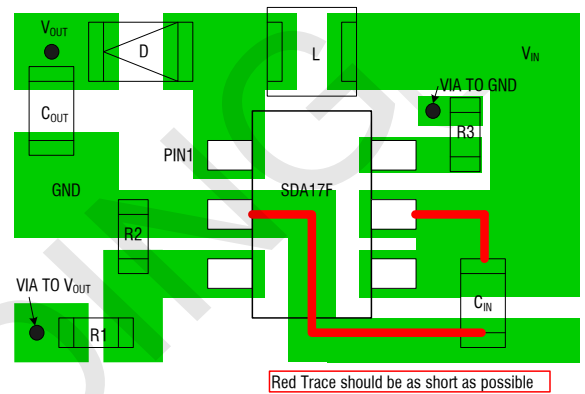
Figure 3. SDA17F Suggested Layout
