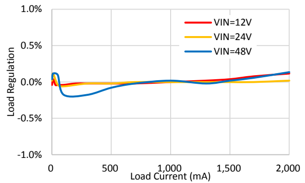
Load Regulation @ 1MHz
