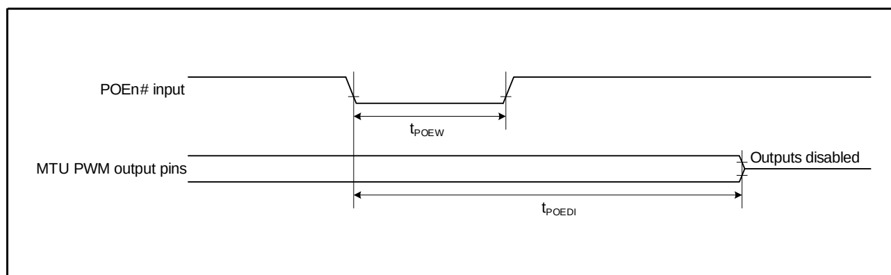
Figure 32.22 Output Disable Time for POE in Response to Transition of the POE# Signal Level (n = 0, 8, 10)
