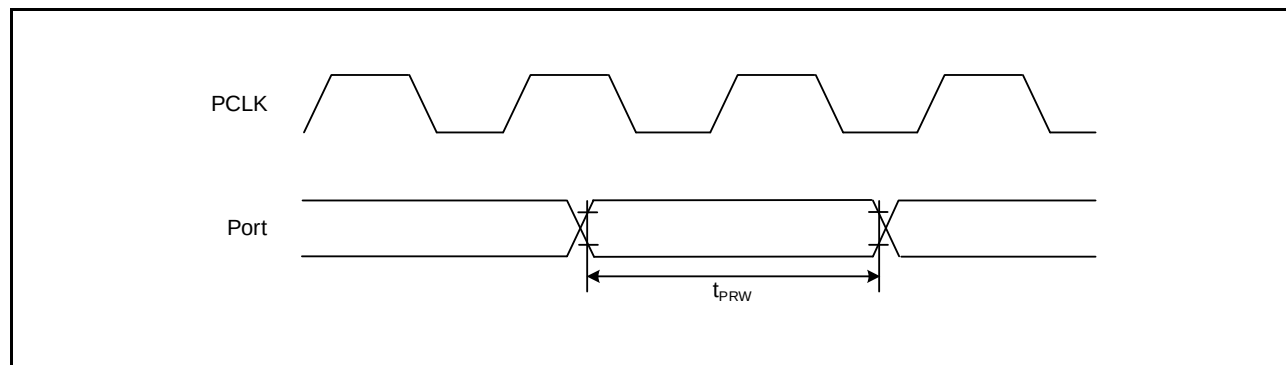
Figure 32.18 I/O Port Input Timing
