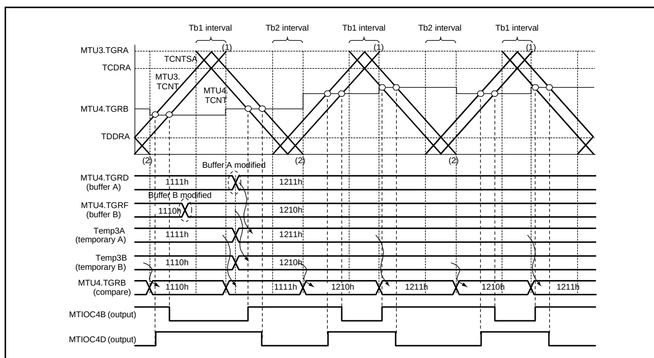
Figure 19.74 Example of Double Buffer Operation
