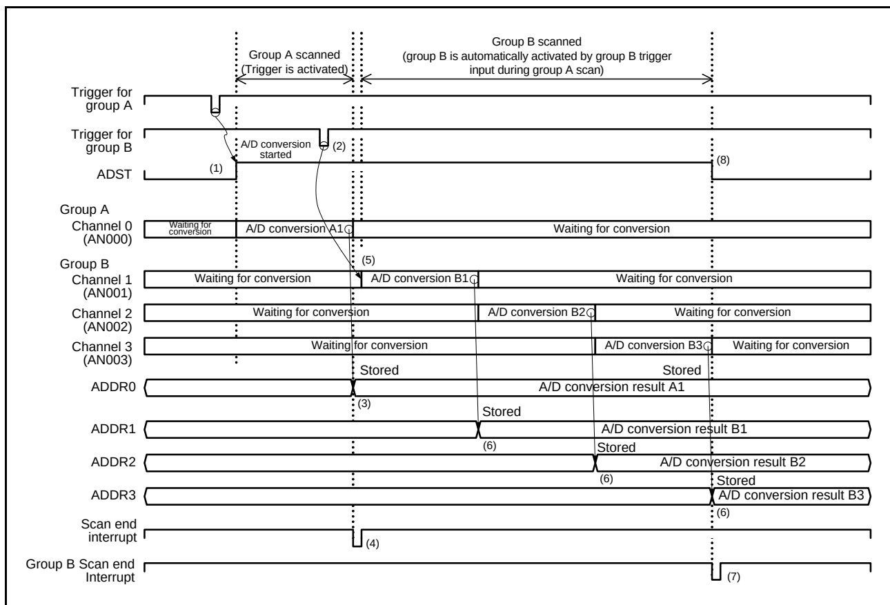
Figure 26.18 Example 3 of Group Priority Operation: Group B Trigger Input during Group A Scan, With Rescan Setting (ADGSPCR.GBRSCN = 1, ADGSPCR.GBRP = 0, ADGSPCR.LGRRS = 0)
