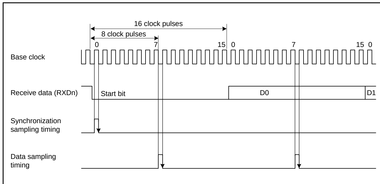
Figure 23.5 Receive Data Sampling Timing in Asynchronous Mode
