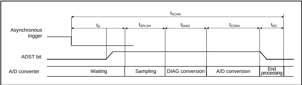
Figure 26.27 Scan Conversion Timing (Activated by Asynchronous Trigger)
