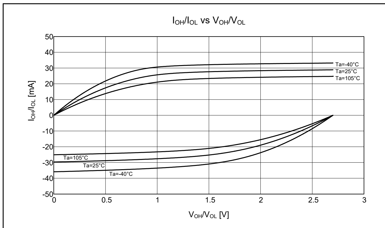
Figure 5.19 V_{OH}/V_{OL} and I_{OH}/I_{OL} Temperature Characteristics at V_{CC} = 2.7 V When High-Drive Output is Selected (Reference Data)
