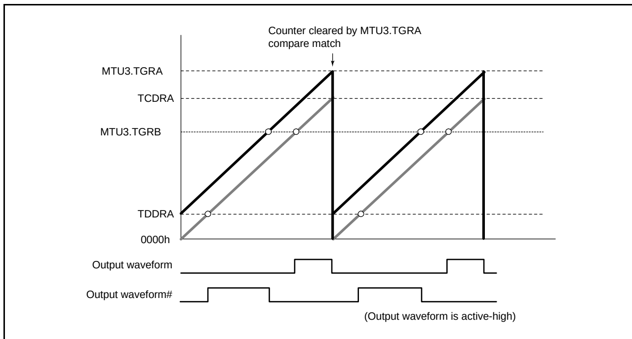
Figure 19.69 Example of Counter Clearing Operation by MTU3.TGRA Compare Match
