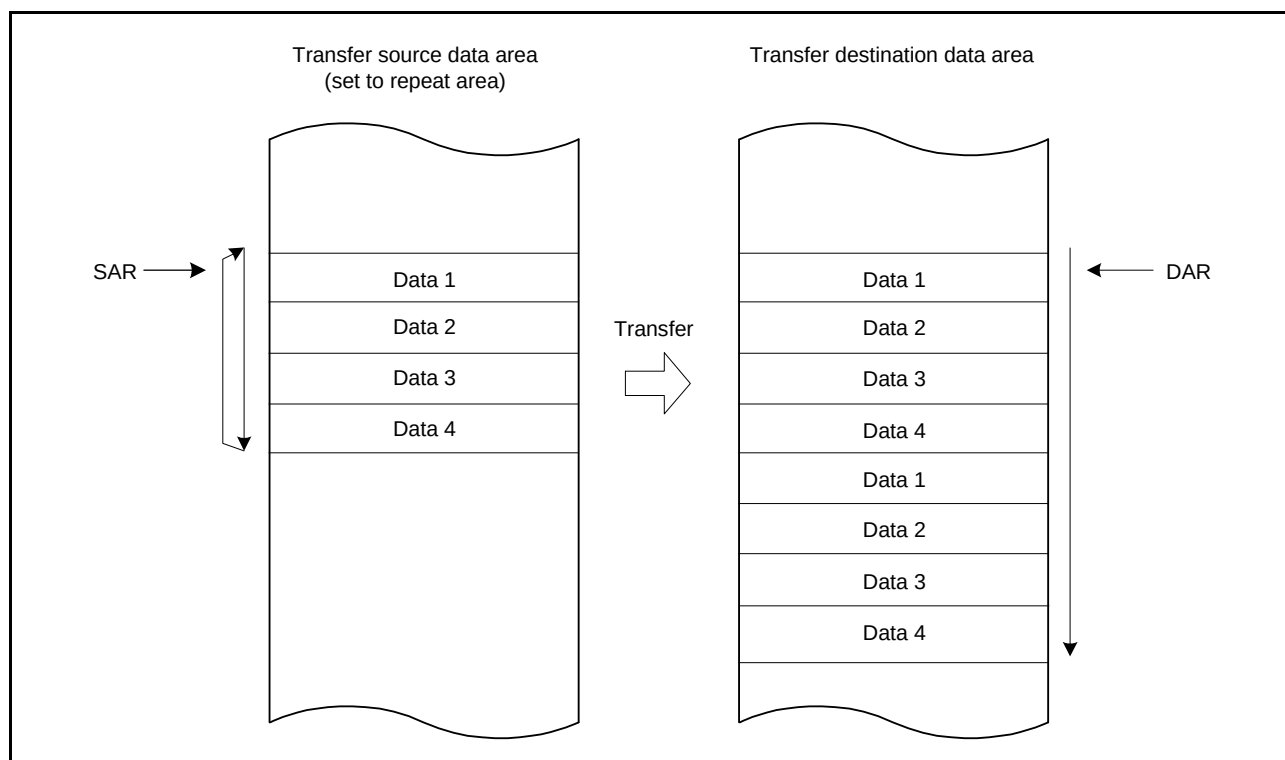
Figure 16.7 Memory Map of Repeat Transfer Mode (Transfer Source: Repeat Area)
