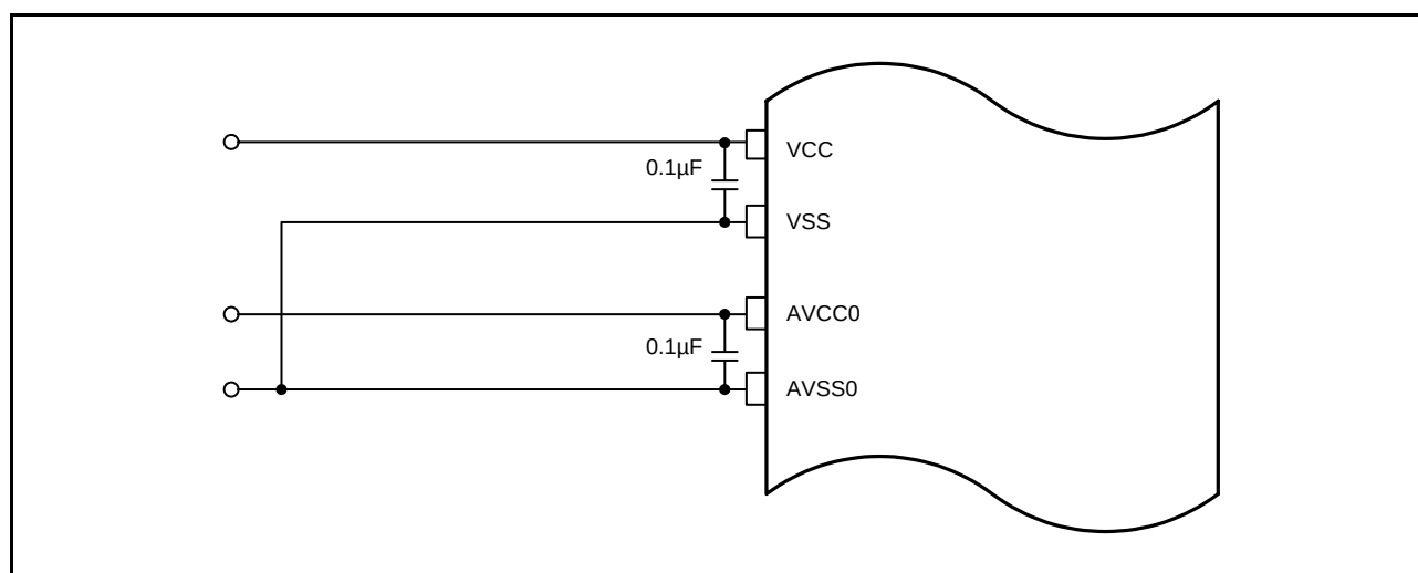
Figure 26.34 Power Supply Pin Connection Example
