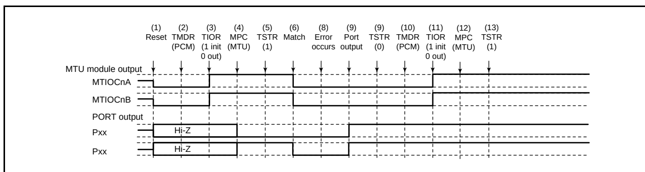
Figure 19.162 Error Occurrence in Phase Counting Mode, Recovery in Phase Counting Mode
