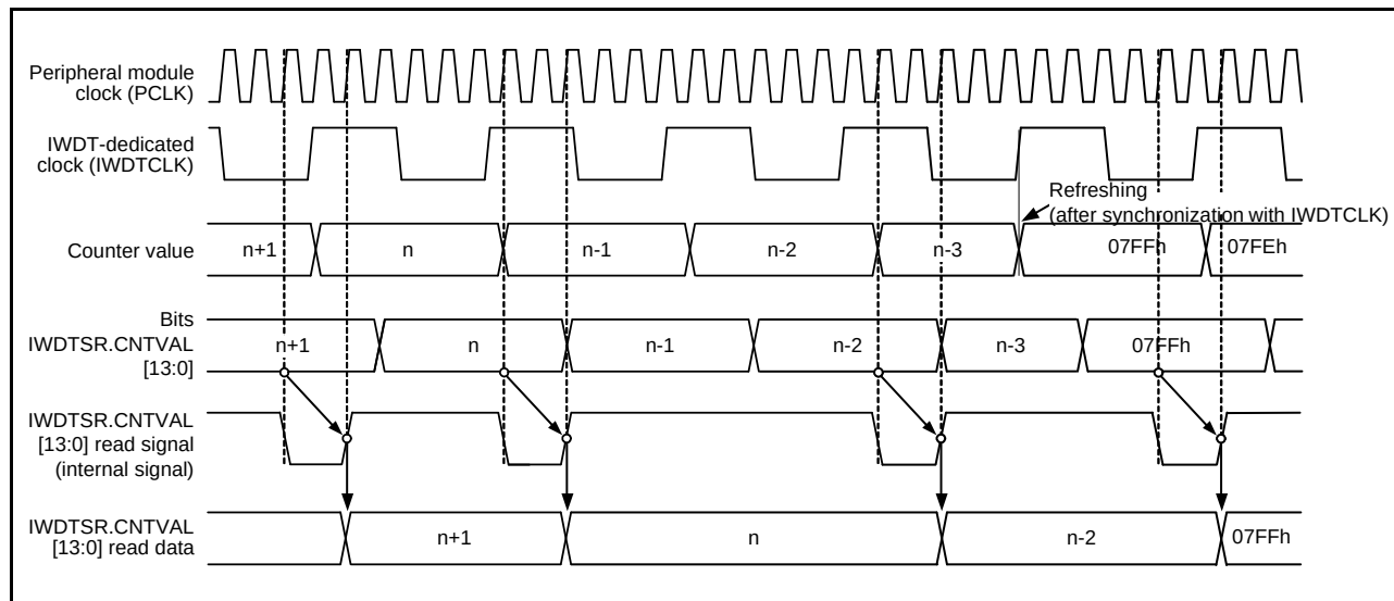
Figure 22.7 Processing for Reading IWDTC Counter Value (IWDTCR.CKS[3:0] = 0000b, IWDTCR.TOPS[1:0] = 11b)
