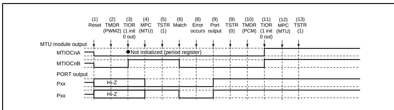
Figure 19.158 Error Occurrence in PWM Mode 2, Recovery in Phase Counting Mode
