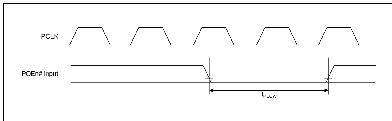
Figure 32.21 POE# Input Timing (n = 0, 8, 10)
