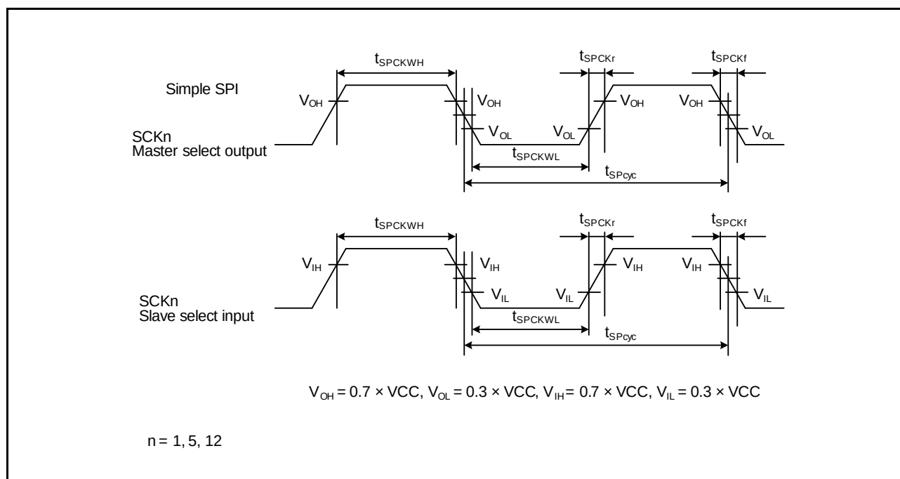
Figure 32.30 Simple SPI Clock Timing
