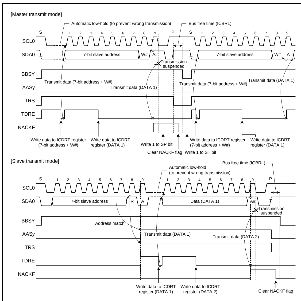
Figure 24.31 Suspension of Data Transmission When NACK is Received (NACKF = 1)
