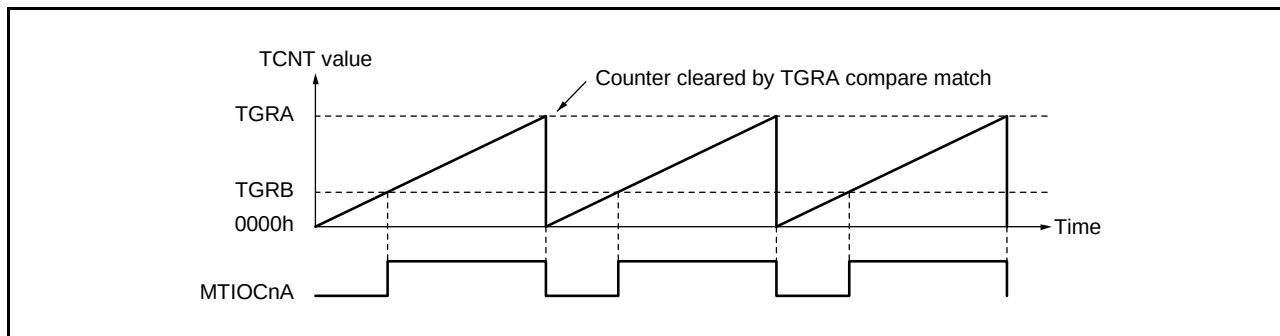
Figure 19.26 Example of PWM Mode 1 Operation (n = 0 to 4)
