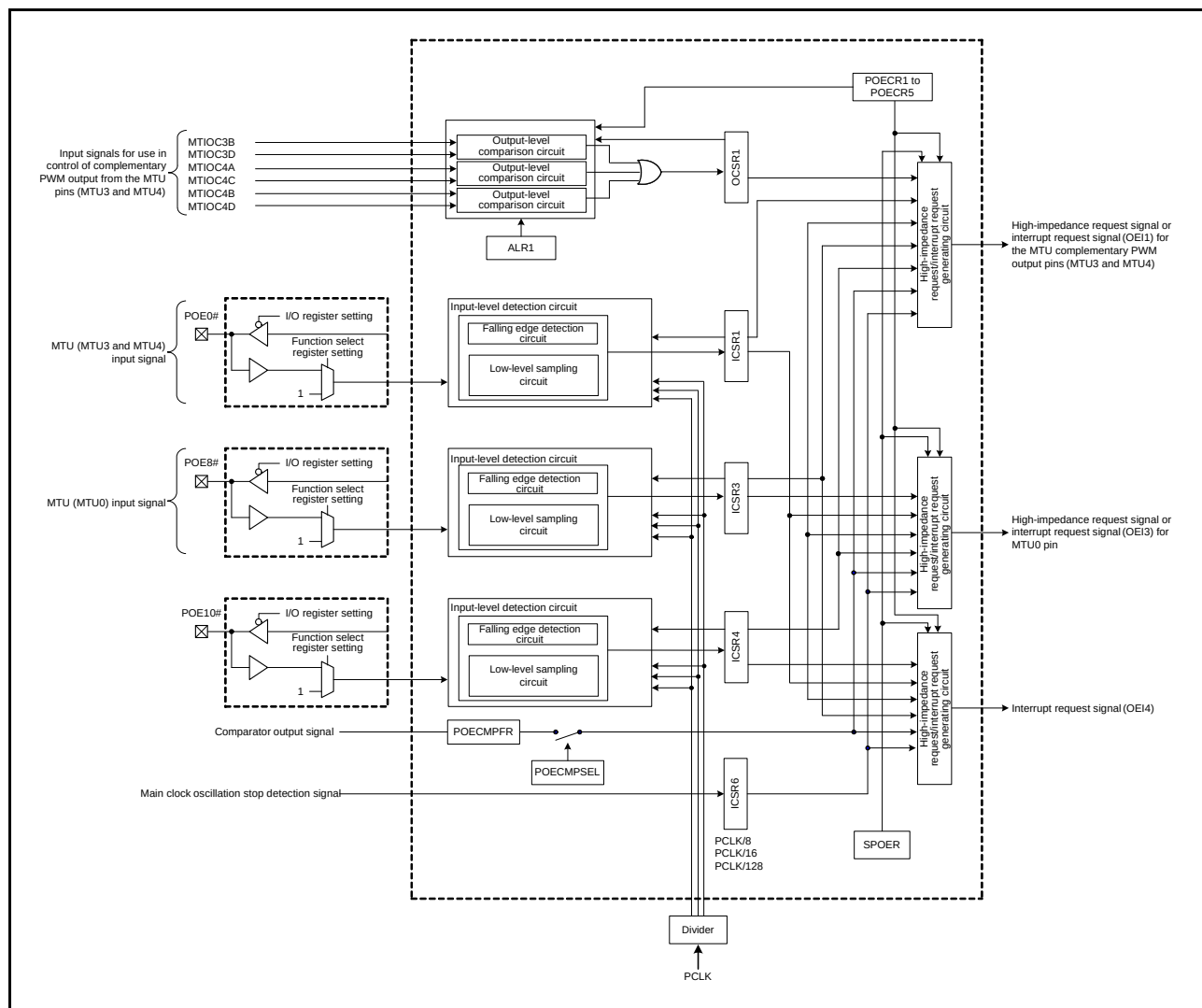
Figure 20.1 POE Block Diagram
