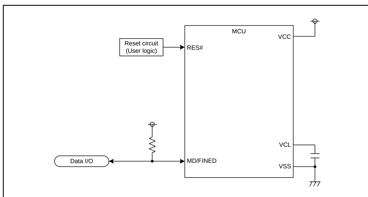
Figure 31.23 Example of Pin Connections in Boot Mode (FINE Interface)
