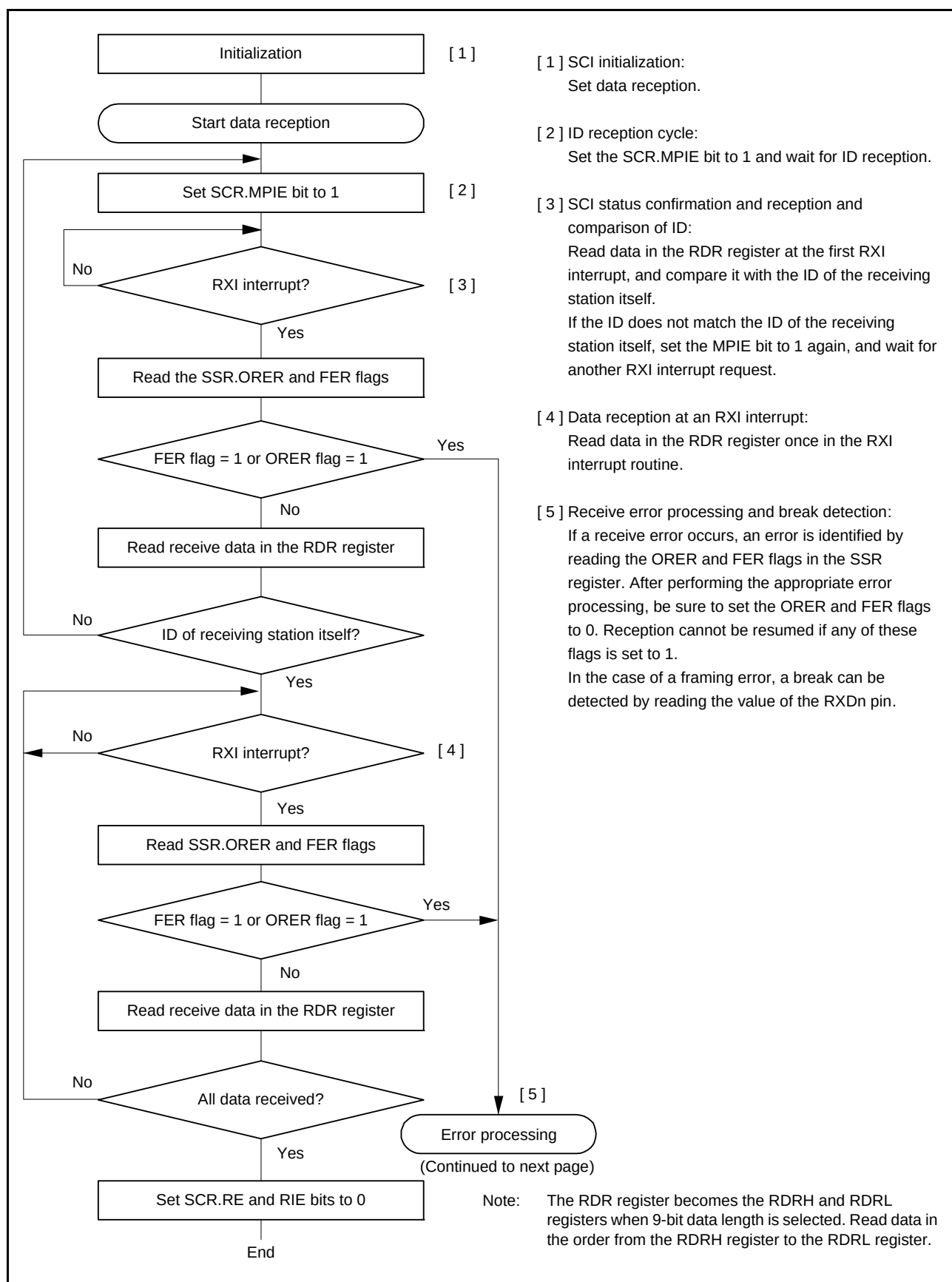
Figure 23.20 Example of Multi-Processor Serial Reception Flowchart (1)
