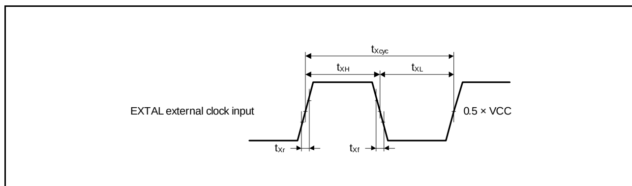
Figure 32.4 EXTAL External Clock Input Timing
