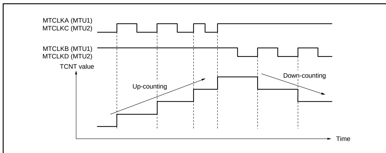
Figure 19.35 Example of Operation in Phase Counting Mode 3 (When MTUn.TCR2.PCB[1:0] = 01b (n = 1, 2))
