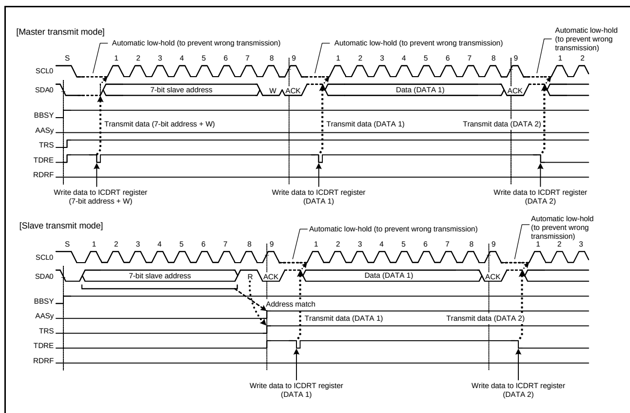
Figure 24.30 Automatic Low-Hold Operation in Transmit Mode
