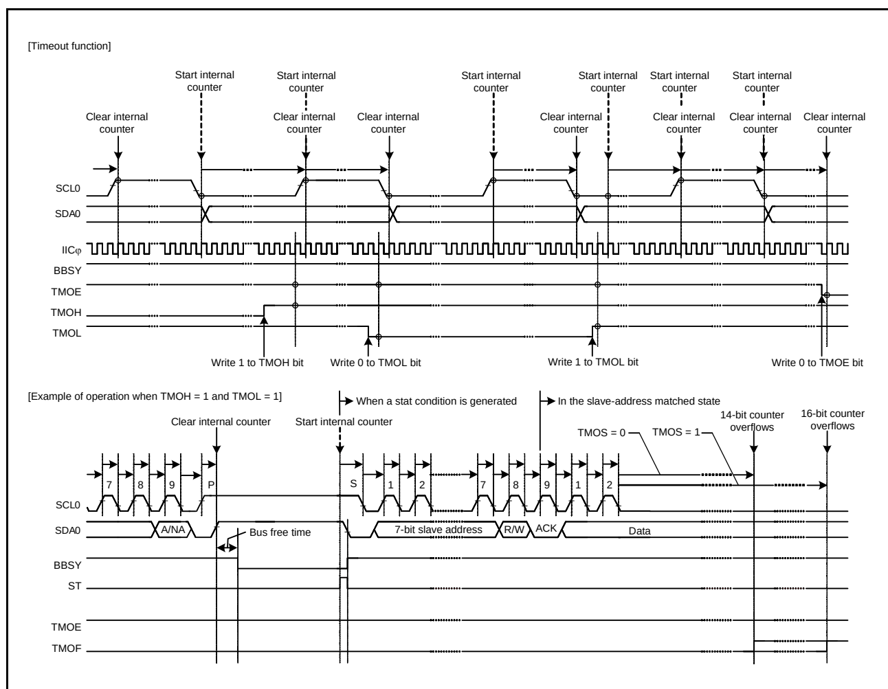
Figure 24.39 Timeout Function
