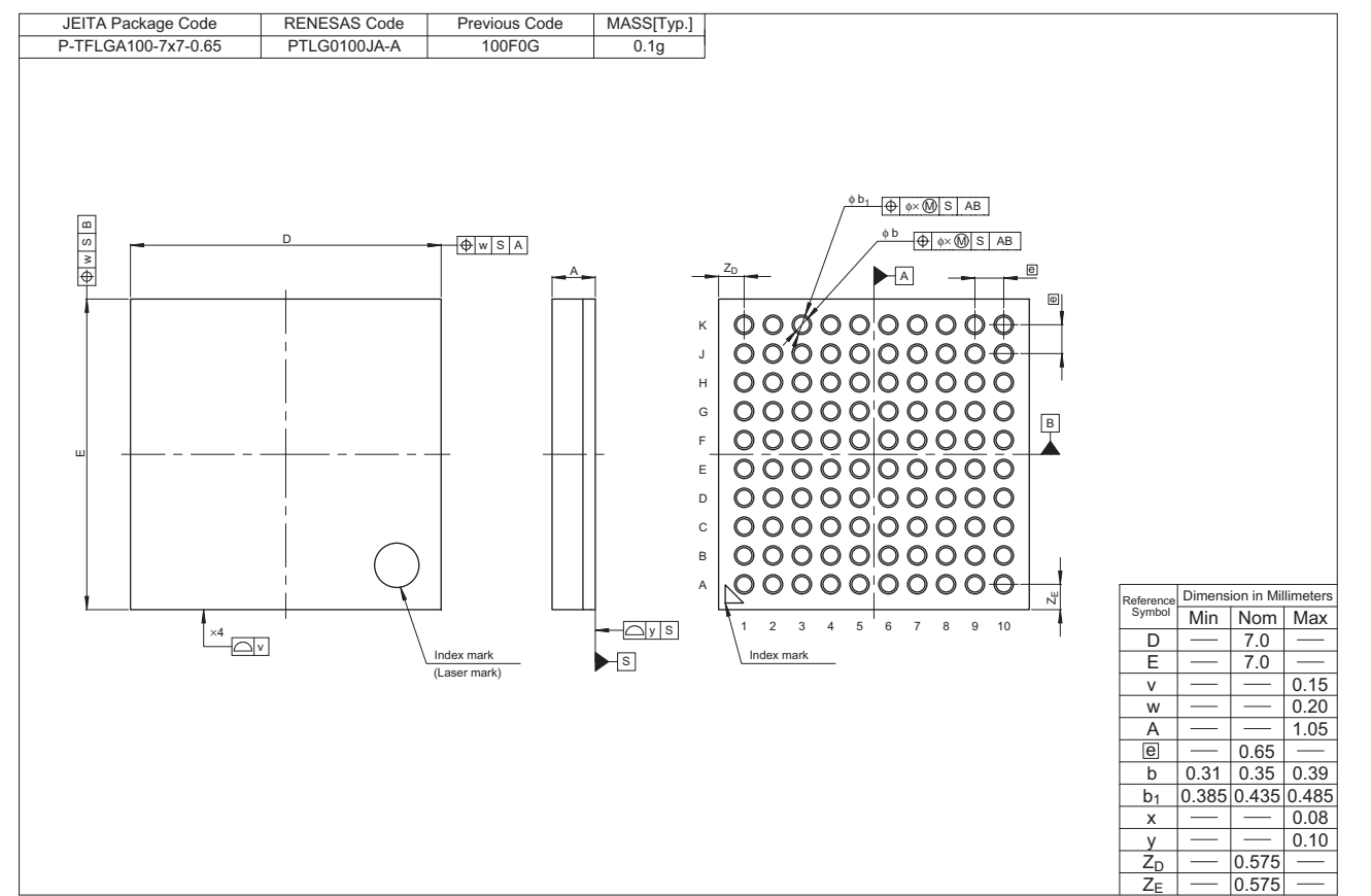
Figure F 100-Pin TFLGA (PTLG0100JA-A)
