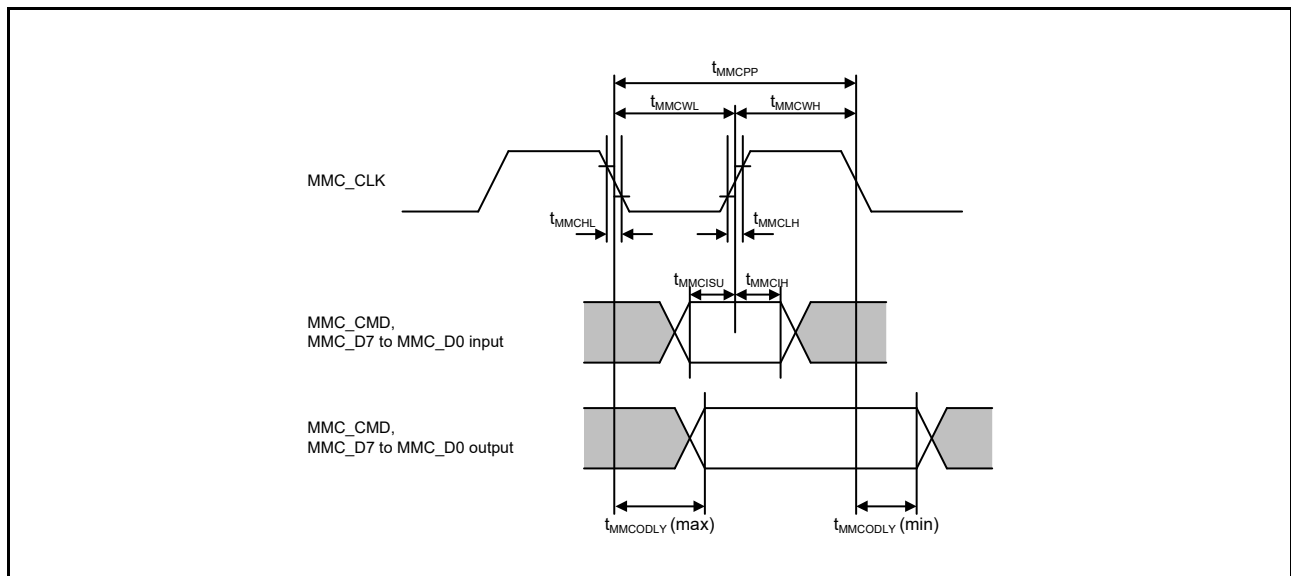
Figure 5.55 MMC Interface
