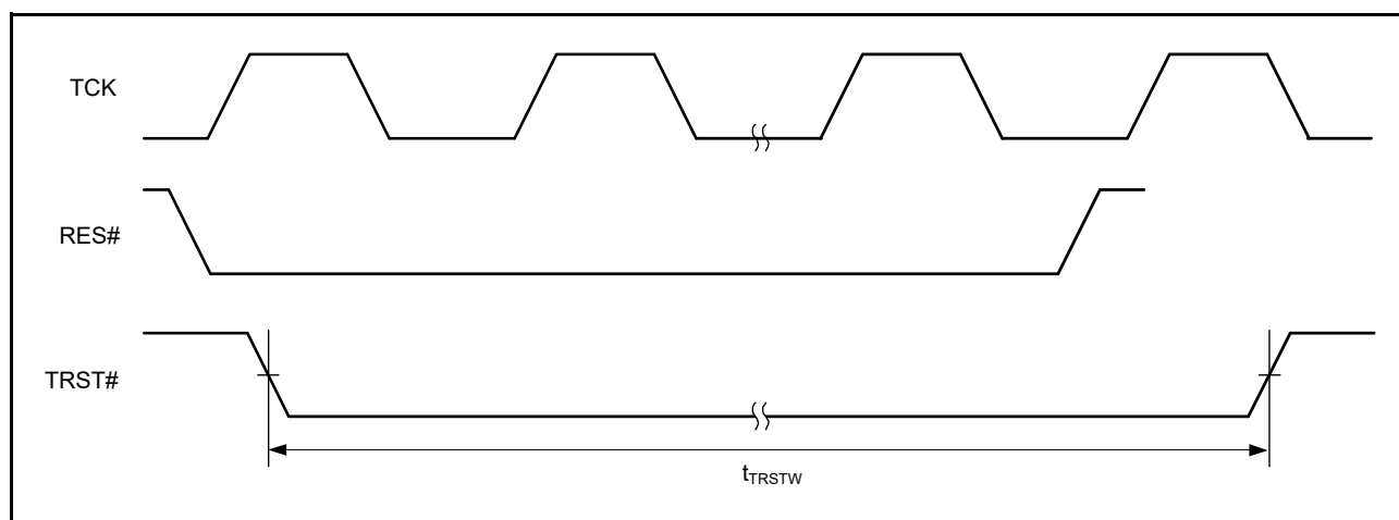
Figure 5.88 Boundary Scan TRST# Timing
