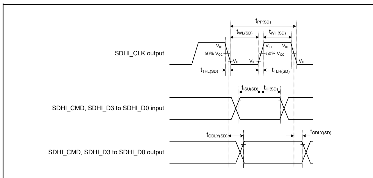
Figure 5.72 SD Host Interface Input/Output Signal Timing
