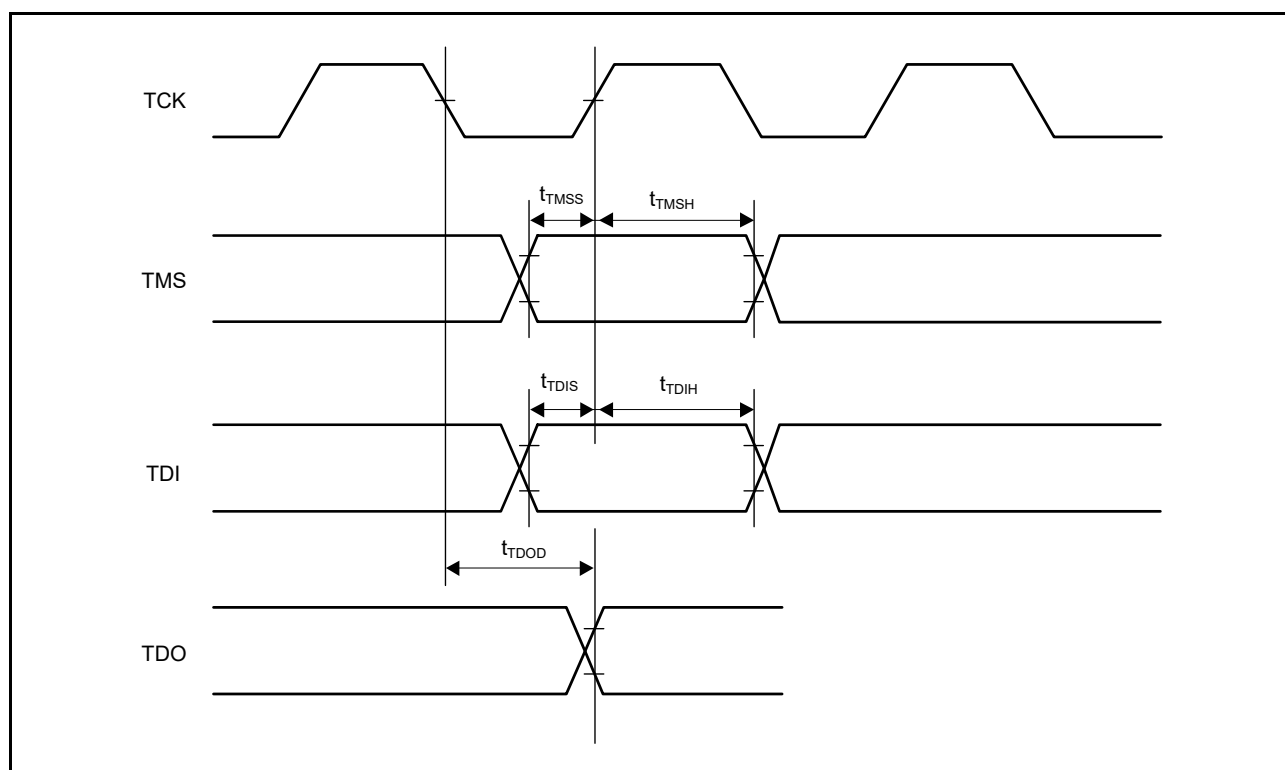
Figure 5.89 Boundary Scan Input/Output Timing
