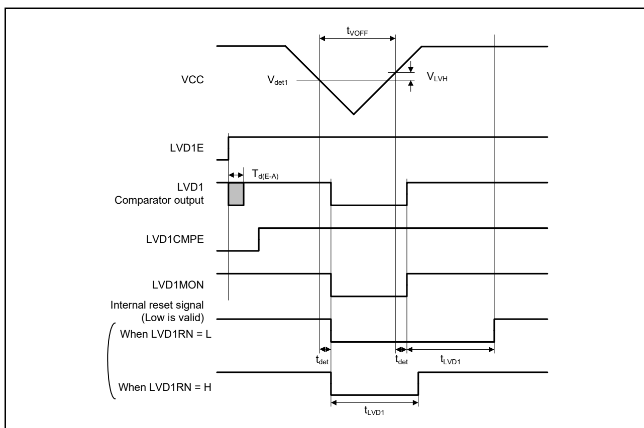
Figure 5.82 Voltage Detection Circuit Timing ( V_{det1} )
