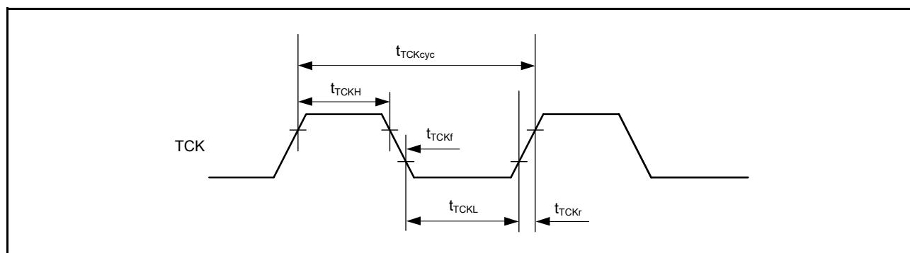
Figure 5.87 Boundary Scan TCK Timing
