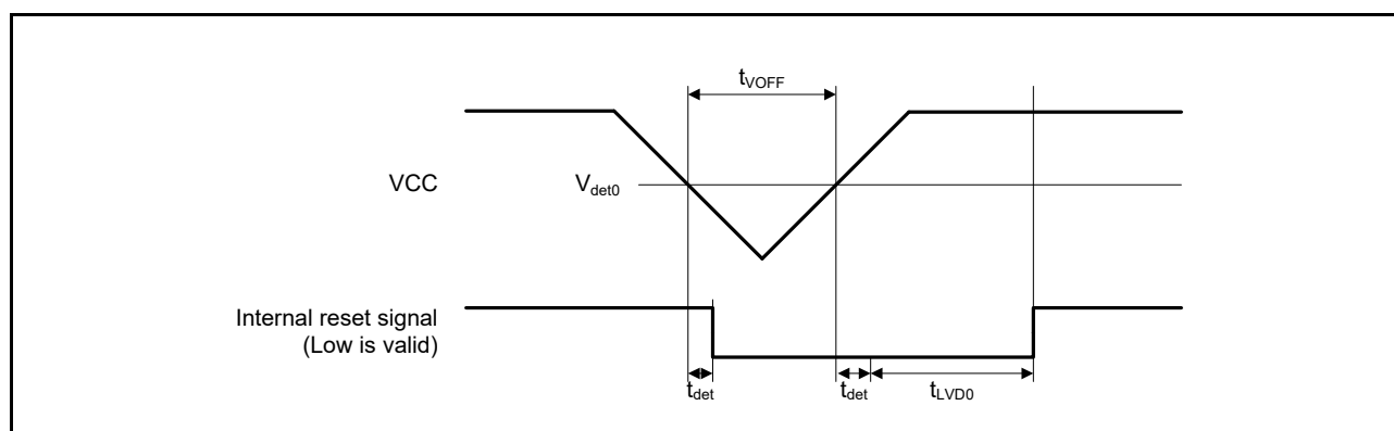
Figure 5.81 Voltage Detection Circuit Timing ( V_{det0} )
