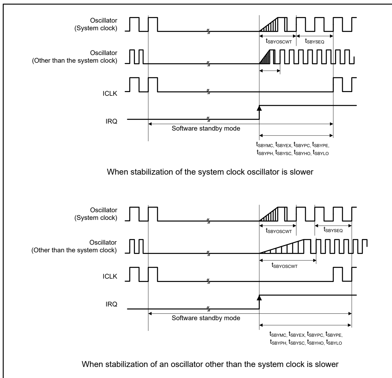
Figure 5.12 Software Standby Mode Recovery Timing
