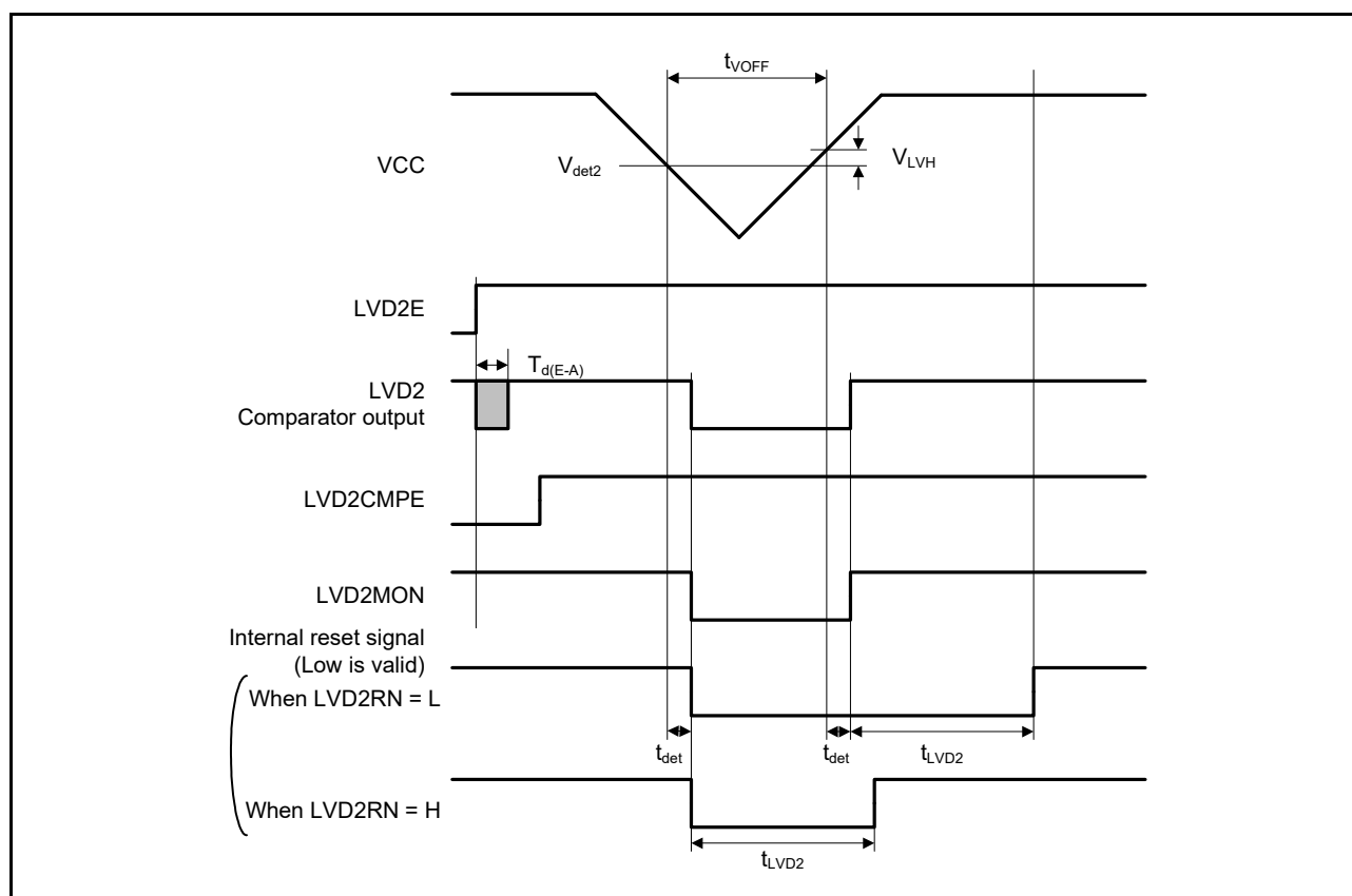
Figure 5.83 Voltage Detection Circuit Timing ( V_{det2} )
