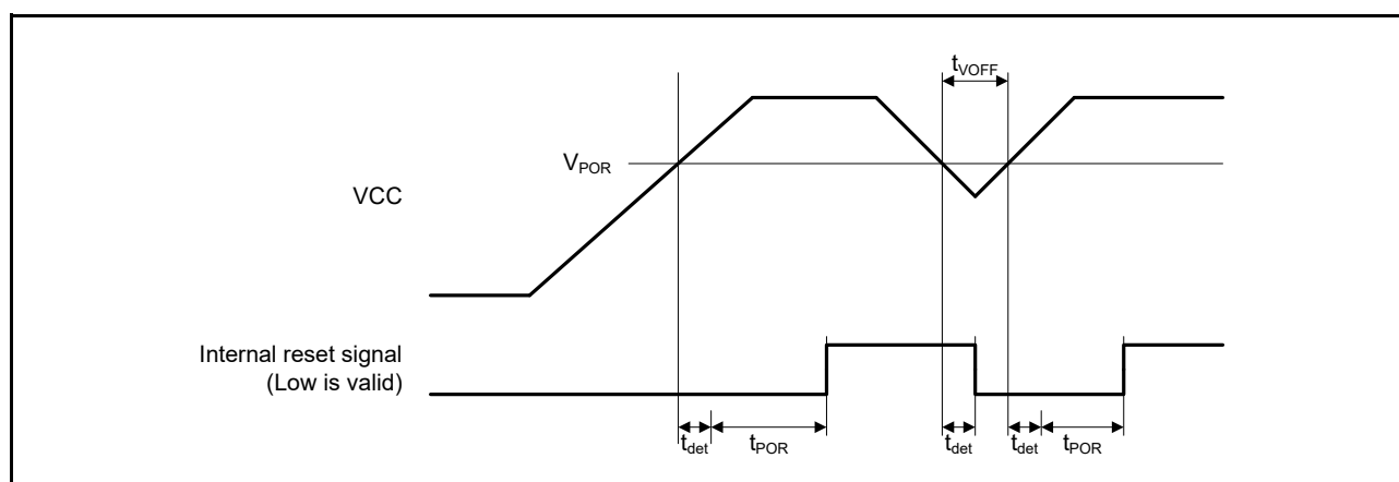
Figure 5.80 Power-on Reset Timing
