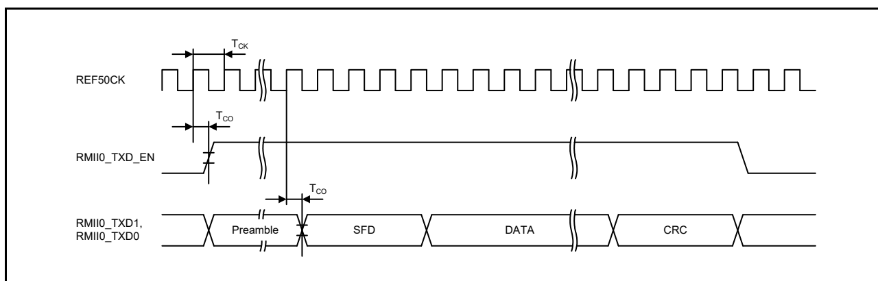
Figure 5.57 RMII Transmission Timing
