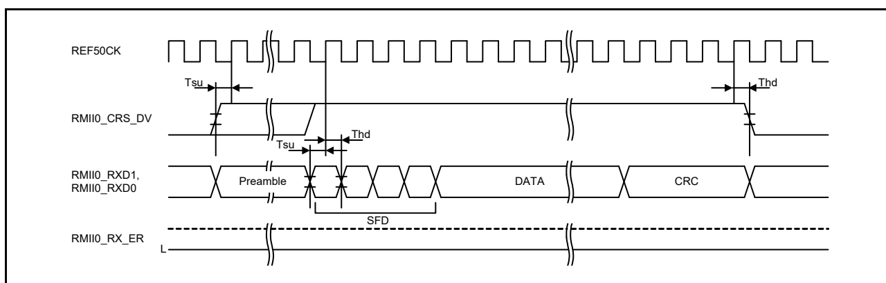
Figure 5.58 RMII Reception Timing (Normal Operation)
