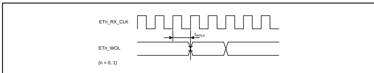
Figure 2.90 WOL Output Timing (MII)
