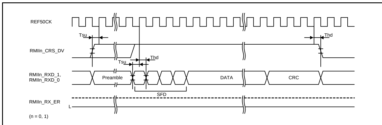
Figure 2.83 RMI Reception Timing (Normal Operation)
