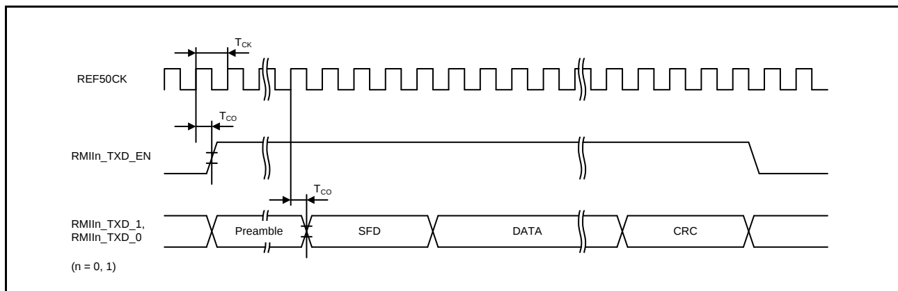
Figure 2.82 RMI Transmission Timing
