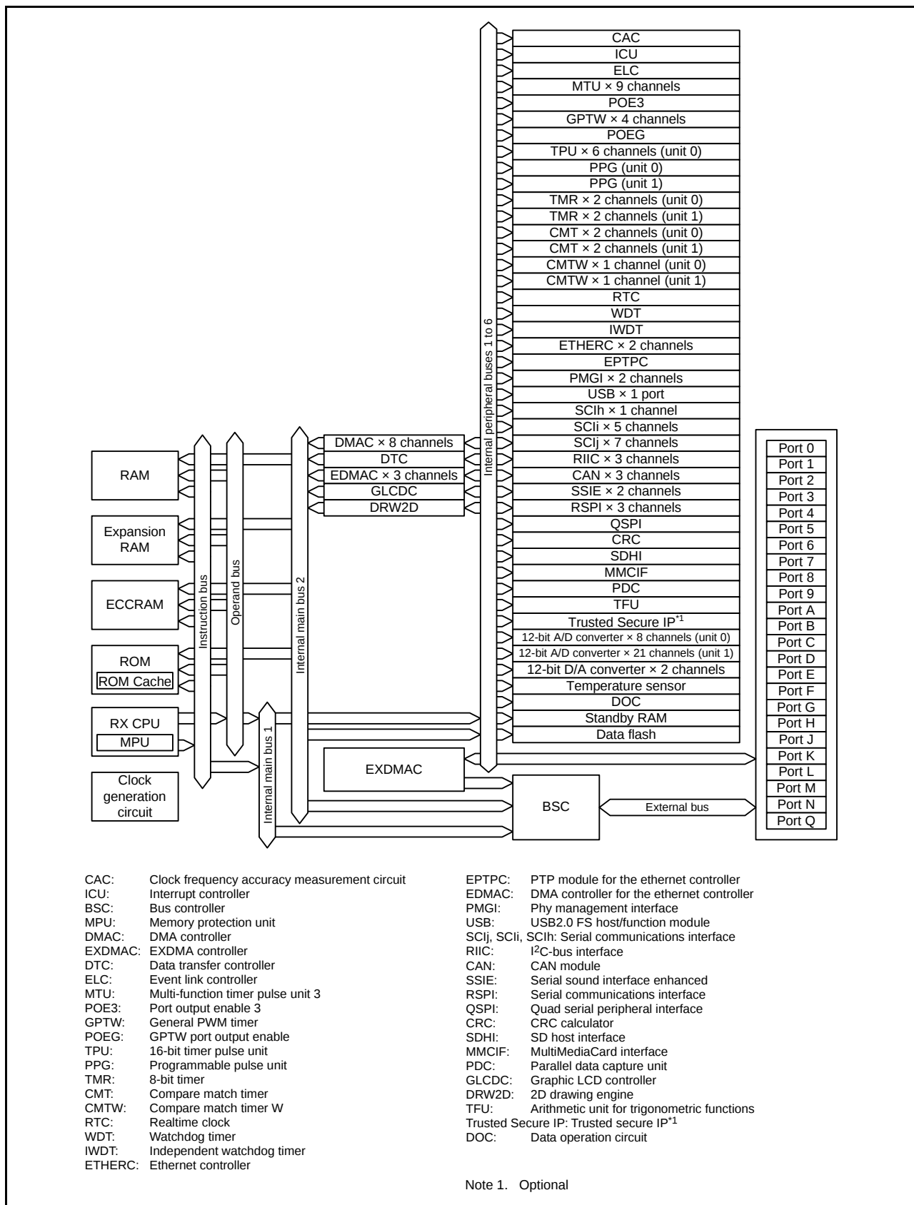
Figure 1.2 Block Diagram
