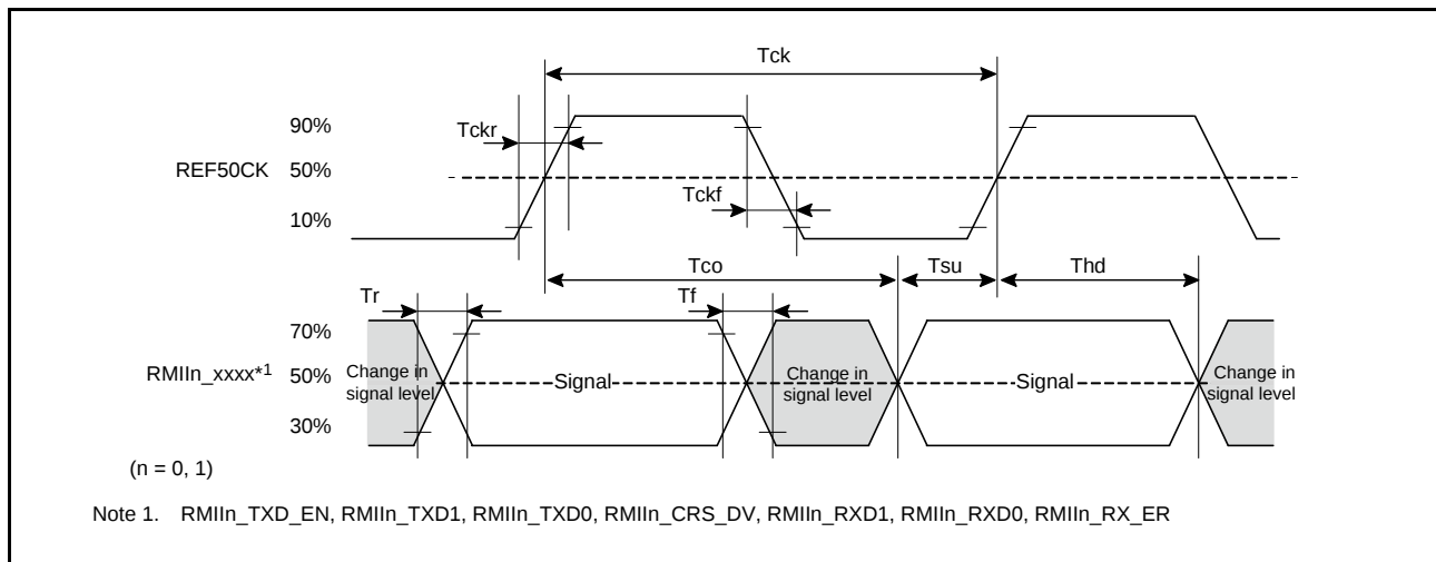
Figure 2.81 Timing with the REF50CK and RMI Signals
