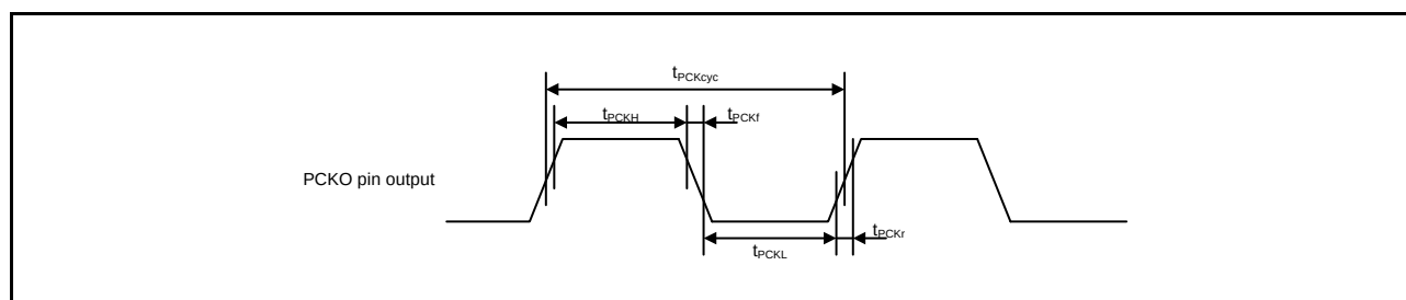
Figure 2.92 PDC Output Clock Timing
