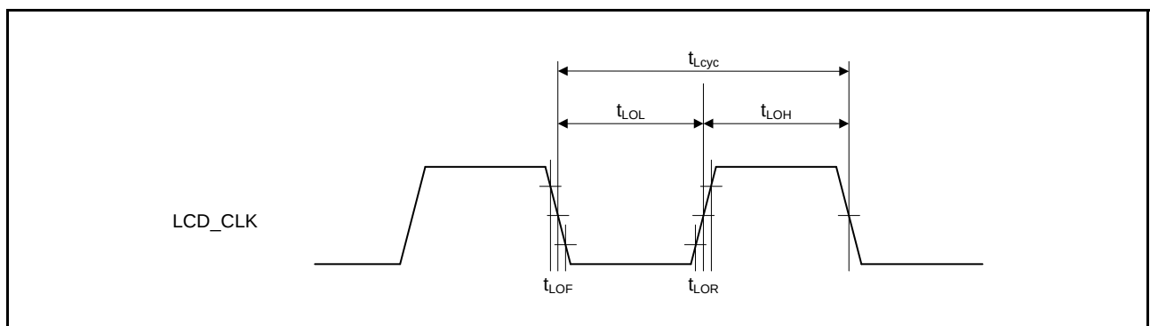
Figure 2.95 LCD_CLK Clock Output Timing
