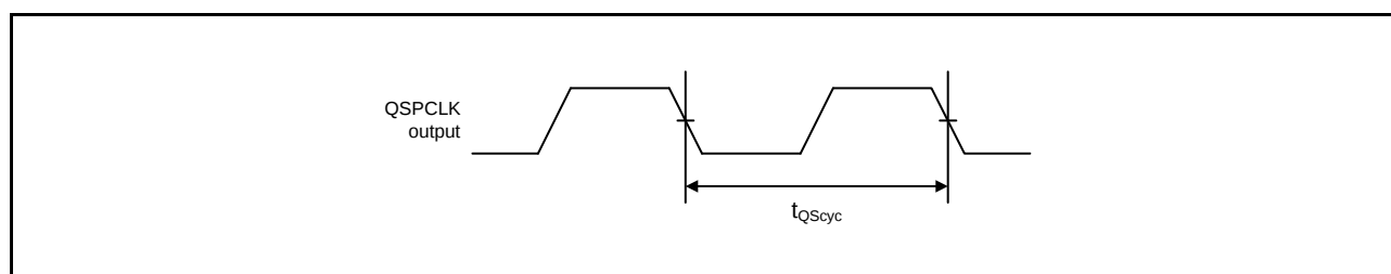
Figure 2.70 QSPI Clock Timing
