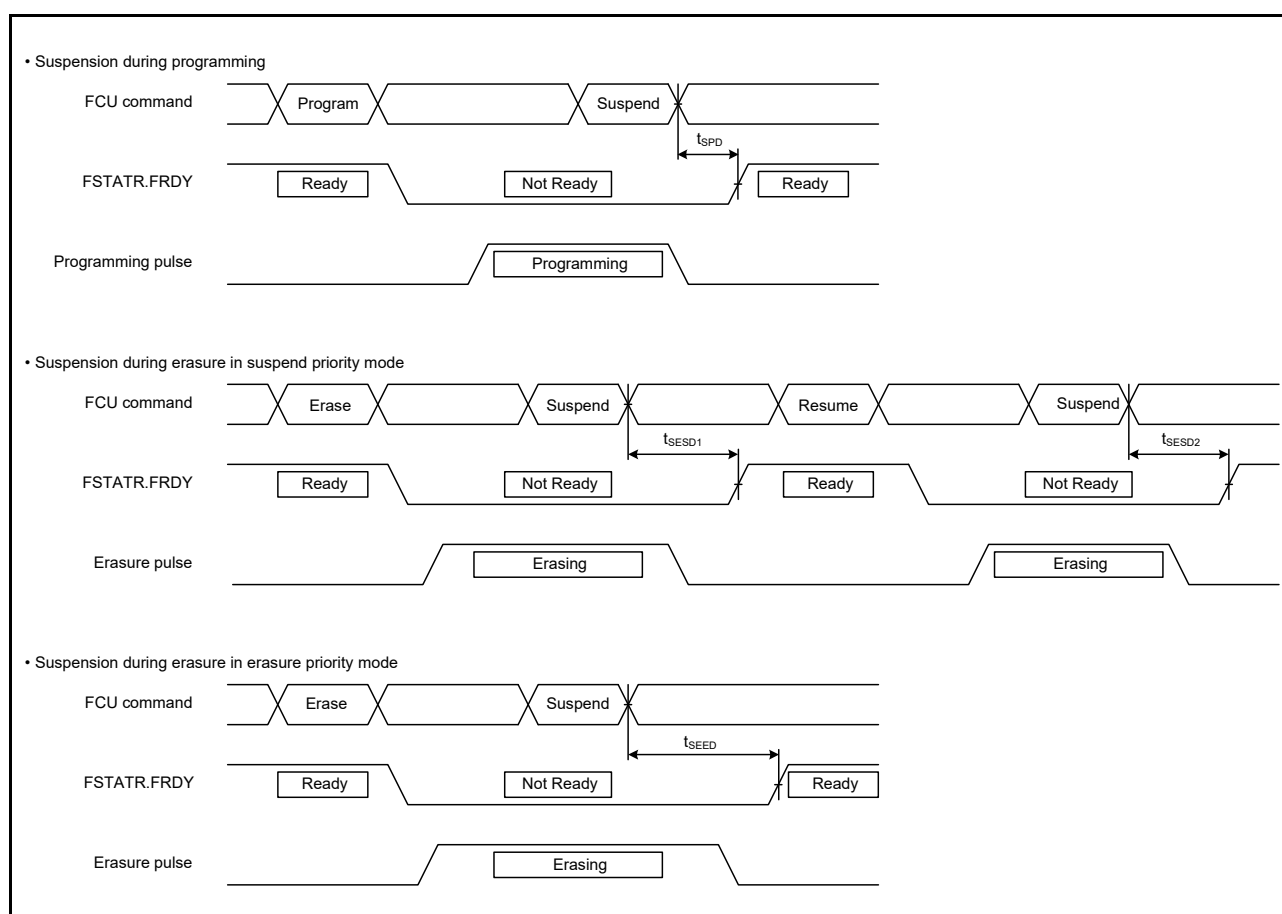
Figure 5.86 Flash Memory Programming/Erase Suspension Timing
