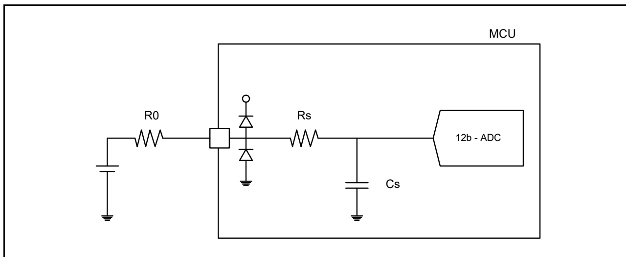
Figure 5.57 Equivalent Circuit
