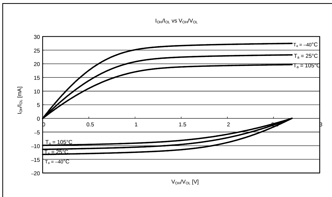
Figure 5.9 V_{OH}/V_{OL} and I_{OH}/I_{OL} Temperature Characteristics of General Ports (Except for the RIIC Output Pin, Ports P40 to P44, P46, Ports PJ6, PJ7) at V_{CC} = 2.7 V (Reference Data)
