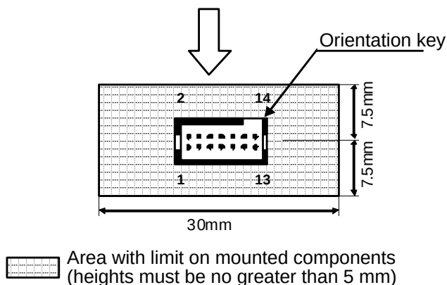
Figure 3 Limit on Height of Components Mounted around the Connector on the User System (the Connector for the Adapter)
