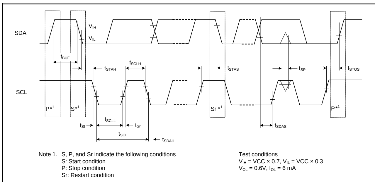
Figure 6.25 RIIC Bus Interface Input/Output Timing and Simple IIC Bus Interface Input/Output Timing
