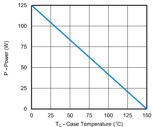
Power, Junction-to-Case
