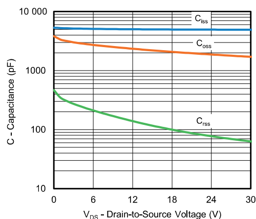
Capacitance
