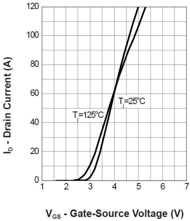
Transfer Characteristics
