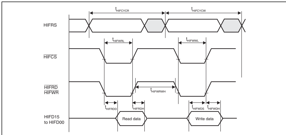
Figure 29.55 HIF Access Timing
