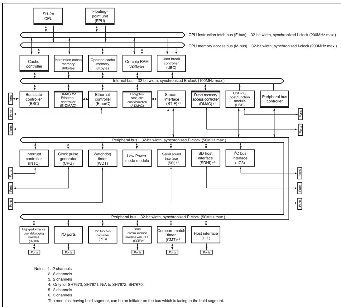
Figure 1.2 Block Diagram
