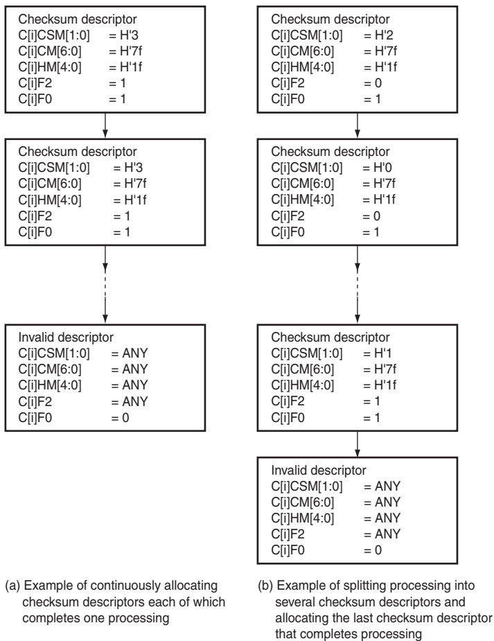
Figure 14.3 Examples of Allocating Checksum Descriptors
