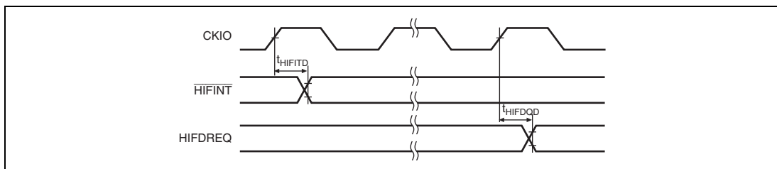
Figure 29.56 HIFINT/HIFDREQ Timing
