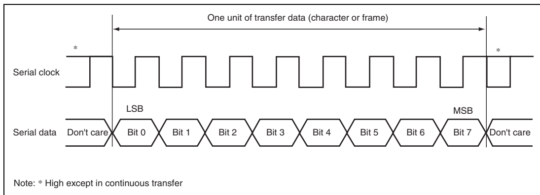
Figure 22.11 Data Format in Clocked Synchronous Communication
