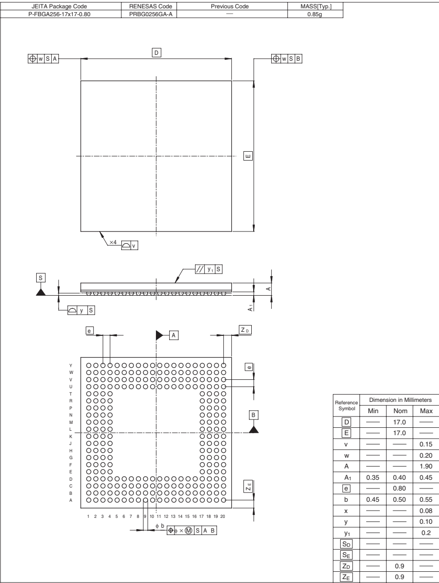
Figure C.1 Package Dimensions
