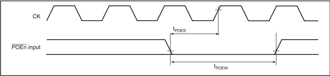
Figure 33.43 POE2 Input/Output Timing
