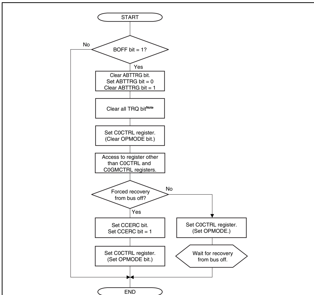
Figure 20-55. Bus-off Recovery (Normal Operation Mode with ABT)
