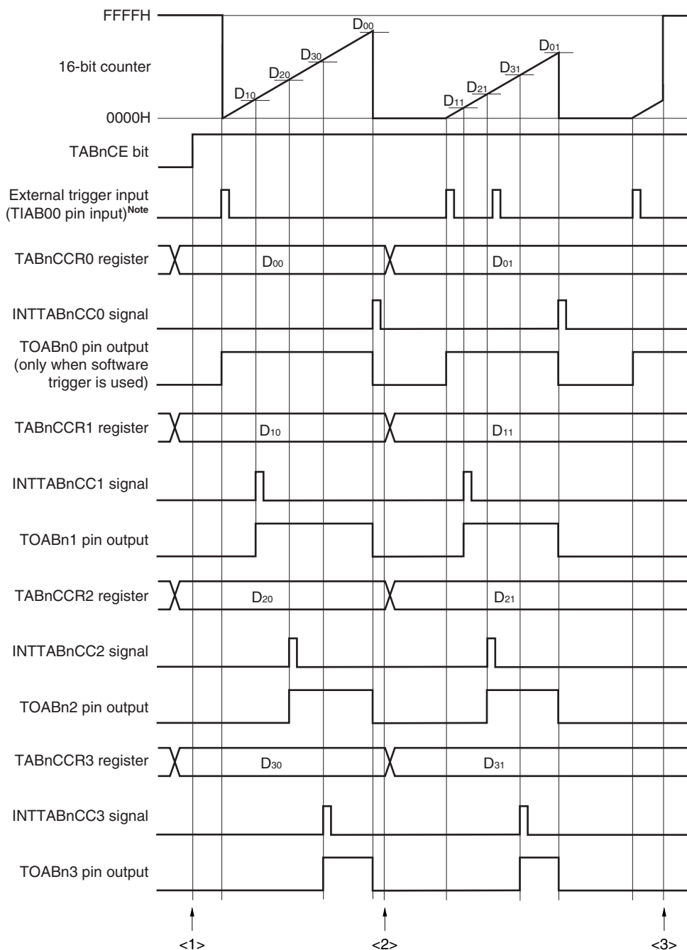
Figure 8-23. Software Processing Flow in One-Shot Pulse Output Mode (1/2)
