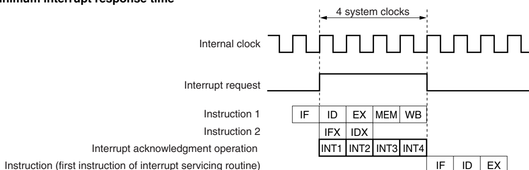
Figure 23-15. Pipeline Operation at Interrupt Request Signal Acknowledgment (Outline)
