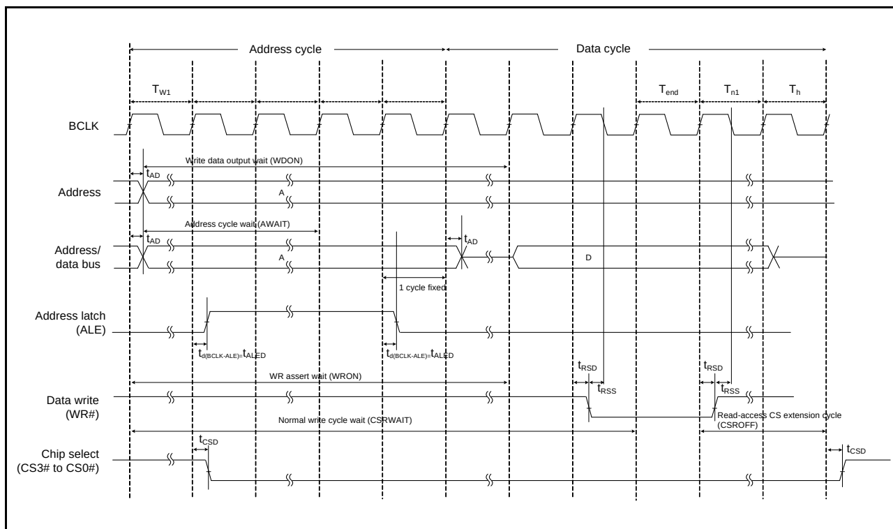
Figure 5.82 Example of Operation in Write Access over the External Bus (Multiplexed)
