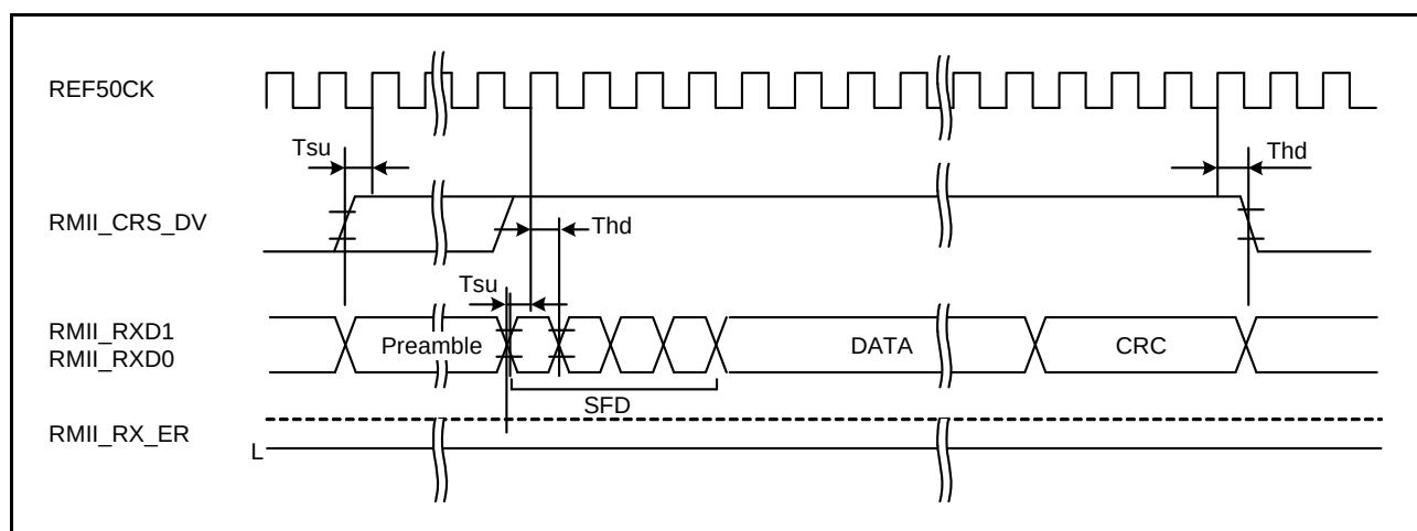
Figure 5.50 RMII Reception Timing (Normal Operation)
