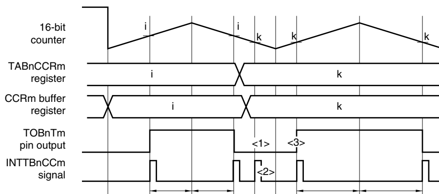
Figure 10-25. Example of Rewriting TABnCCR1 to TABnCCR3 Registers (Rewriting After Match Occurs)
