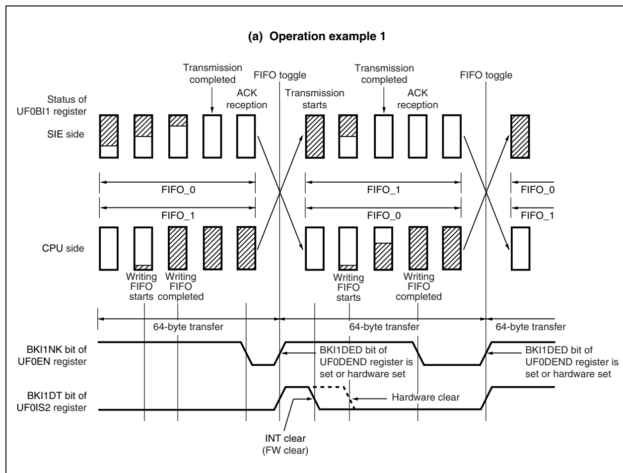
Figure 18-9. Operation of UF0BI1 Register (1/3)
