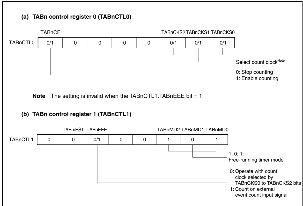
Figure 7-36. Register Setting in Free-Running Timer Mode (1/3)
