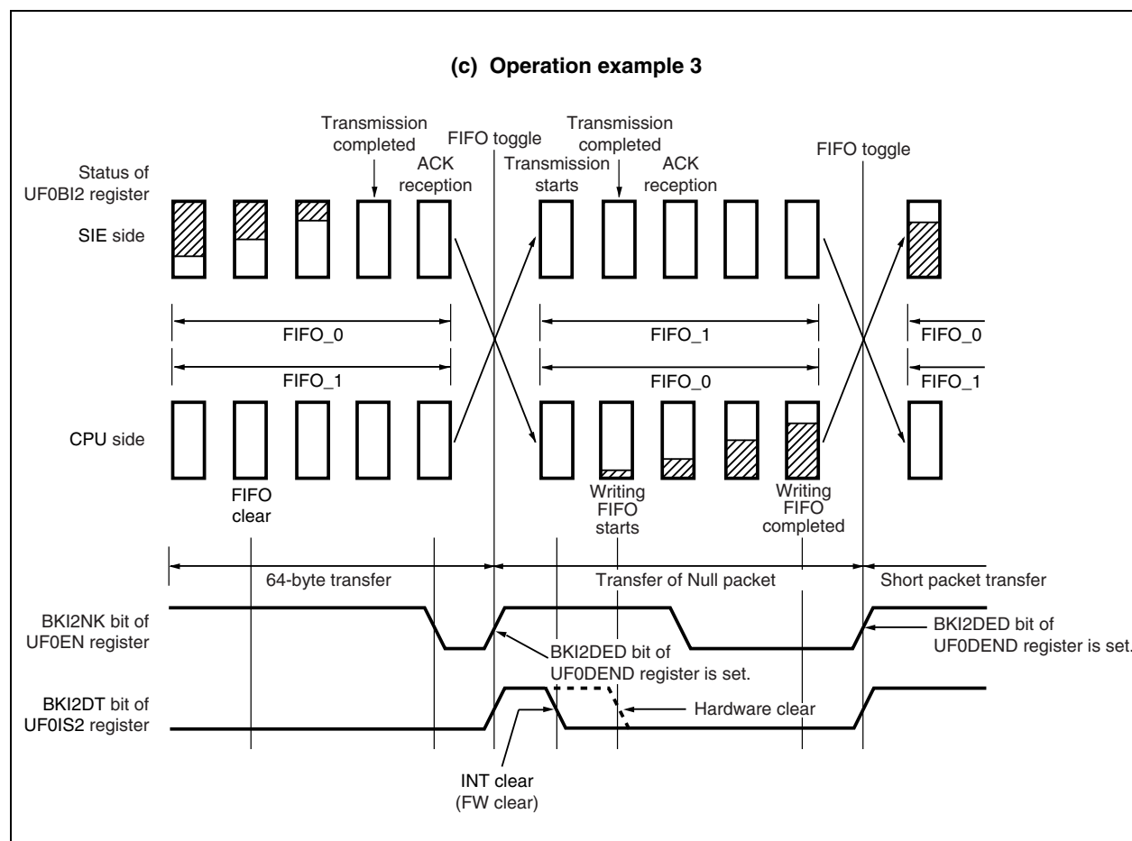
Figure 18-10. Operation of UF0BI2 Register (3/3)
