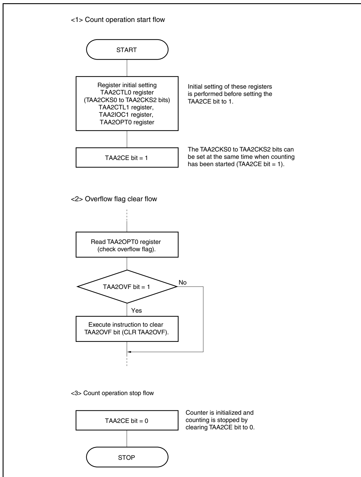
Figure 6-43. Software Processing Flow in Free-Running Timer Mode (Capture Function) (2/2)
