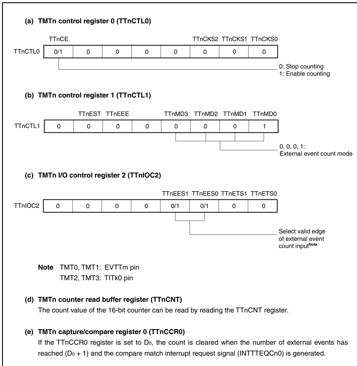
Figure 8-17. Register Setting for Operation in External Event Count Mode (1/2)
