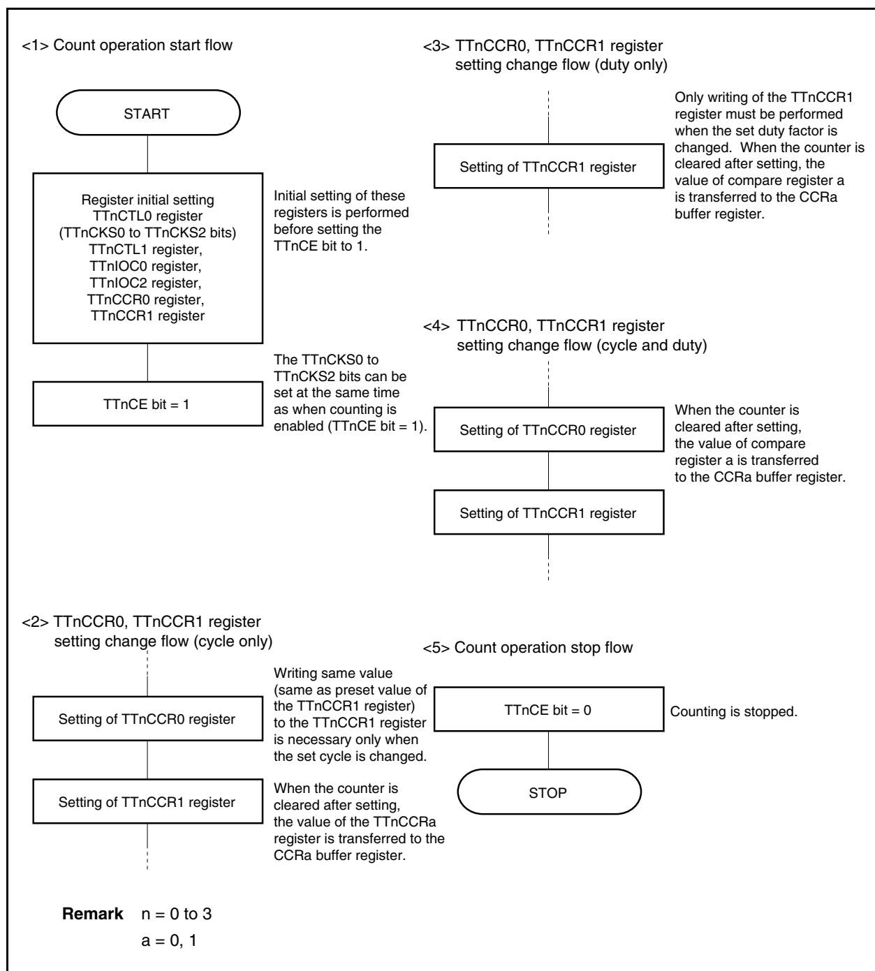
Figure 8-36. Software Processing Flow in PWM Output Mode (2/2)
