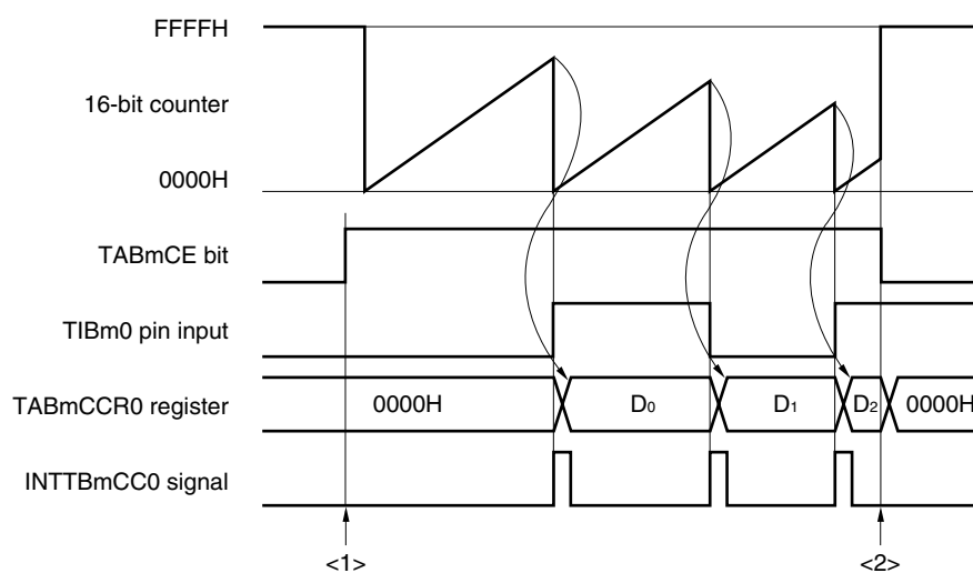
Figure 7-42. Software Processing Flow in Pulse Width Measurement Mode
