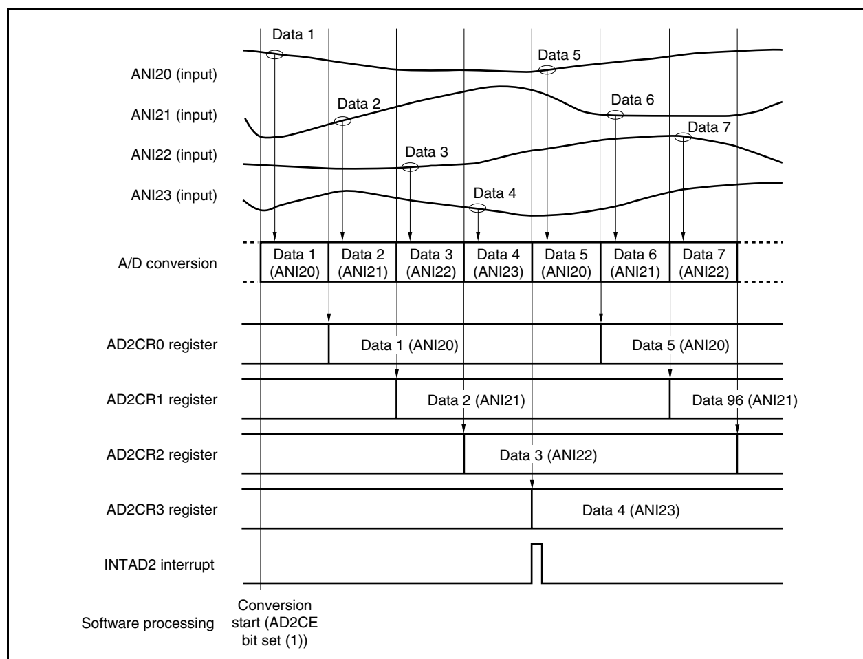
Figure 13-5. Continuous Scan Mode Operation Timing (When AD2M0.AD2MD1 and AD2M0.AD2MD0 Bits = 01, AD2S.AD2S3 to AD2S.AD2S0 Bits = 0011)
