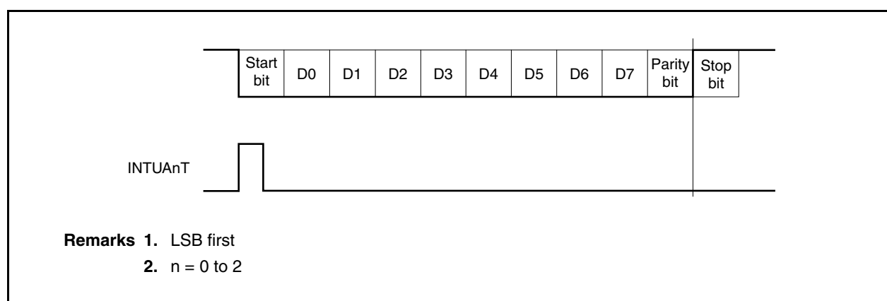
Figure 14-6. UART Transmission
