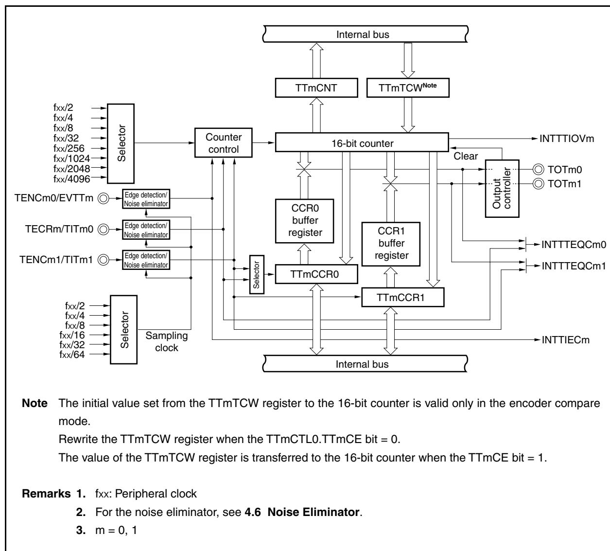
Figure 8-1. Block Diagram of TMT0 and TMT1
