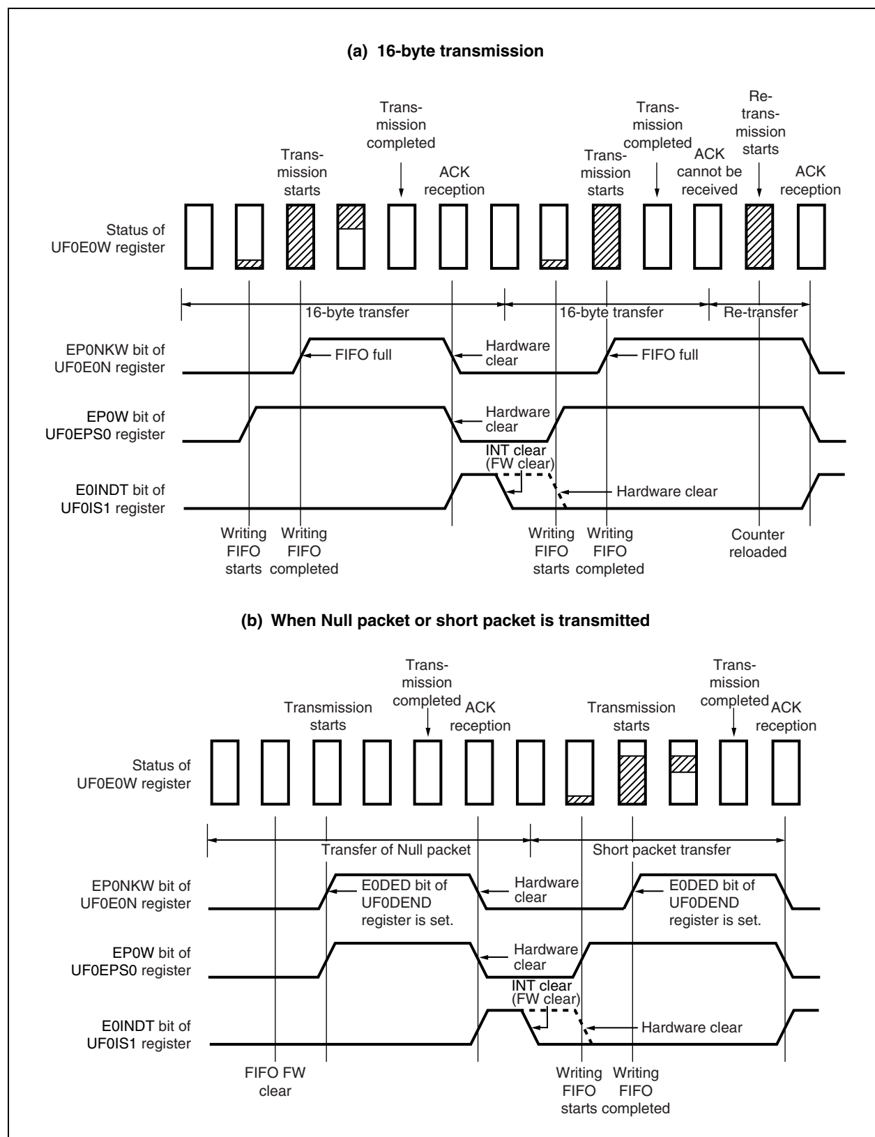
Figure 18-6. Operation of UF0E0W Register
