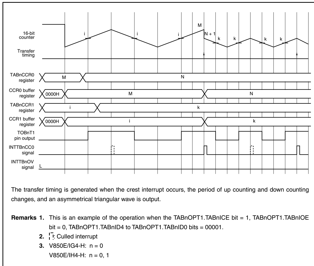
Figure 10-32. Rewriting TABnCCR0 Register (When Crest Interrupt Is Set)
