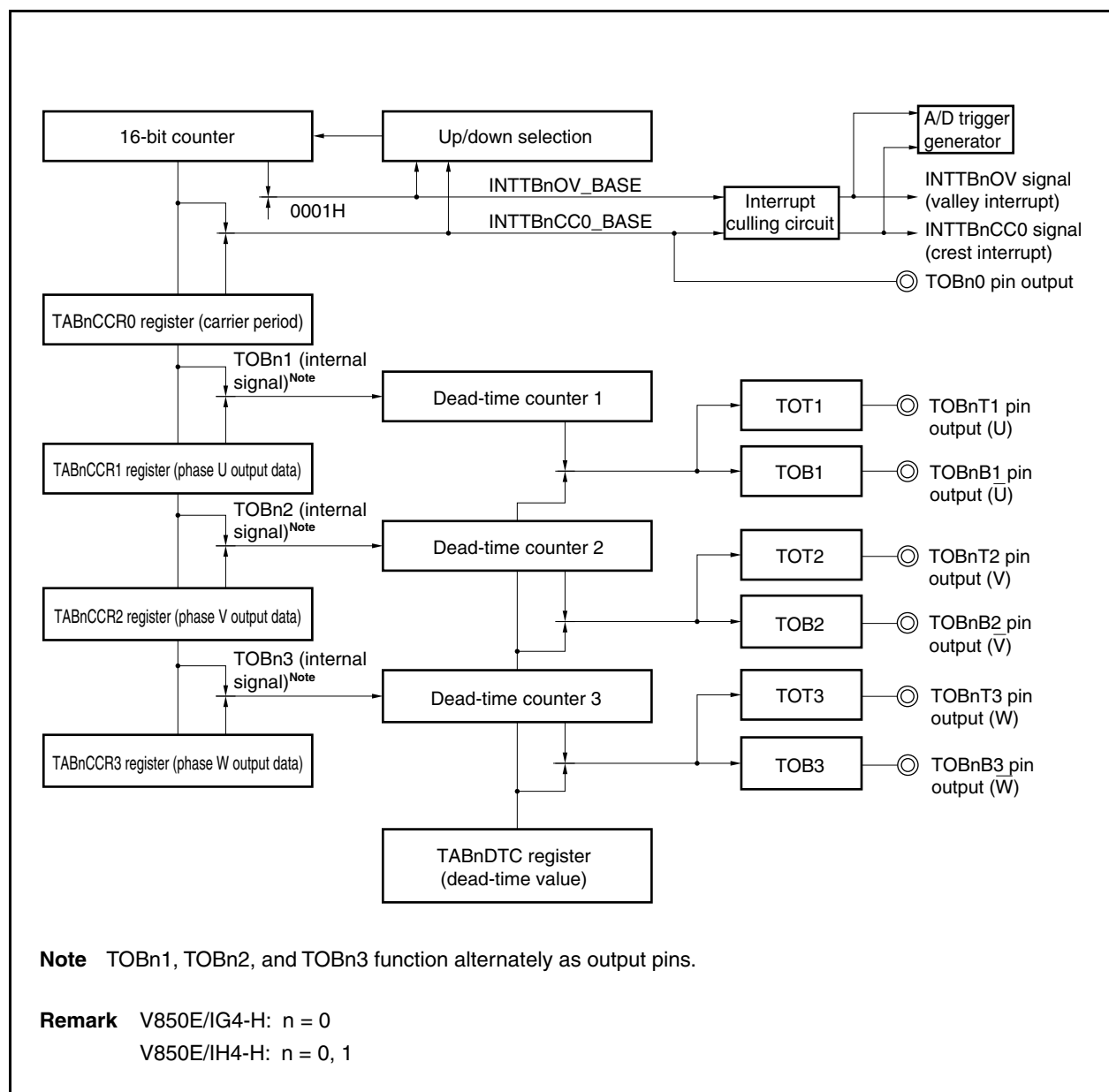
Figure 10-5. Outline of 6-Phase PWM Output Mode
