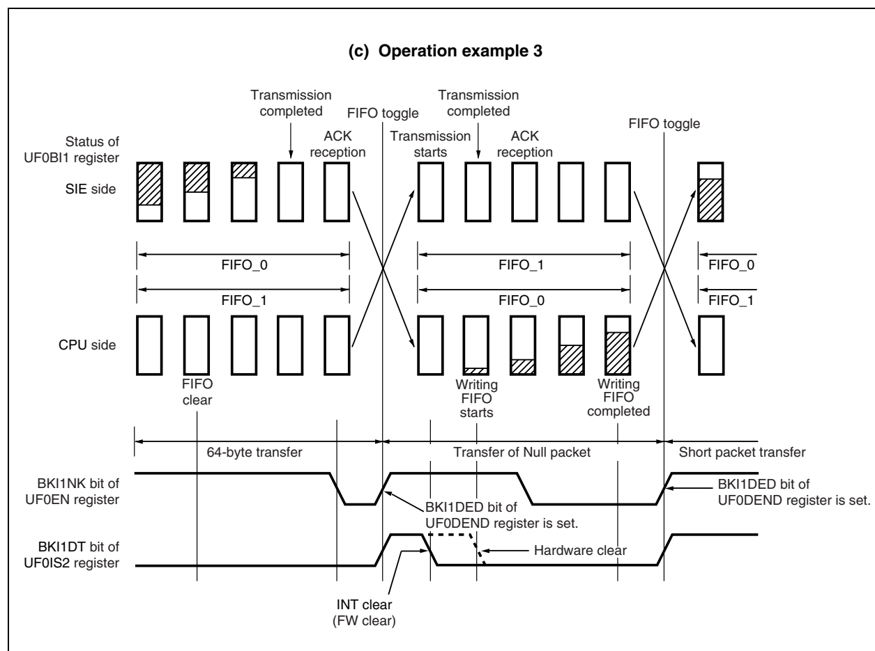
Figure 18-9. Operation of UF0BI1 Register (3/3)
