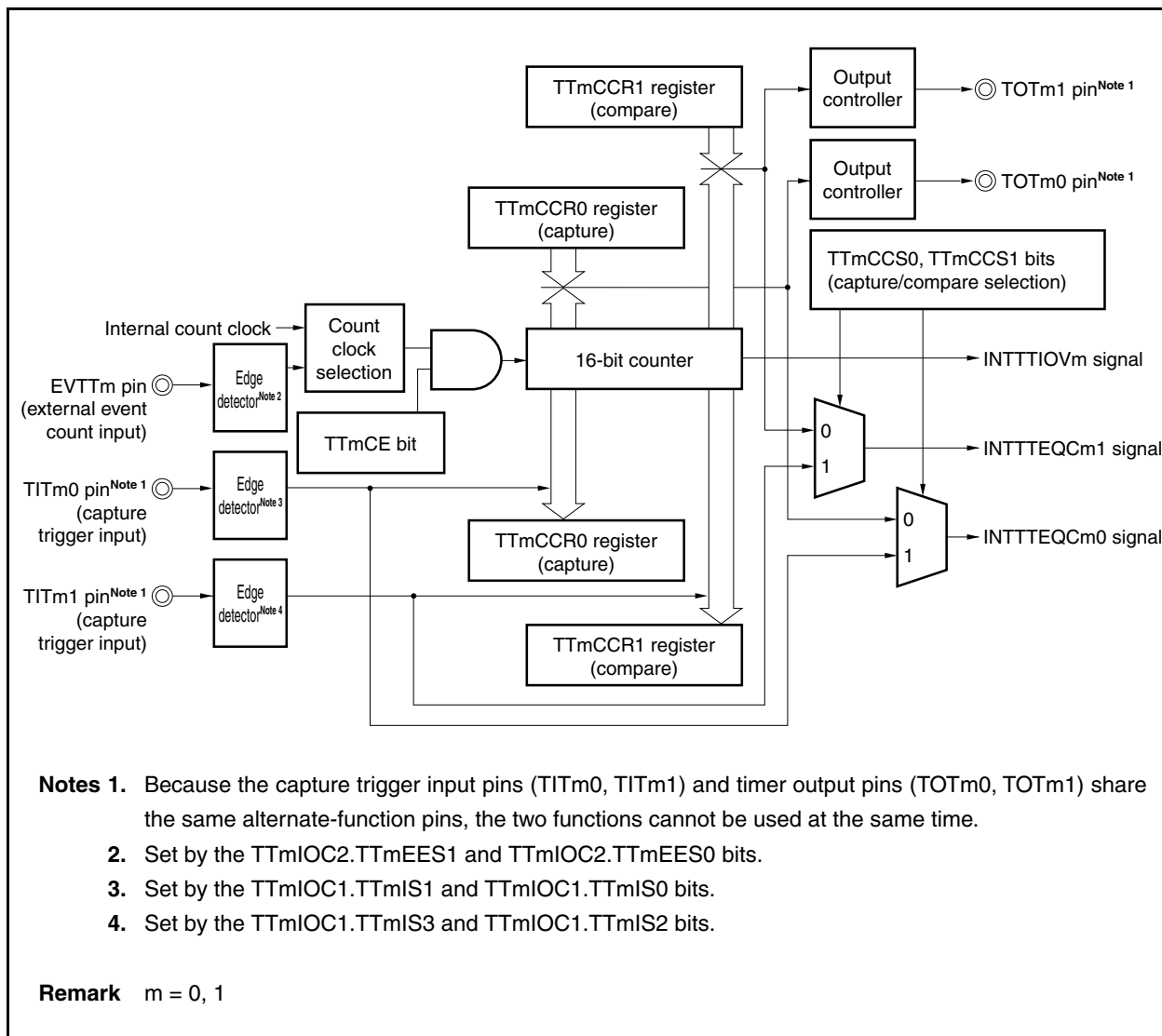
Figure 8-37. Configuration of TMT0 and TMT1 in Free-Running Timer Mode
