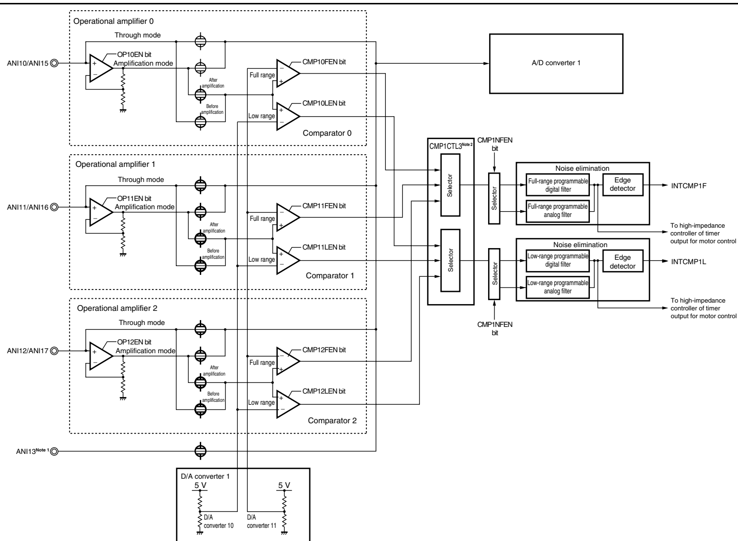
Figure 12-4. Block Diagram of Operational Amplifier for Input Level Amplification and Overvoltage Detection Comparator in A/D Converter 1
