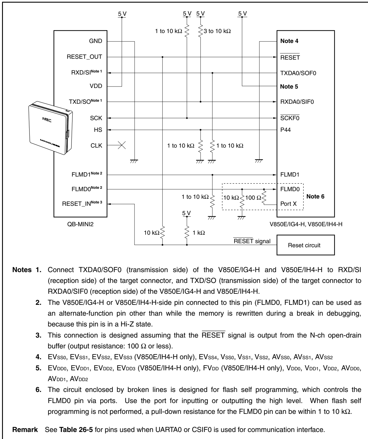
Figure 26-6. Circuit Connection Example When UARTA0/CSIF0 Is Used for Communication Interface
