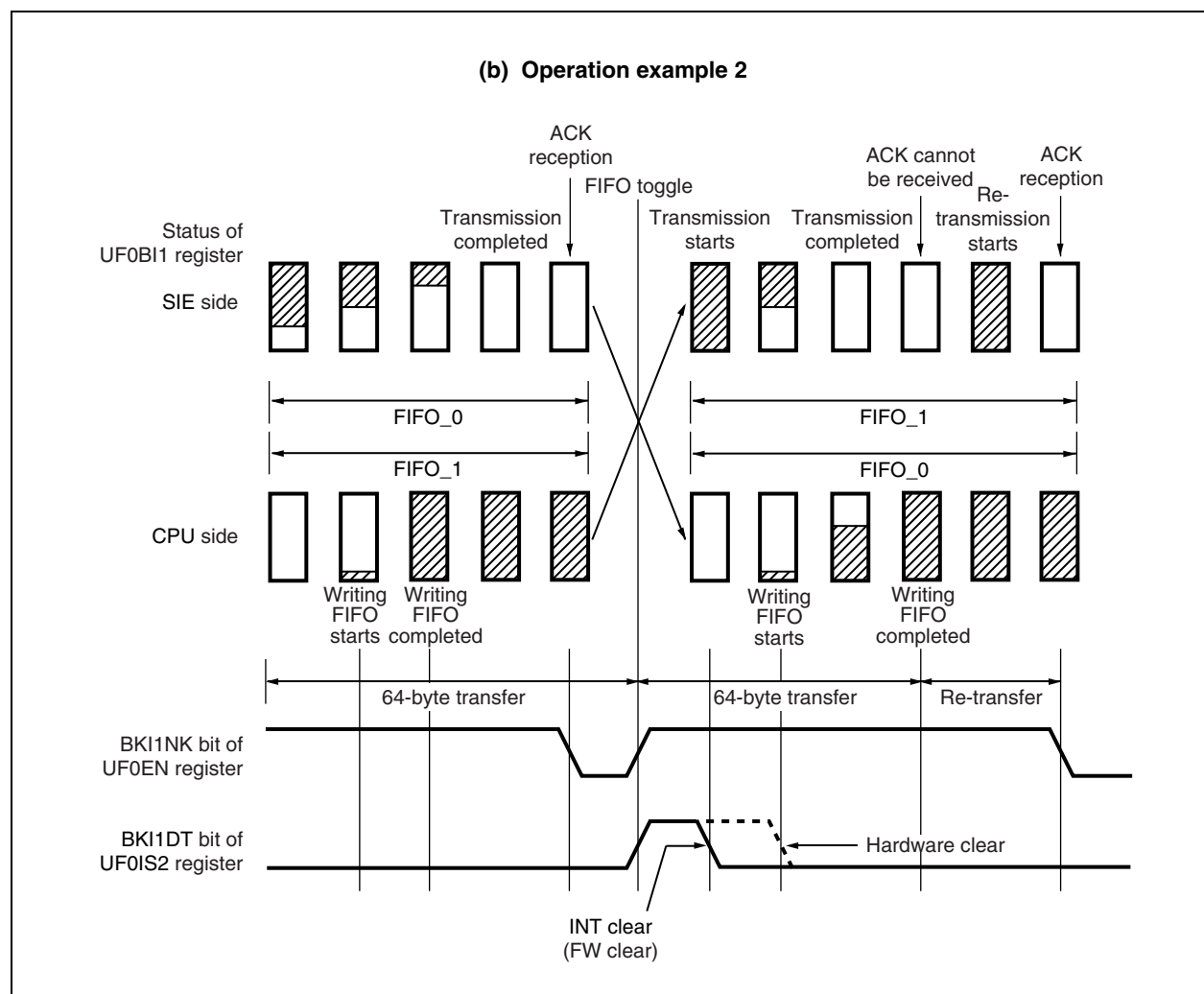
Figure 18-9. Operation of UF0BI1 Register (2/3)
