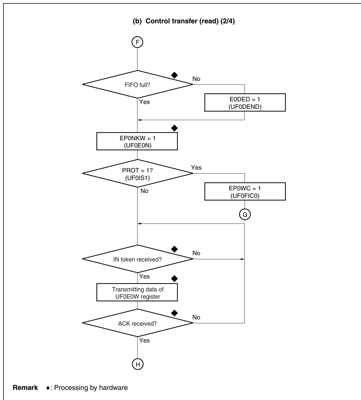
Figure 18-24 CPUDEC Request for Control Transfer (4/12)
