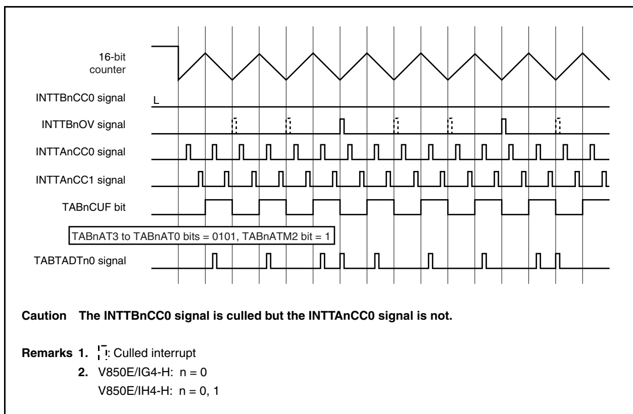
Figure 10-40. Example of A/D Conversion Start Trigger (TABTADTn0) Signal Output (TABnOPT1.TABnICE Bit = 0, TABnOPT1.TABnIOE Bit = 1, TABnOPT1.TABnID4 to TABnOPT1.TABnID0 Bits = 00010: With Interrupt Culling) (2)
