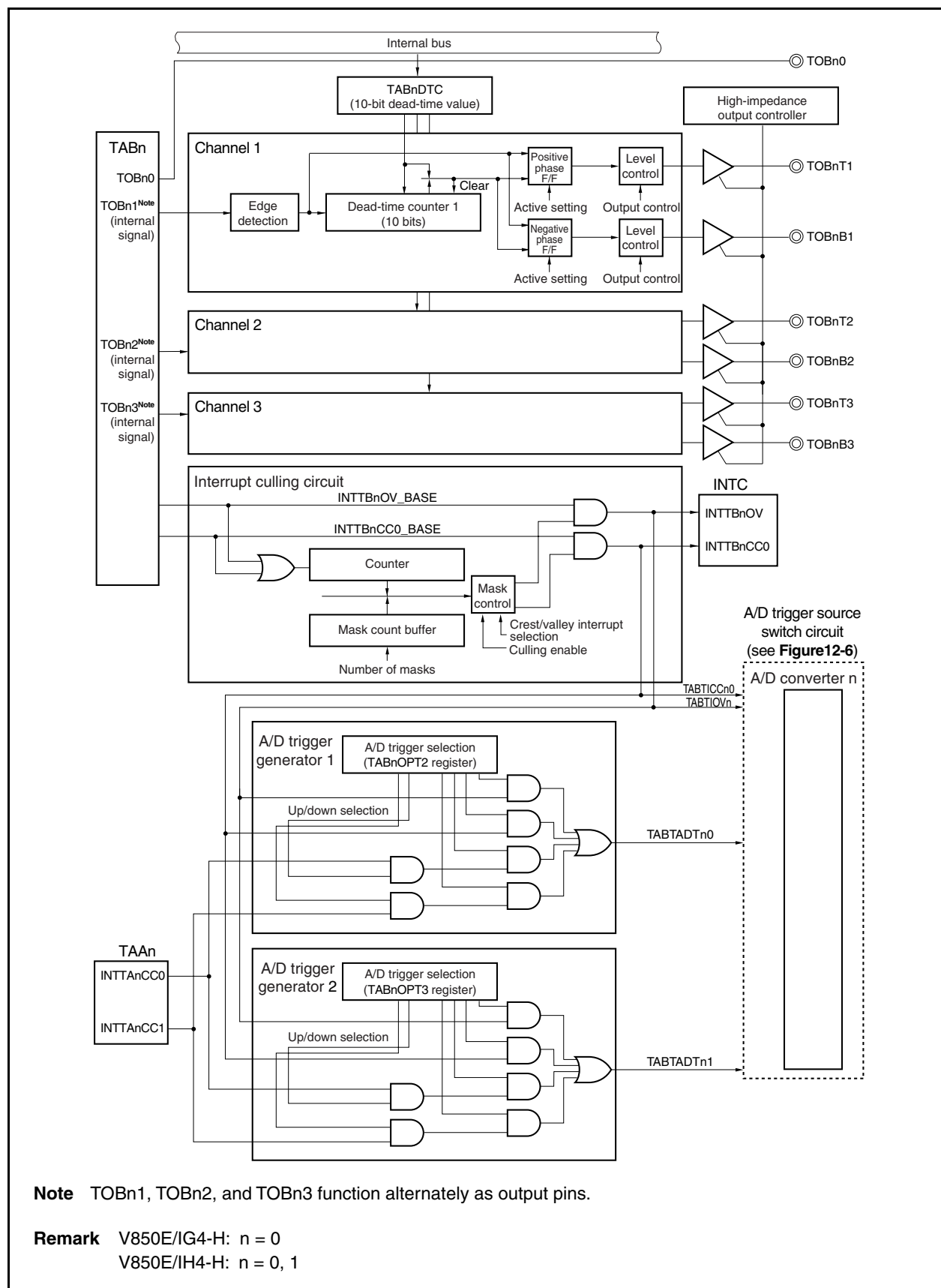
Figure 10-2. TMQn Option
