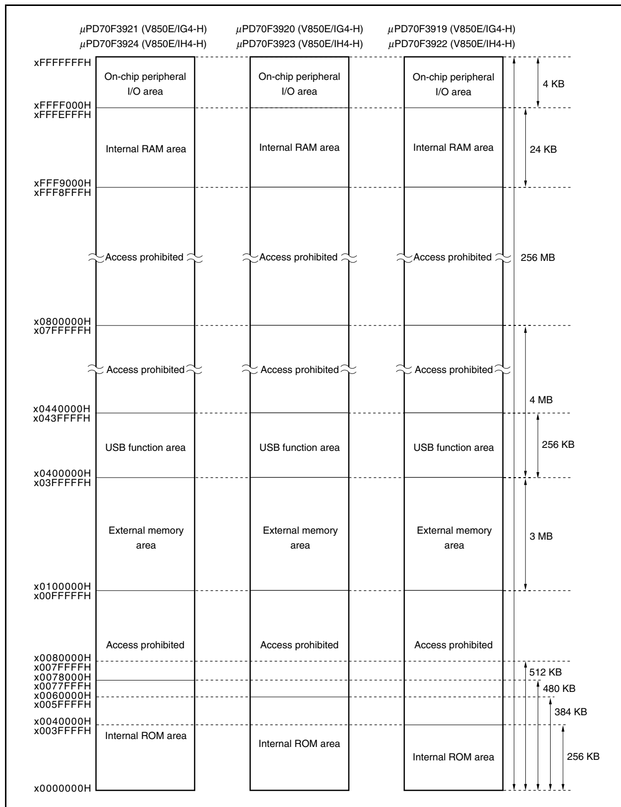
Figure 3-4. Memory Map
