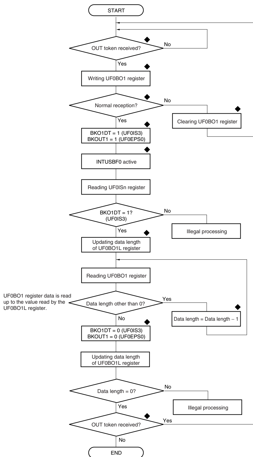
Figure 18-27. Normal Processing for Bulk Transfer (OUT) (Endpoint2)
