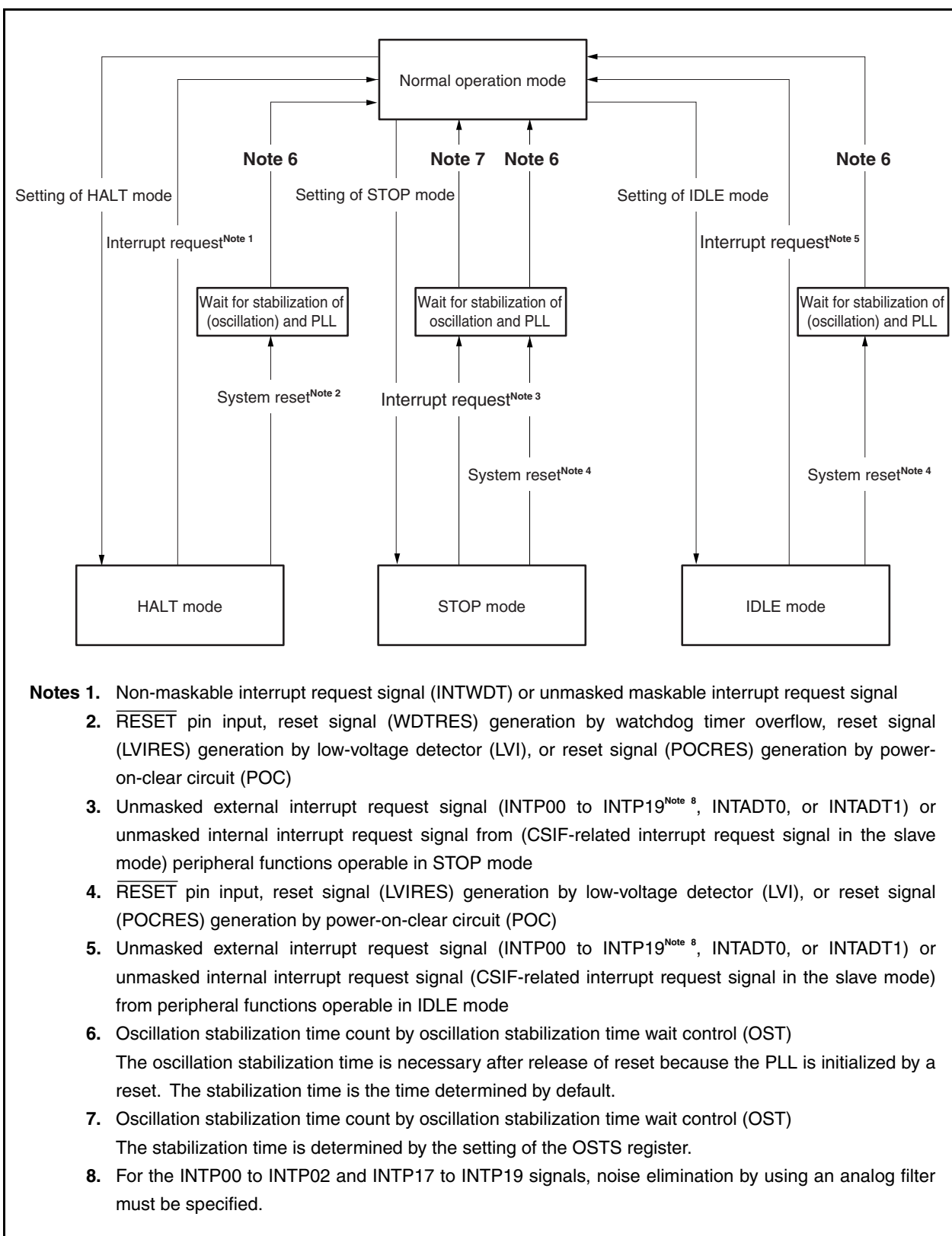
Figure 22-1. Status Transition
