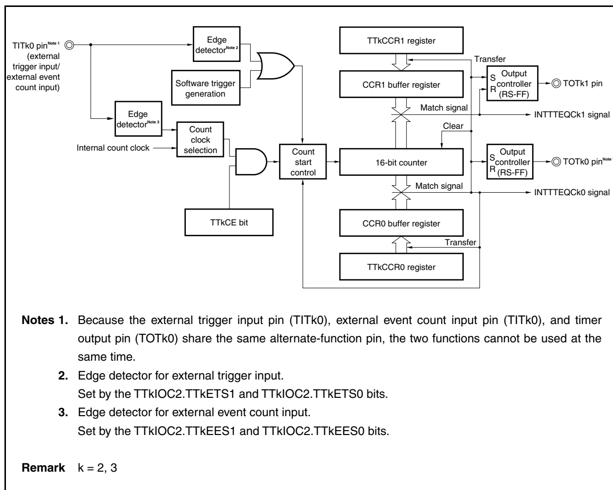
Figure 8-28. Configuration of TMT2 and TMT3 in One-Shot Pulse Output Mode
