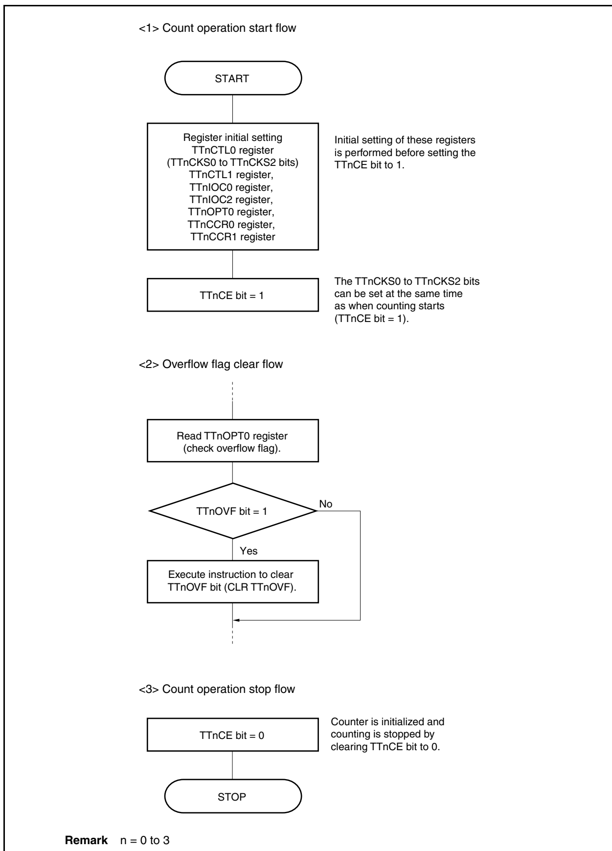
Figure 8-42. Software Processing Flow in Free-Running Timer Mode (Compare Function) (2/2)
