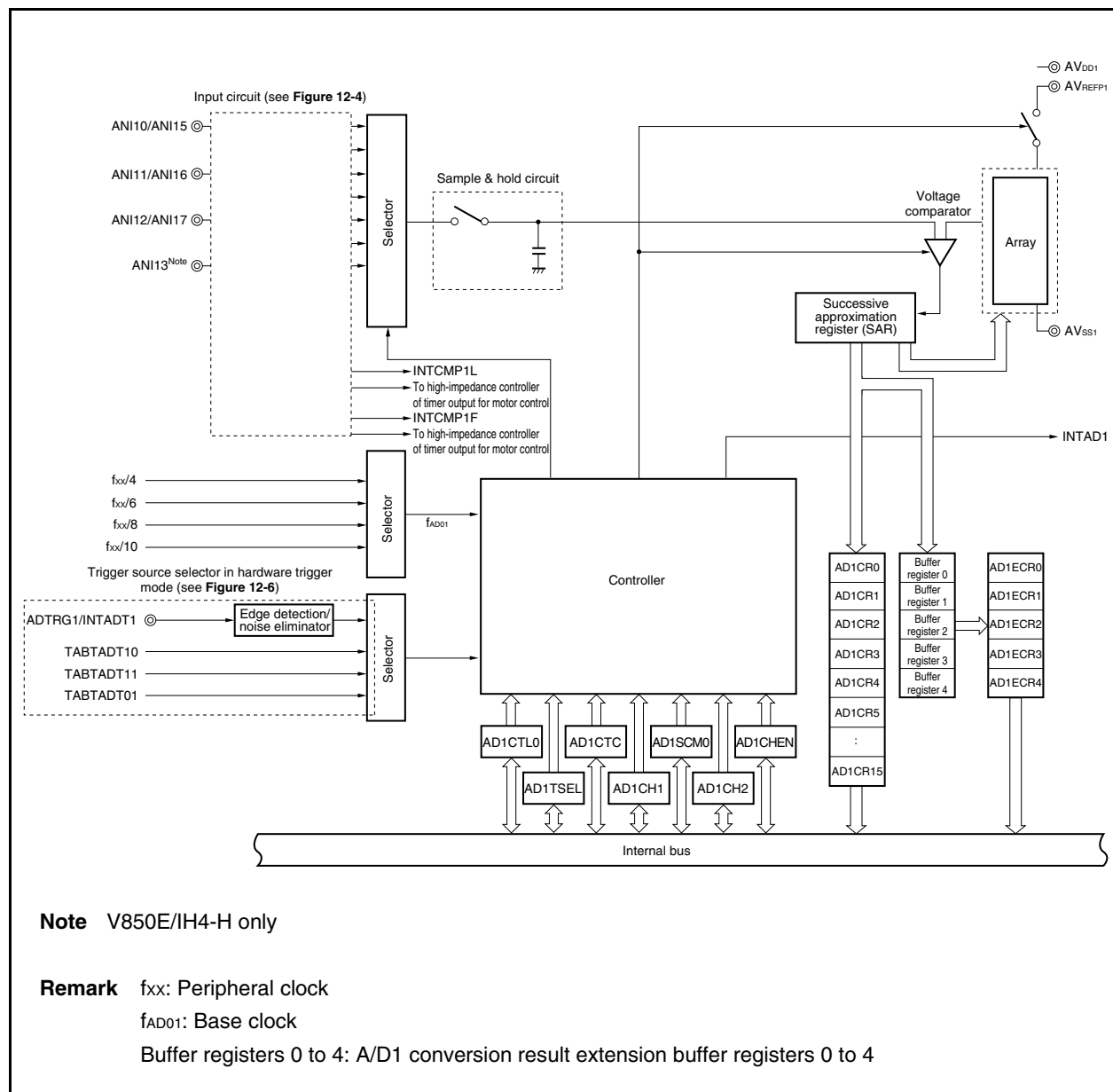
Figure 12-2. Block Diagram of A/D Converter 1
