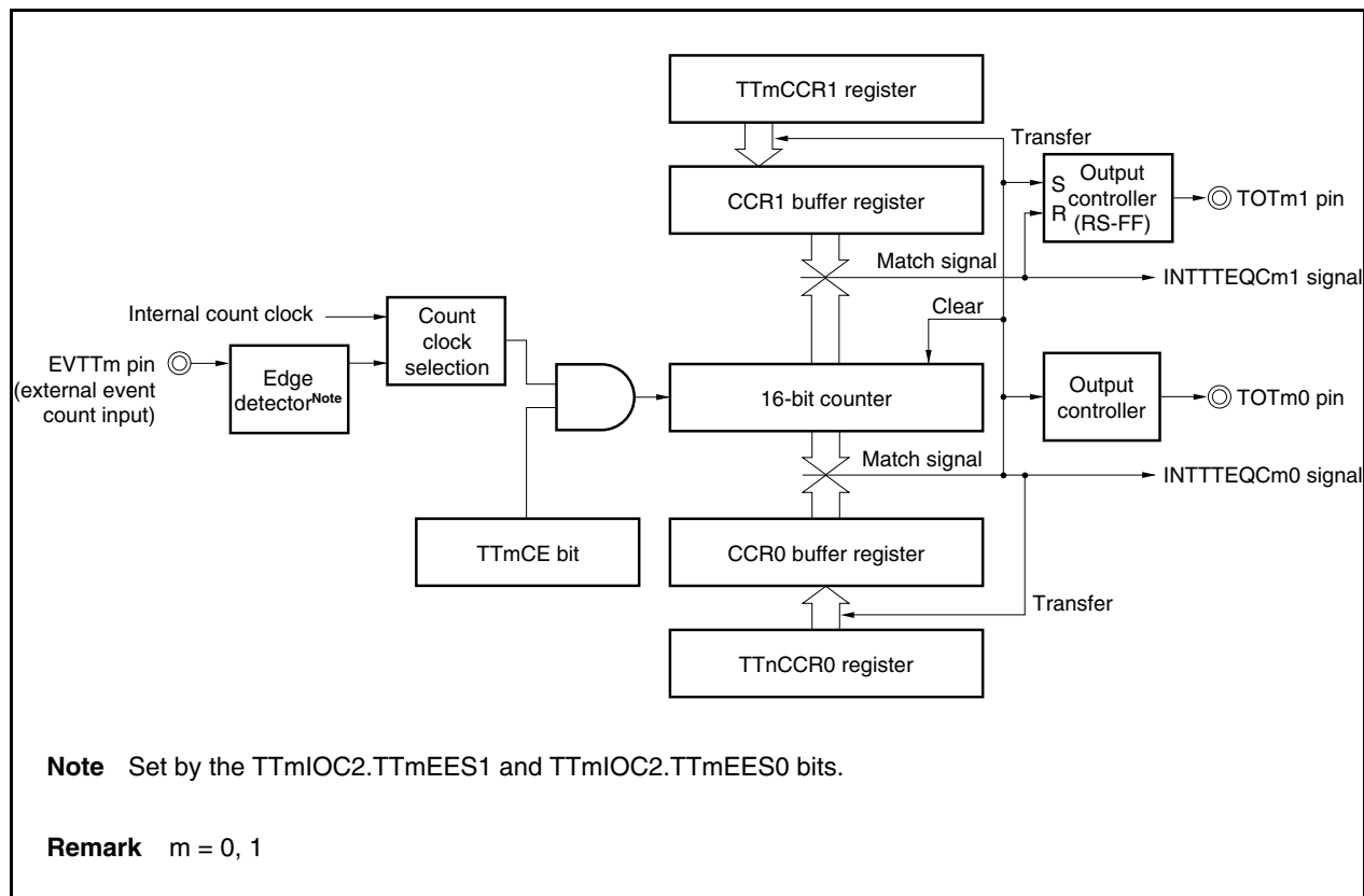
Figure 8-32. Configuration of TMT0 and TMT1 in PWM Output Mode
