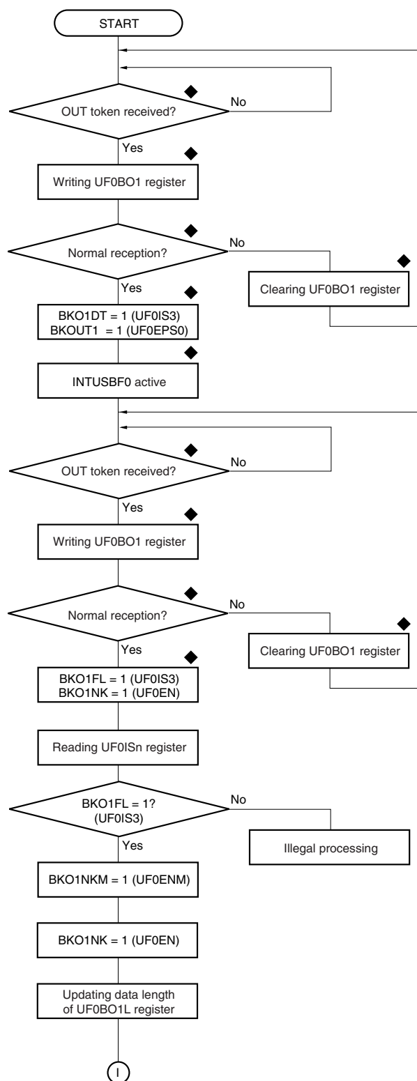
Figure 18-28. Processing If More Data Than Expected by System Is Transmitted (Endpoint2) (1/2)
