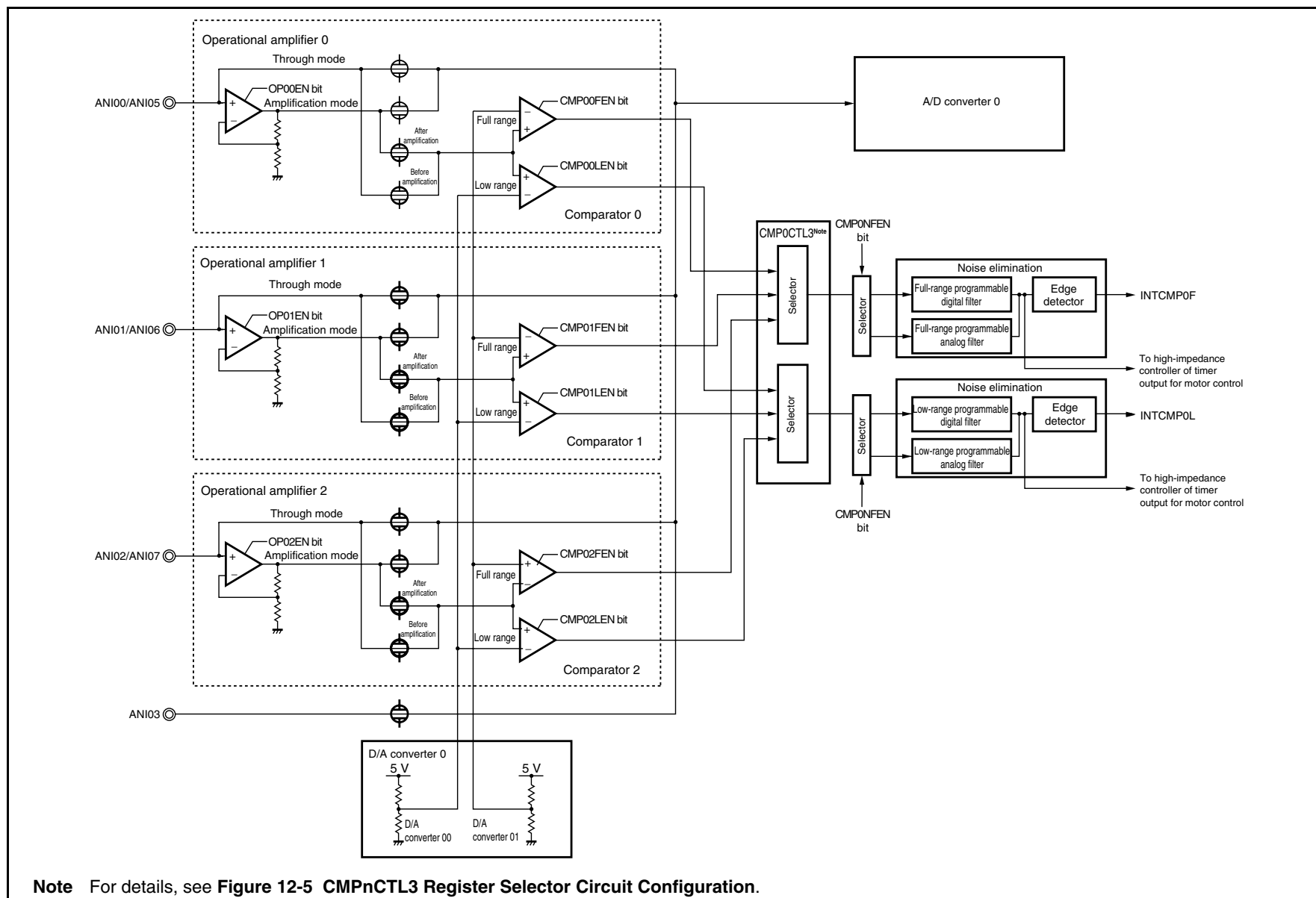
Figure 12-3. Block Diagram of Operational Amplifier for Input Level Amplification and Overvoltage Detection Comparator in A/D Converter 0
