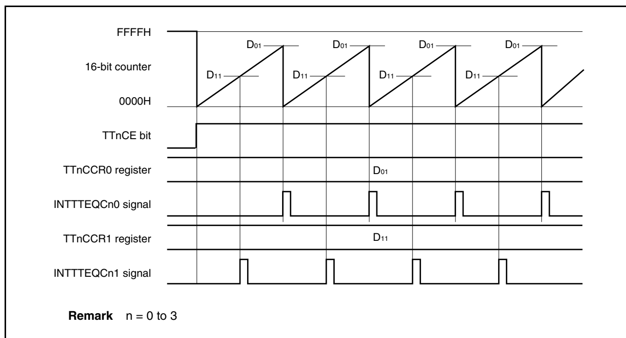
Figure 8-20. Timing Chart When D_{01} \geq D_{11}
