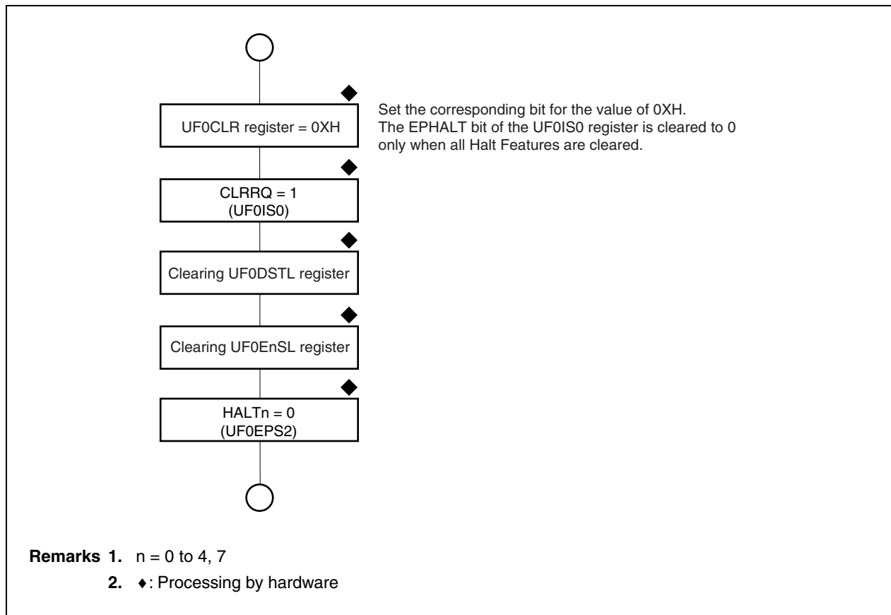
Figure 18-20. CLEAR_FEATURE Processing
