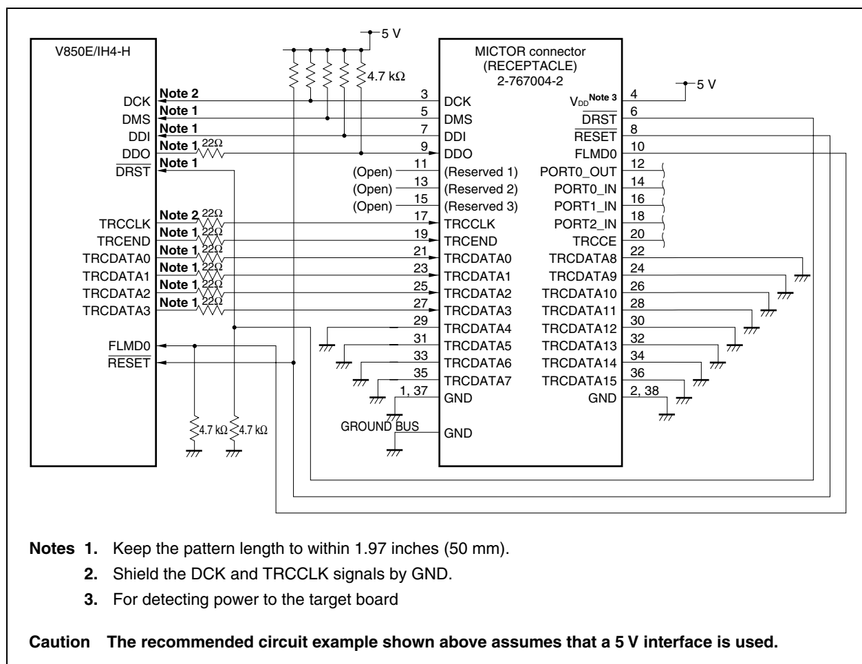
Figure 26-2. Example of Recommended Emulator Connection Circuit
