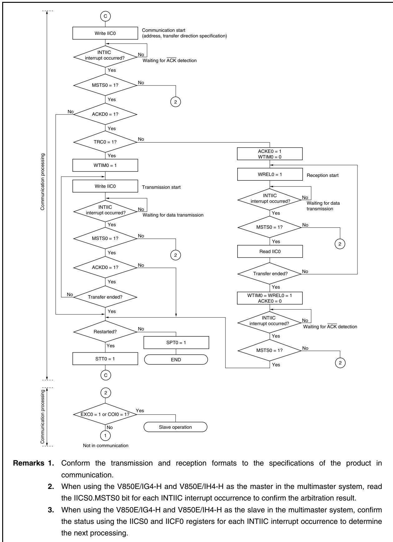
Figure 17-17. Master Operation in Multimaster System (3/3)
