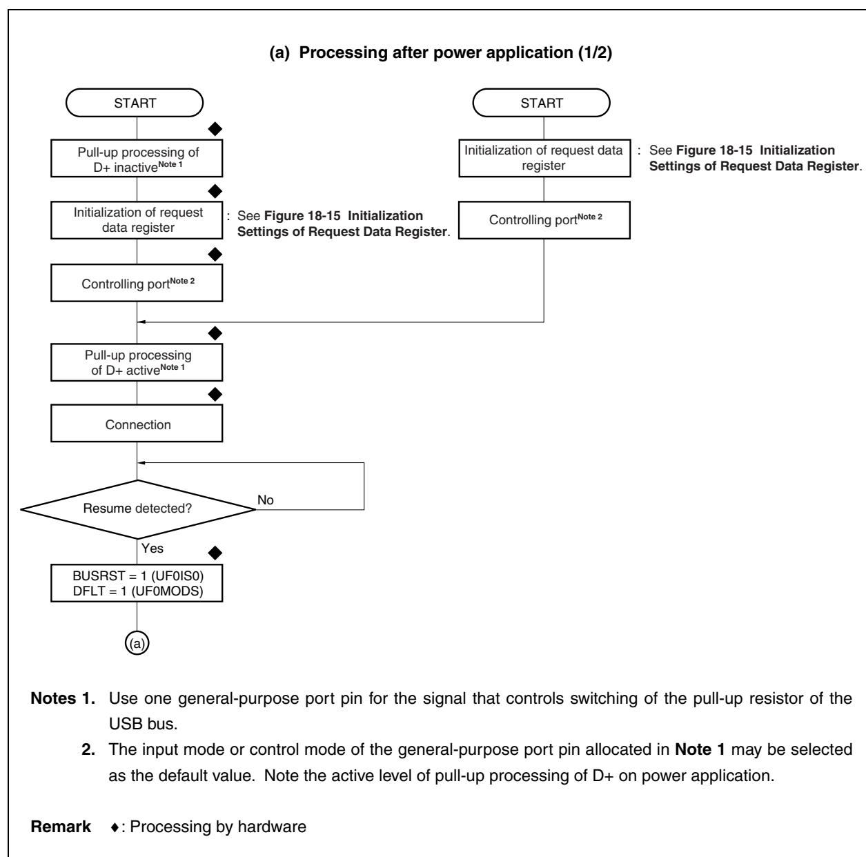
Figure 18-31. Example of Processing After Power Application/Power Failure (1/3)
