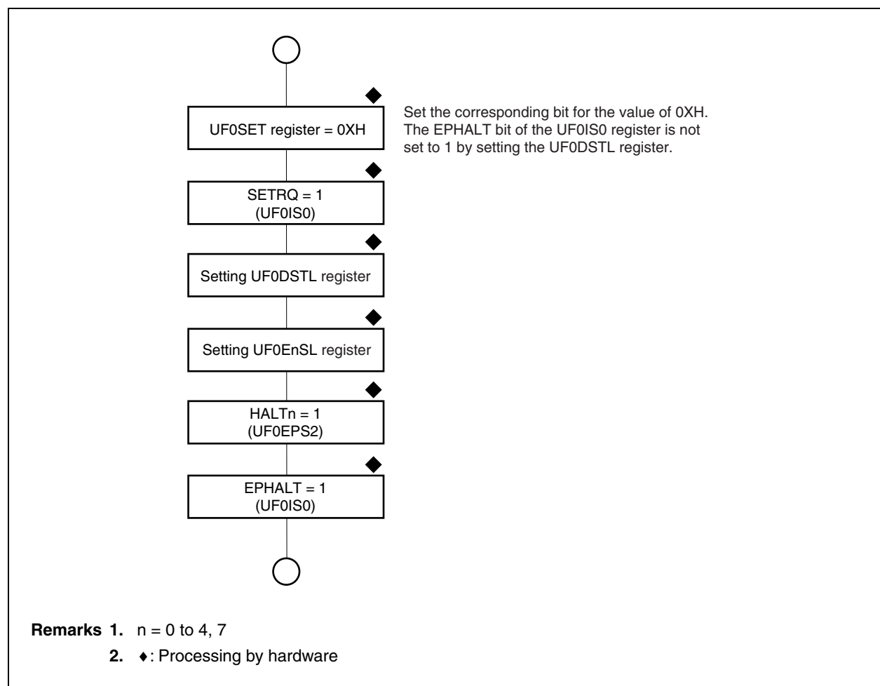
Figure 18-21. SET_FEATURE Processing
