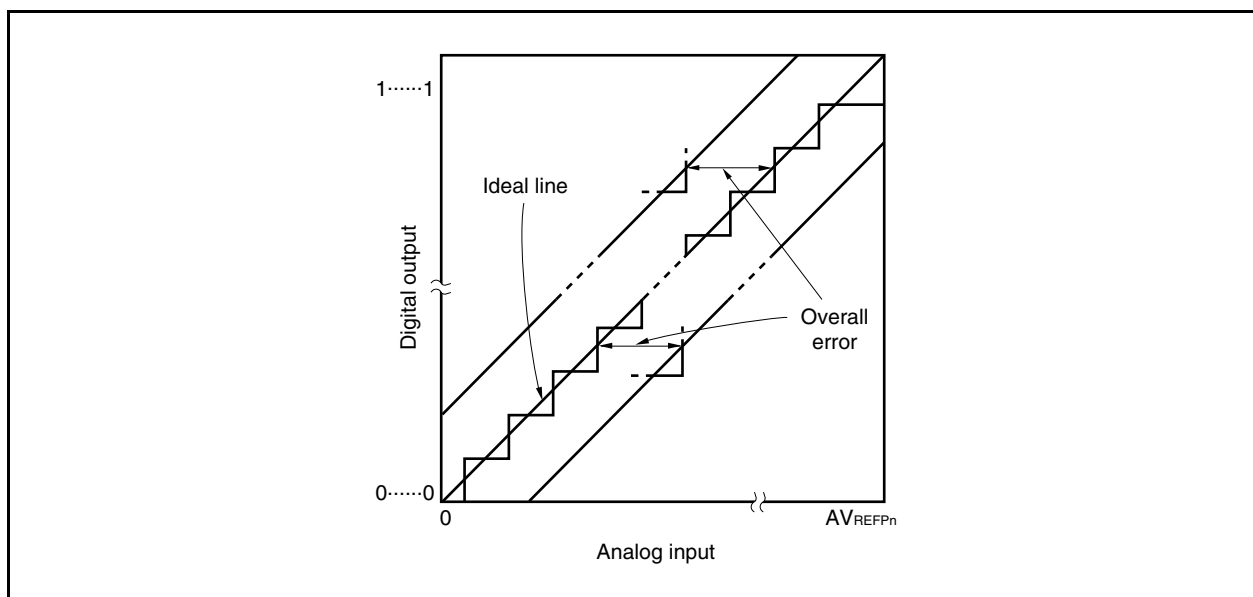
Figure 12-23. Overall Error
