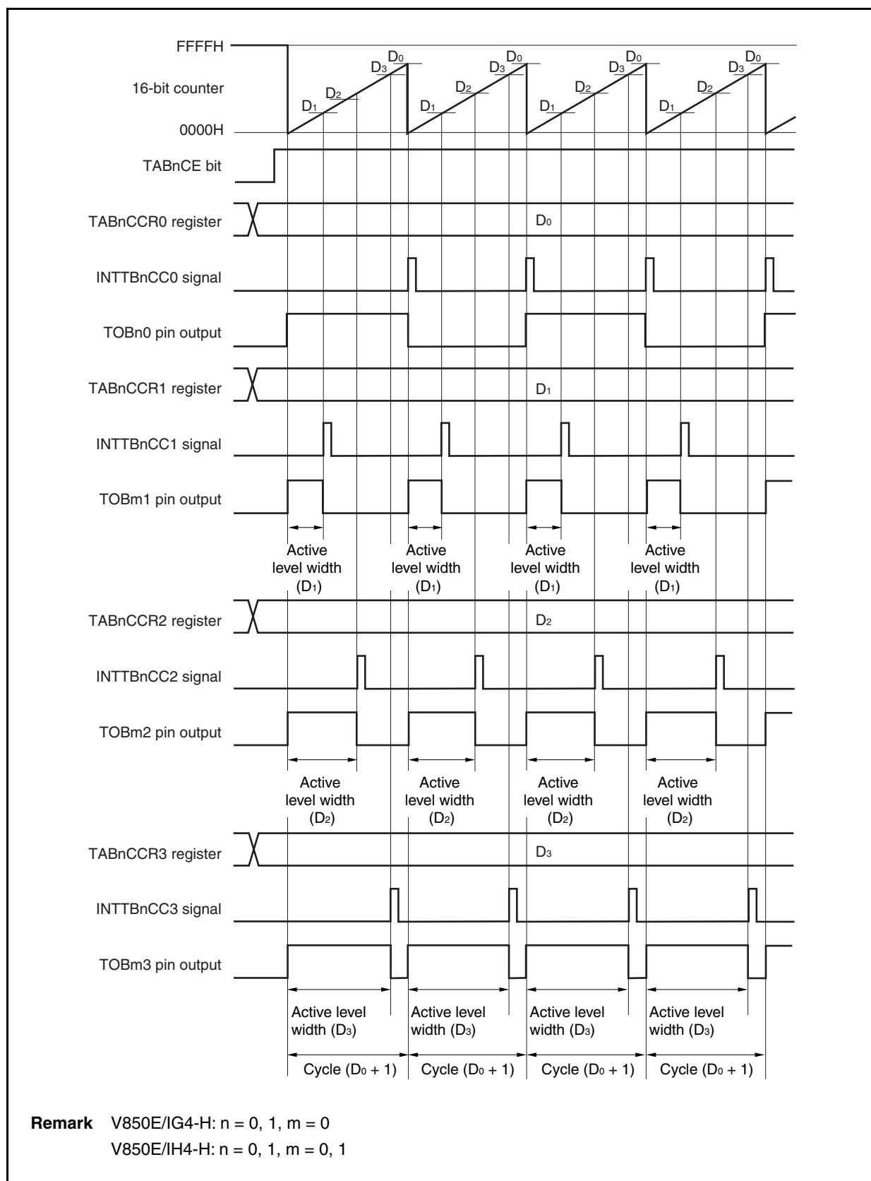
Figure 7-30. Basic Timing in PWM Output Mode
