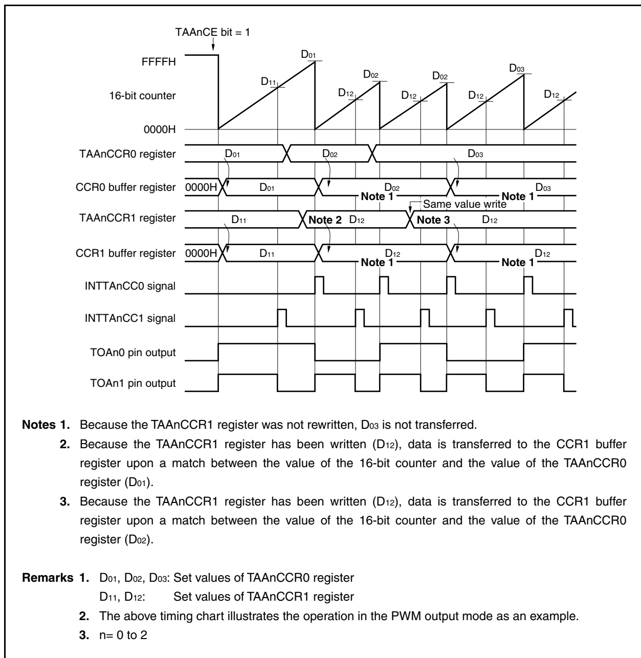
Figure 6-7. Timing of Batch Write
