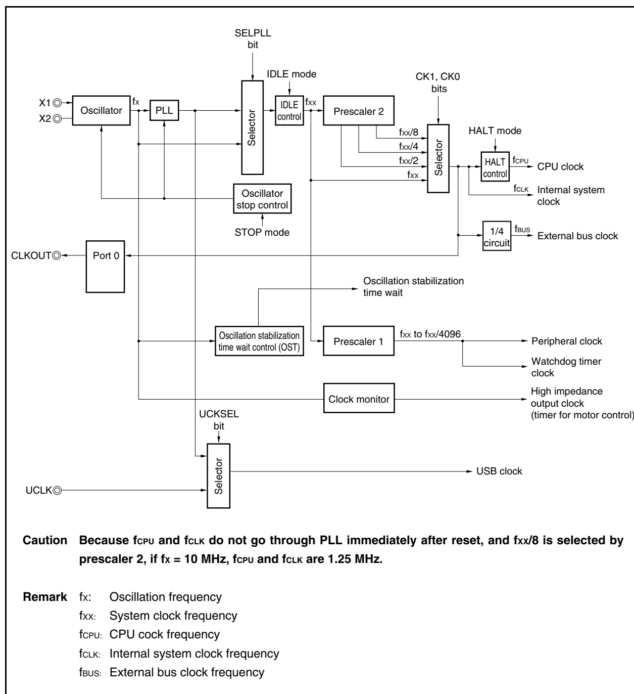
Figure 5-1. Clock Generator
