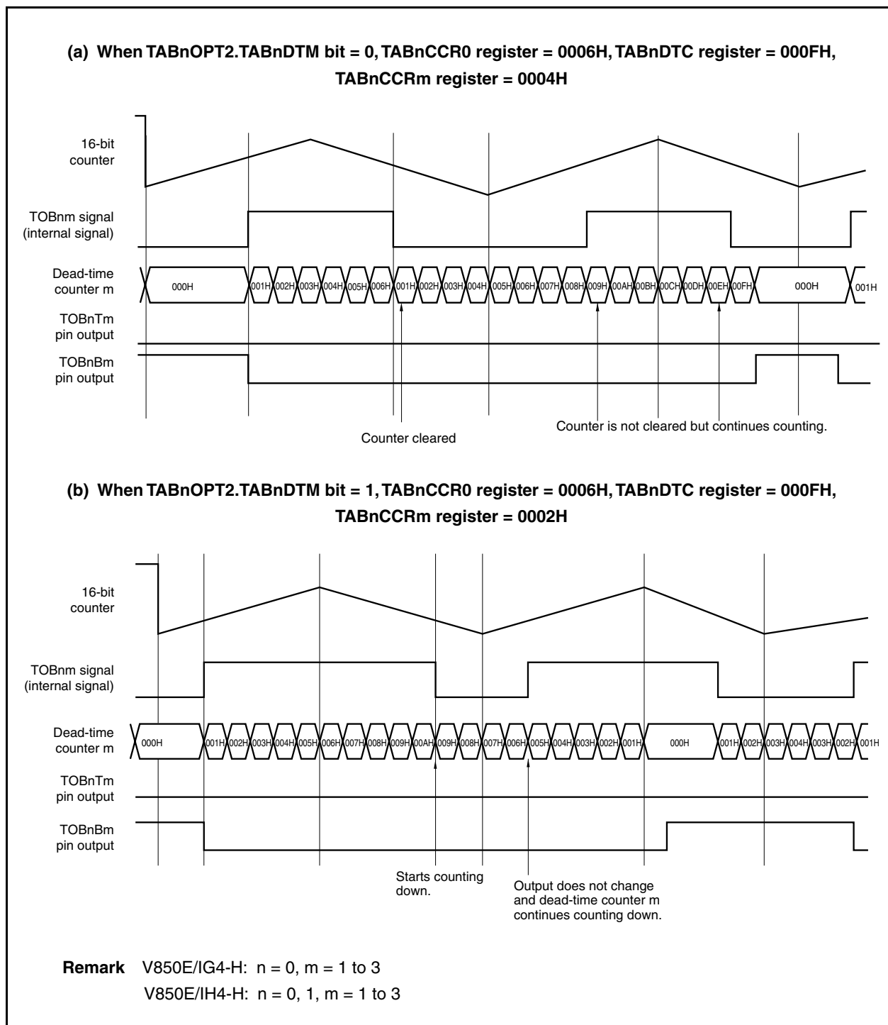
Figure 10-14. Operation of Dead-Time Counter m (2)
