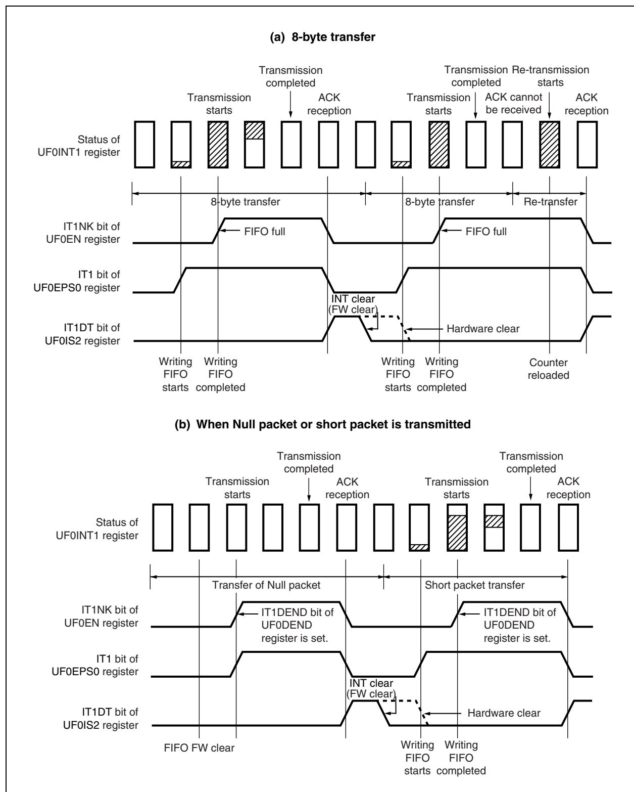
Figure 18-11. Operation of UF0INT1 Register
