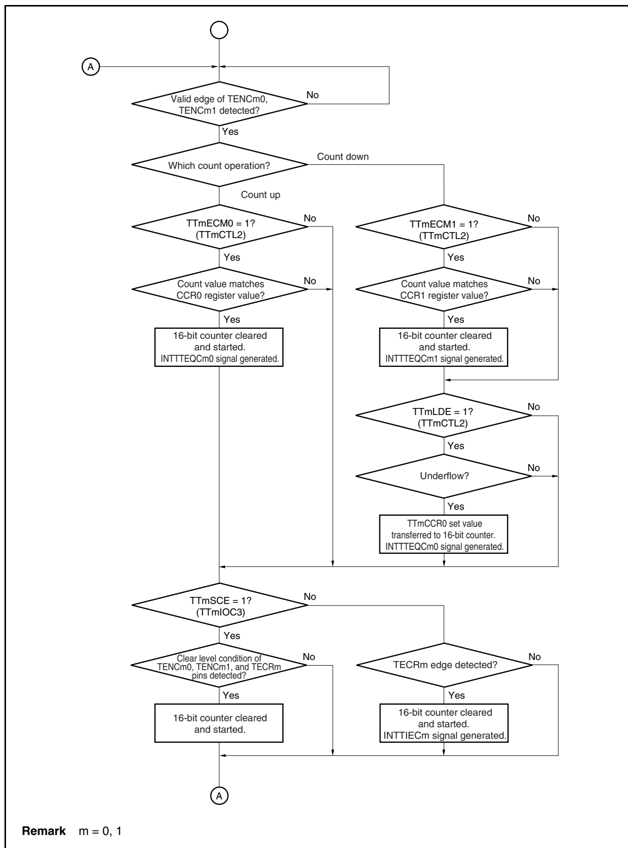
Figure 8-65. Encoder Compare Mode Operation Processing
