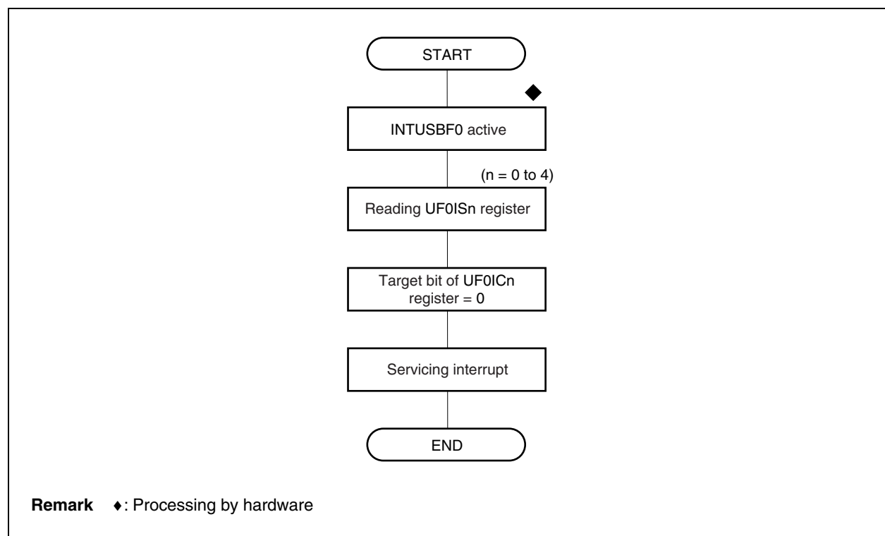
Figure 18-18. Interrupt Servicing
