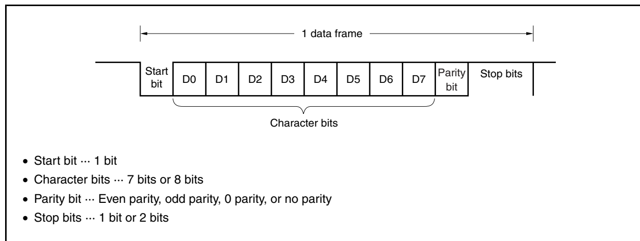
Figure 15-3. Asynchronous Serial Interface Transmit/Receive Data Format (LSB-First Transfer)
