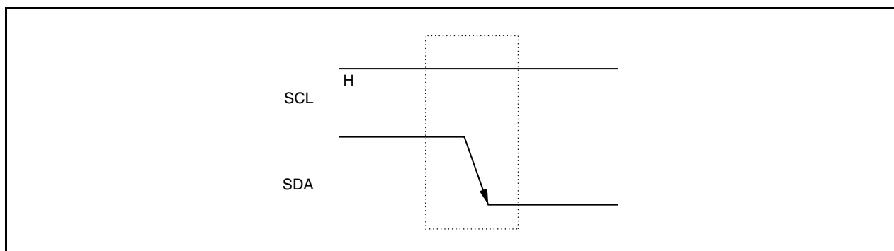
Figure 17-6. Start Conditions
