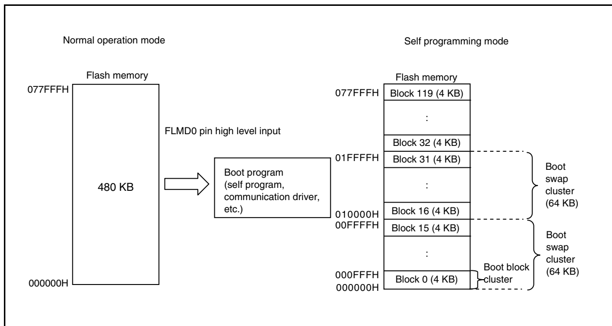
Figure 27-3. Self Programming
