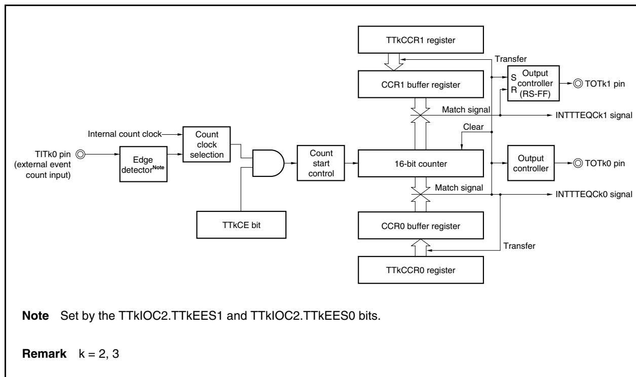
Figure 8-50. Configuration of TMT2 and TMT3 in Triangular-Wave PWM Output Mode
