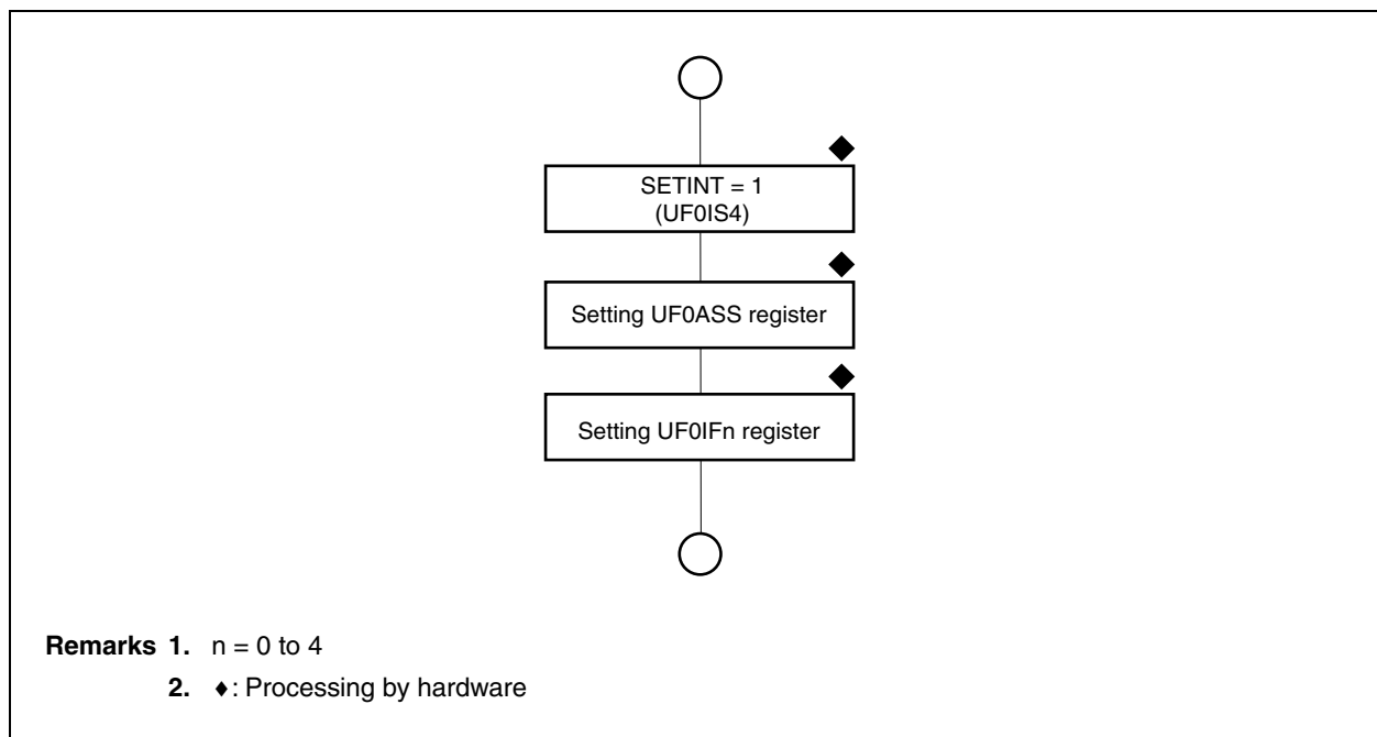
Figure 18-23. SET_INTERFACE Processing
