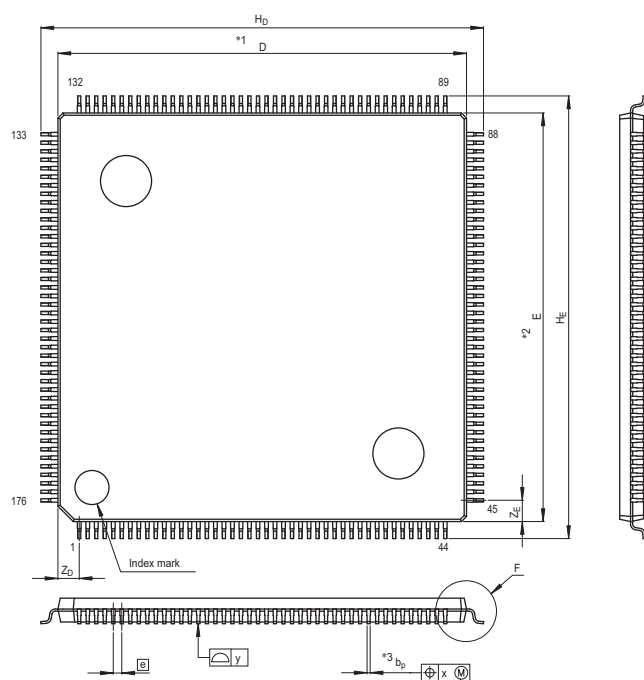
Figure C 176-Pin LQFP (PLQP0176KB-A)
