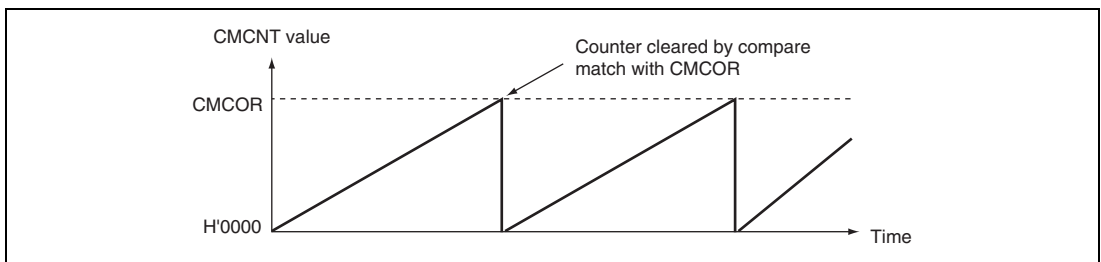
Figure 12.2 Counter Operation
