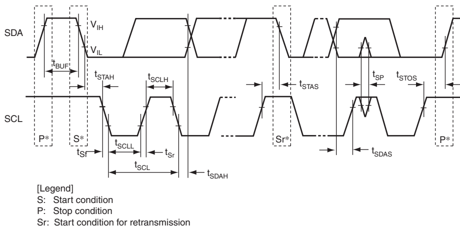
Figure 37.53 (1) Input/Output Timing
