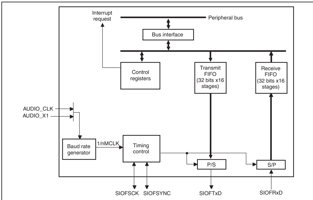
Figure 20.1 Block Diagram
