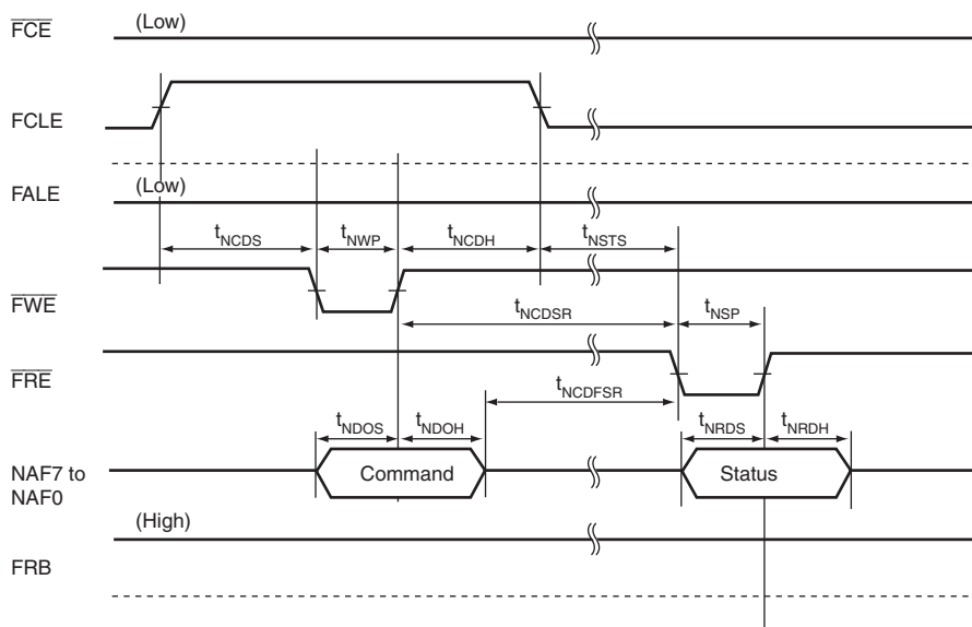
Figure 37.65 NAND Type Flash Memory Status Read Timing
