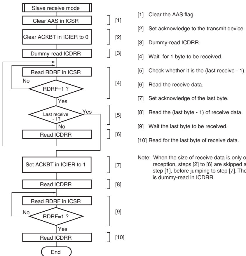
Figure 18.21 Sample Flowchart for Slave Receive Mode
