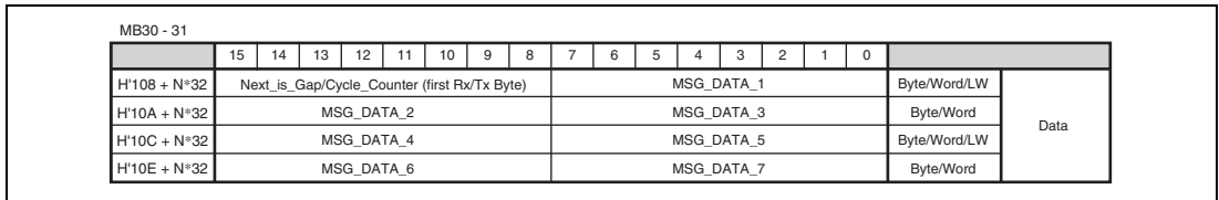
Figure 21.5 Message Data Field
