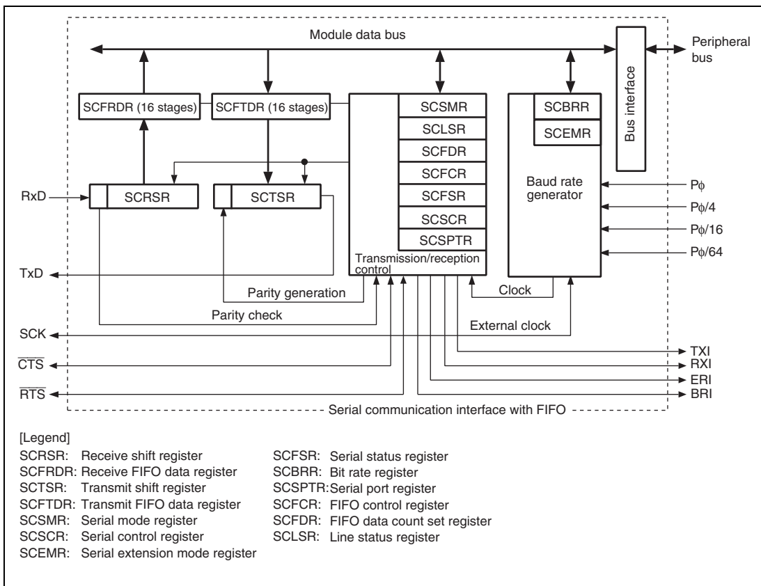
Figure 15.1 Block Diagram
