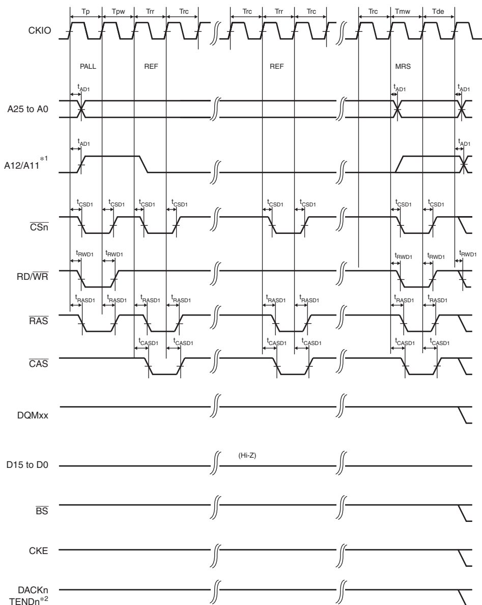
Figure 37.33 Synchronous DRAM Mode Register Write Timing (WTRP = 1 Cycle)
