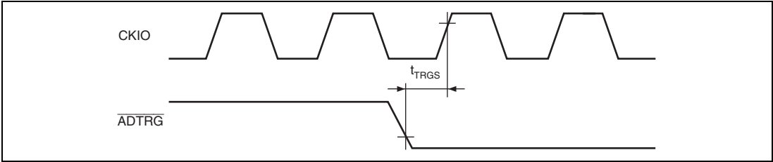
Figure 37.60 A/D Converter External Trigger Input Timing
