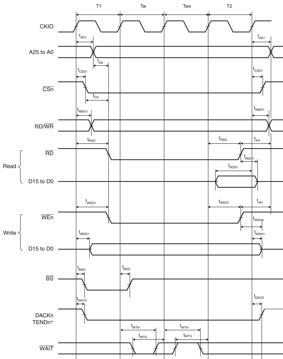
Figure 37.11 Basic Bus Timing for Normal Space (One Software Wait Cycle, One External Wait Cycle)
