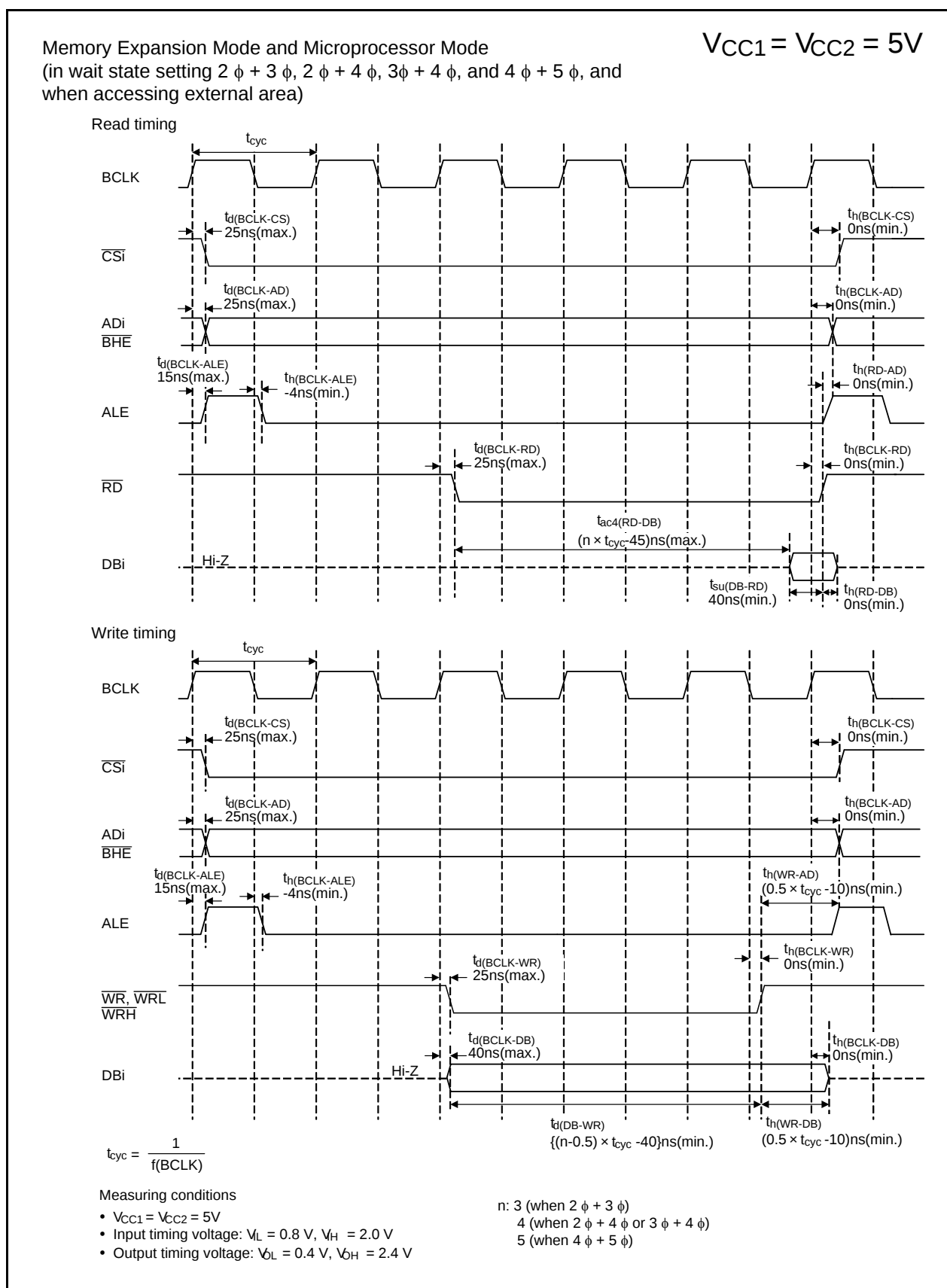
Figure 5.18 Timing Diagram
