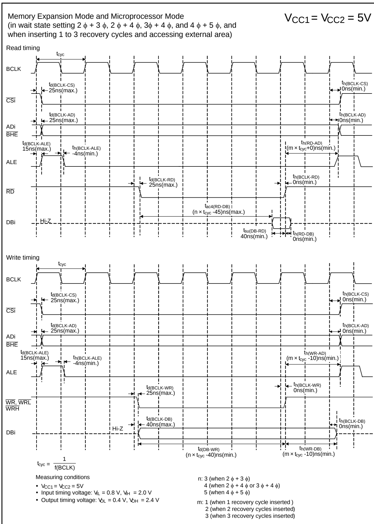
Figure 5.19 Timing Diagram
