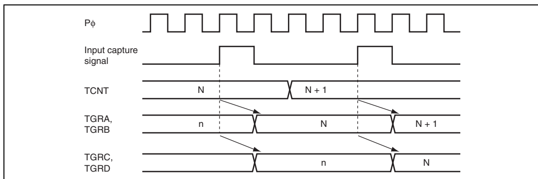
Figure 12.94 Buffer Operation Timing (Input Capture)
