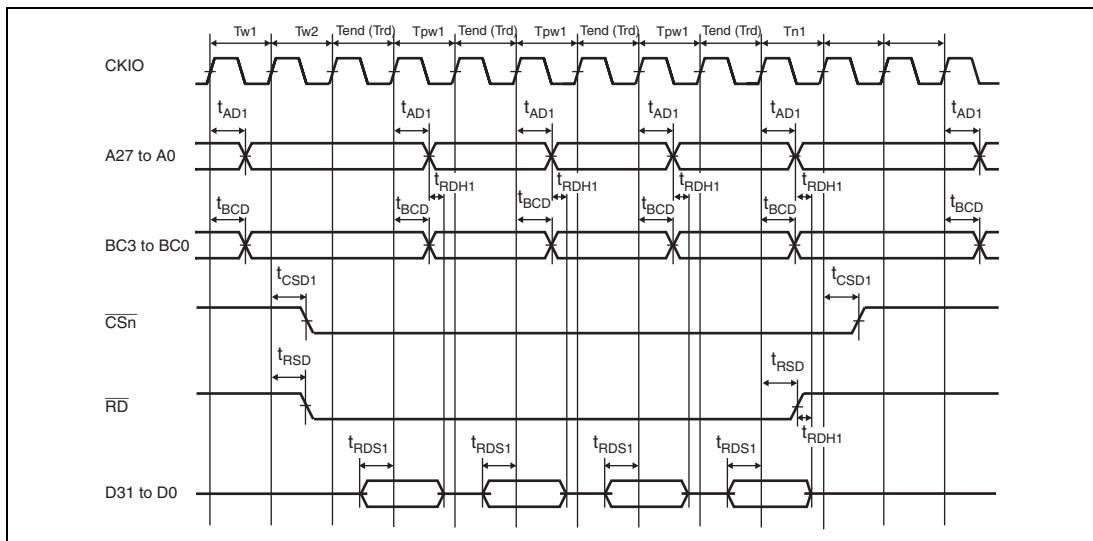
Figure 29.12 External Address Space: Basic Bus Timing
