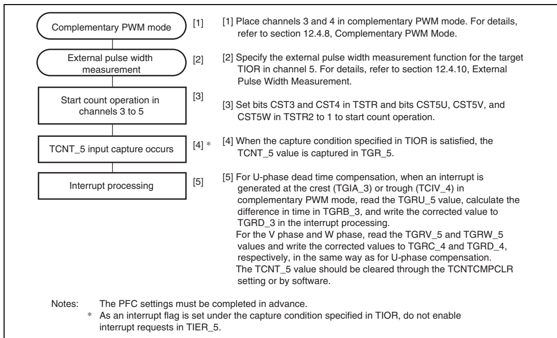
Figure 12.80 Example of Dead Time Compensation Setting Procedure
