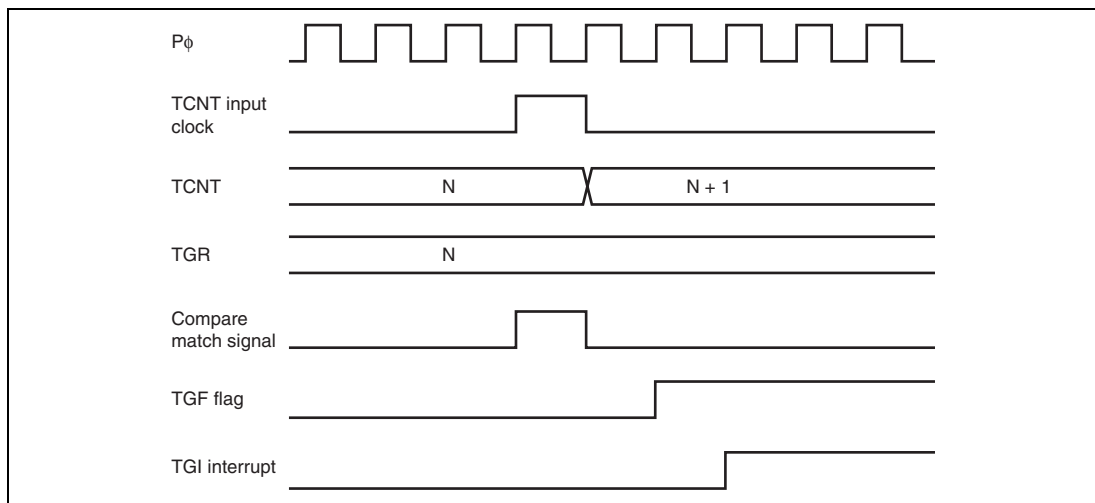
Figure 12.99 TGI Interrupt Timing (Compare Match) (Channels 0 to 4)
