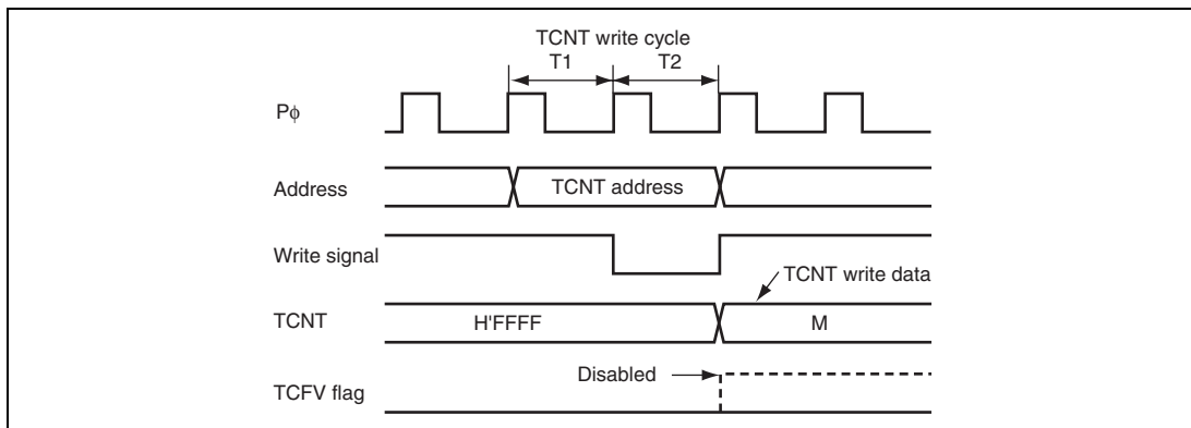
Figure 12.124 Contention between TCNT Write and Overflow
