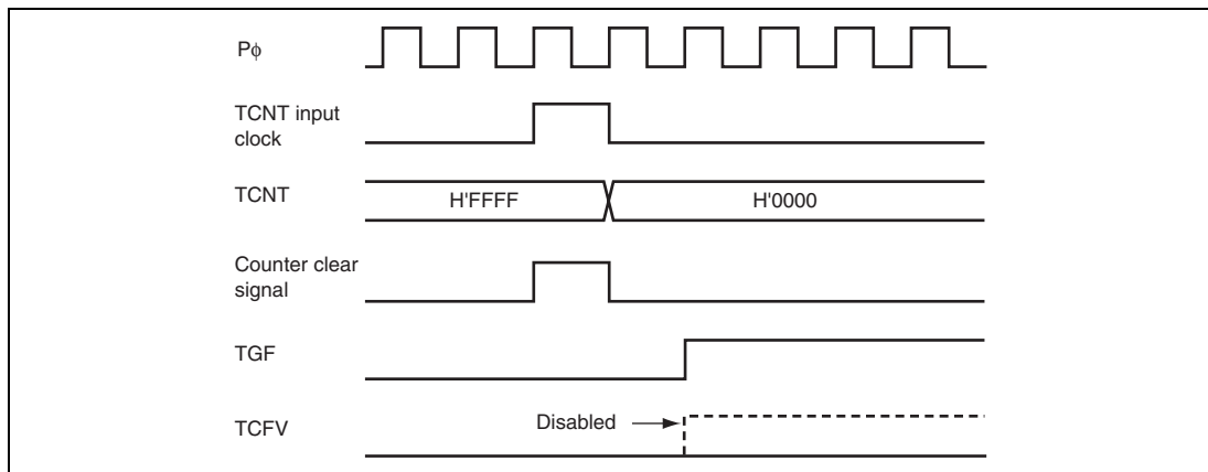
Figure 12.123 Contention between Overflow and Counter Clearing
