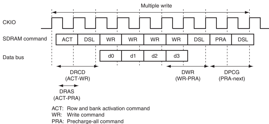
Figure 9.35 Multiple Write Timing Example 3
