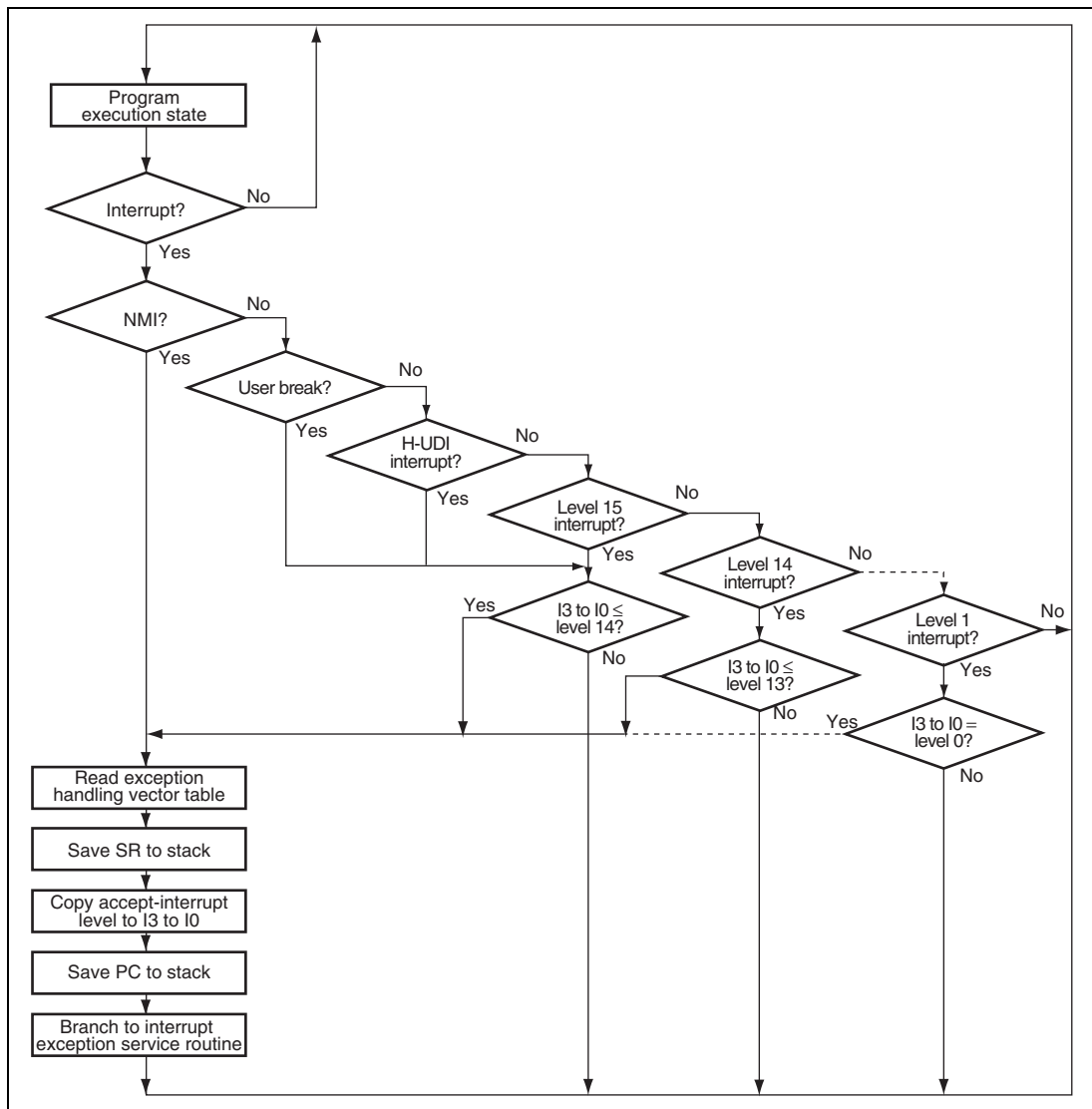
Figure 6.2 Interrupt Operation Flow
