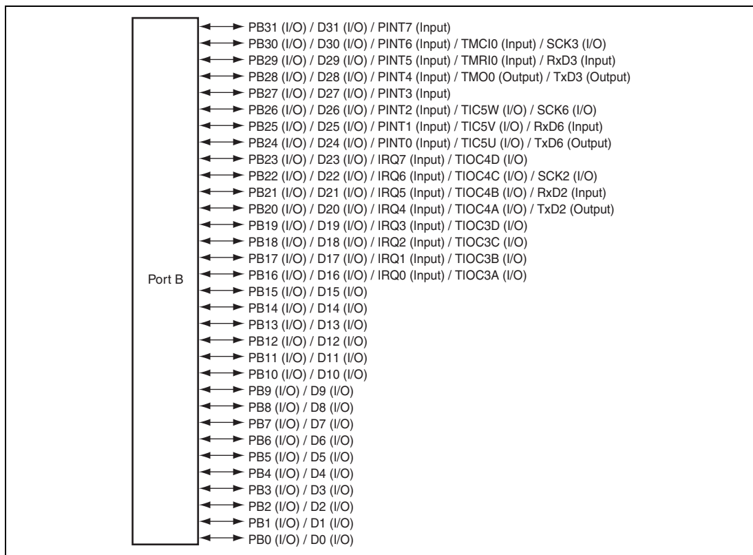
Figure 22.2 Port B
