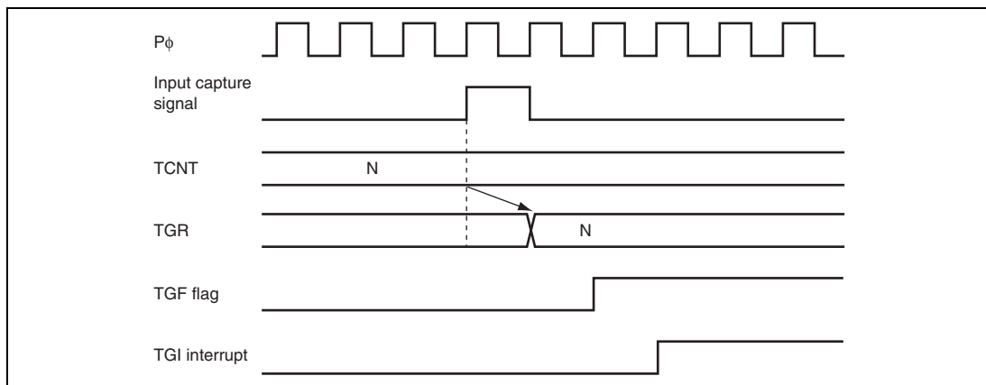
Figure 12.101 TGI Interrupt Timing (Input Capture) (Channels 0 to 4)
