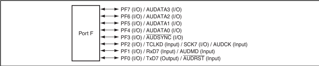
Figure 22.6 Port F
