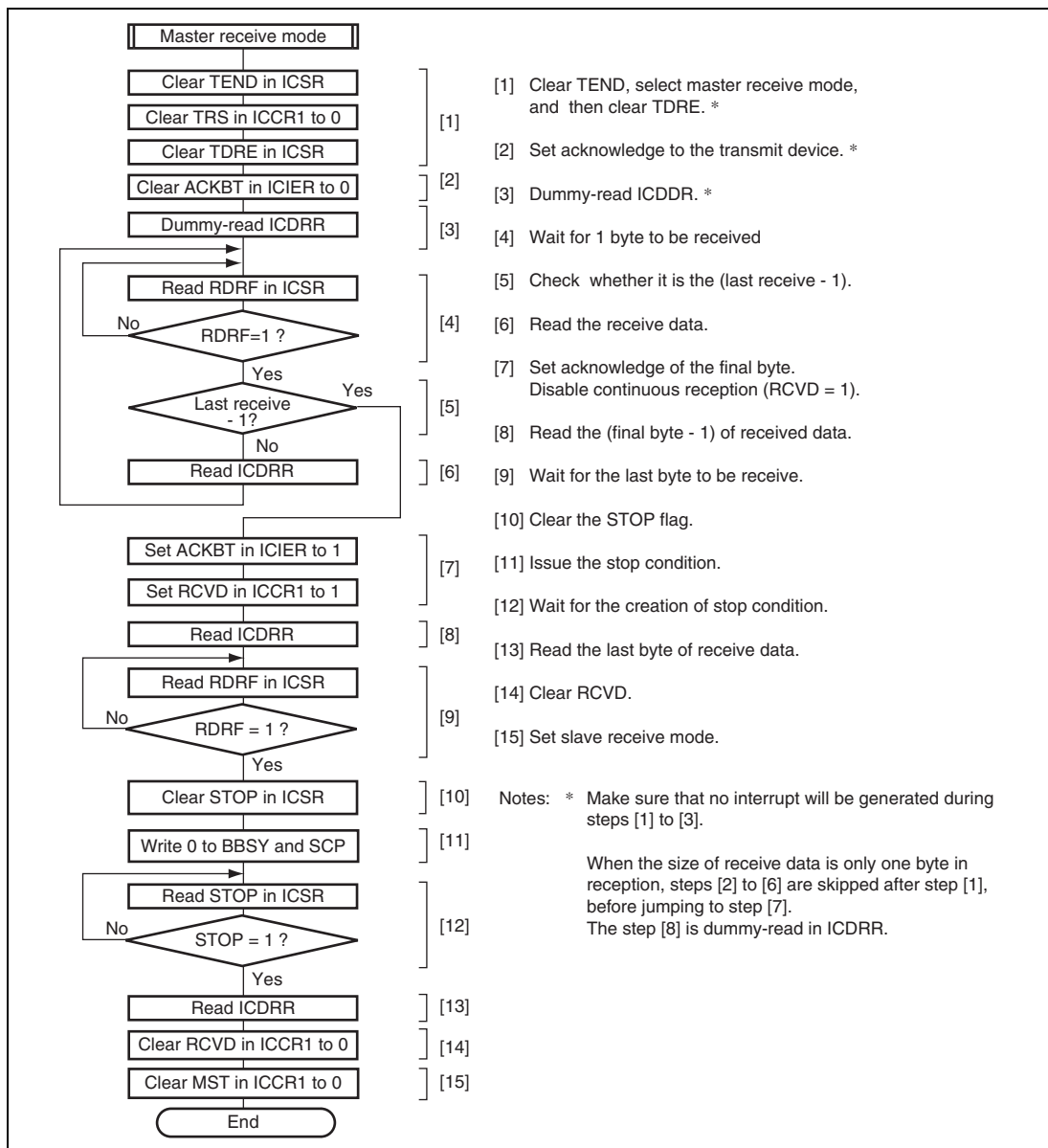
Figure 17.19 Sample Flowchart for Master Receive Mode
