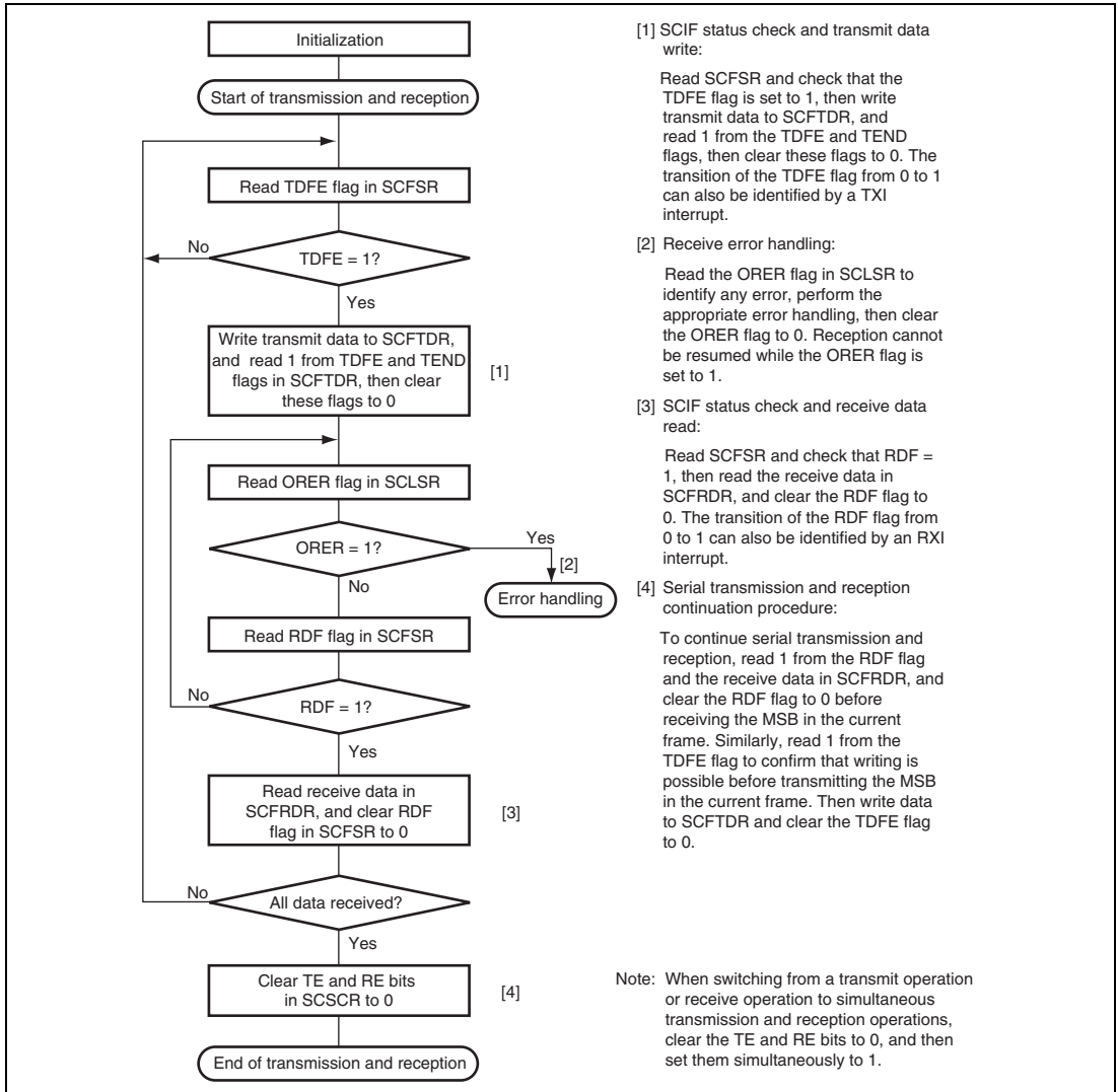
Figure 16.16 Sample Flowchart for Transmitting/Receiving Serial Data
