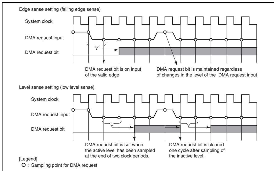
Figure 11.6 Example of Timing between DMA Request Input and DMA Request Bit
