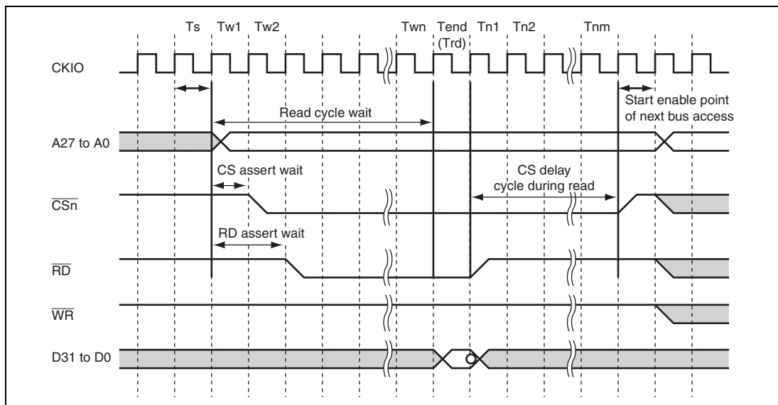
Figure 9.2 Basic Bus Timing (Read Operation)
