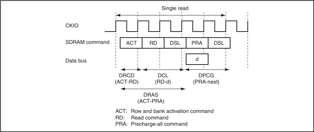
Figure 9.36 Single Read Timing Example 1
