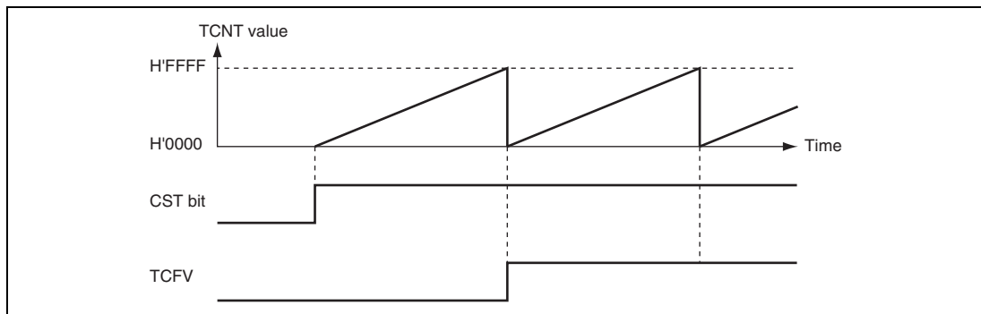
Figure 12.5 Free-Running Counter Operation
