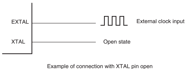
Figure 4.2 Example of Connecting External Clock
