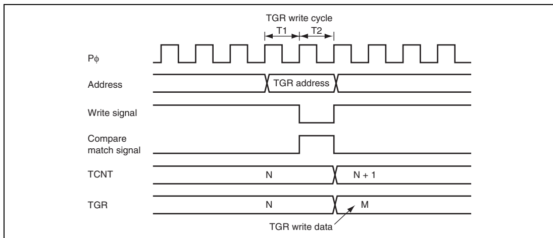
Figure 12.111 Contention between TGR Write and Compare Match
