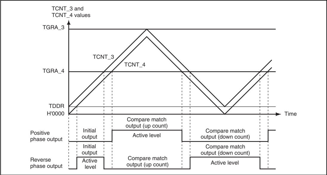
Figure 12.2 Complementary PWM Mode Output Level Example
