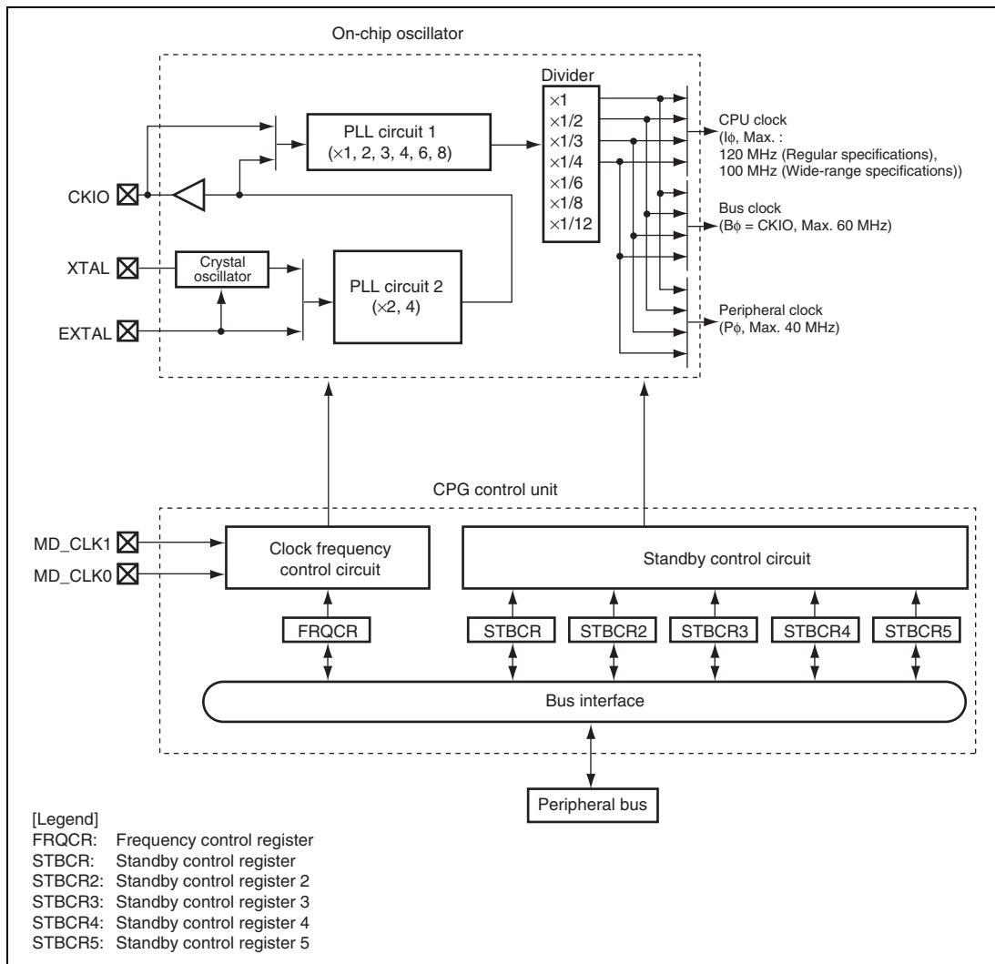
Figure 4.1 Block Diagram of Clock Pulse Generator
