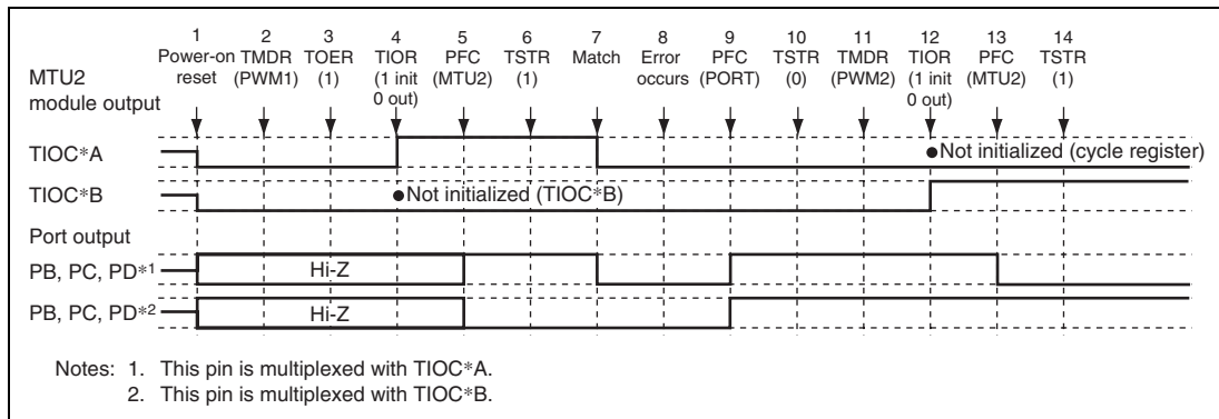
Figure 12.135 Error Occurrence in PWM Mode 1, Recovery in PWM Mode 2
