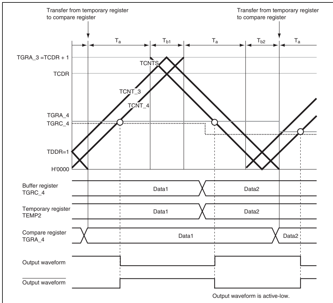
Figure 12.41 Example of Operation without Dead Time
