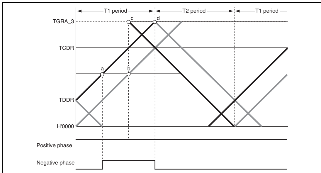
Figure 12.51 Example of Complementary PWM Mode 0% and 100% Waveform Output (3)
