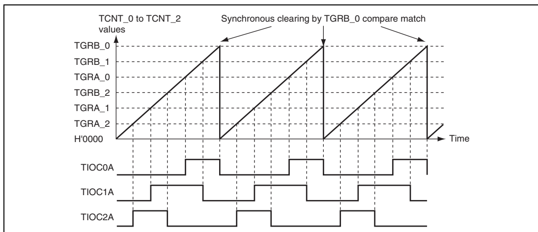
Figure 12.13 Example of Synchronous Operation
