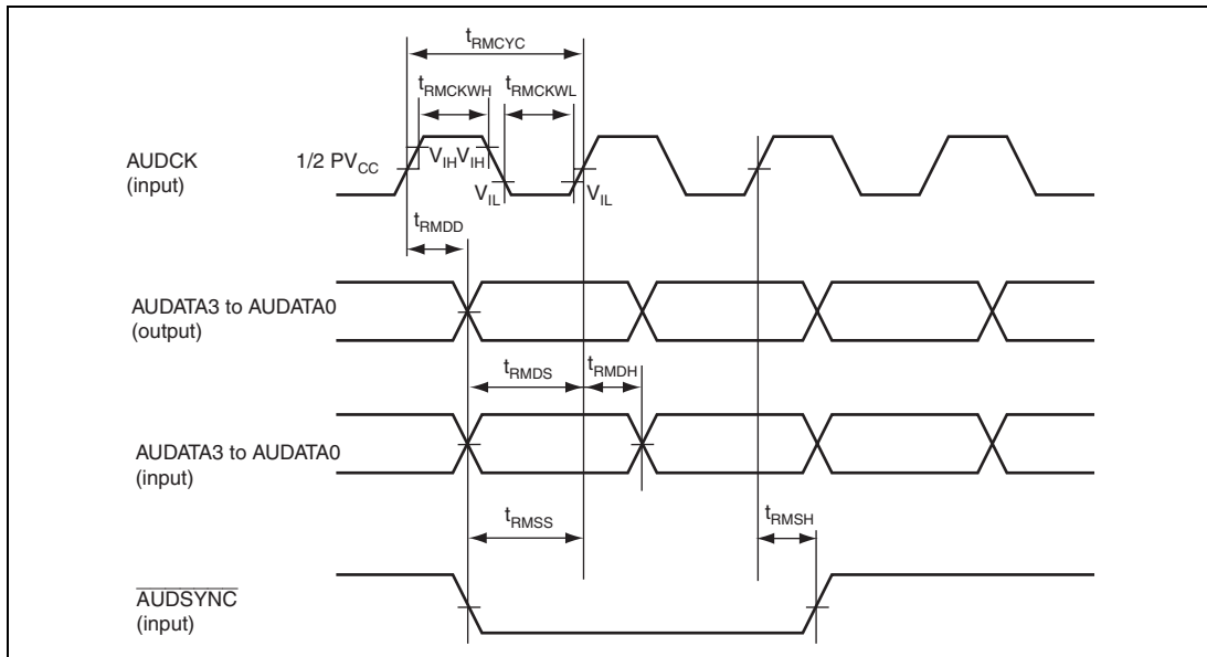
Figure 29.47 RAM Monitor Timing
