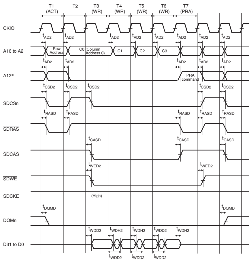
Figure 29.18 Multiple Write Bus Timing for SDRAM Space (Four Data Access, DCL = 2 (Two Cycles), DRCD = 1 (Two Cycles), DPCG = 1 (Two Cycles))
