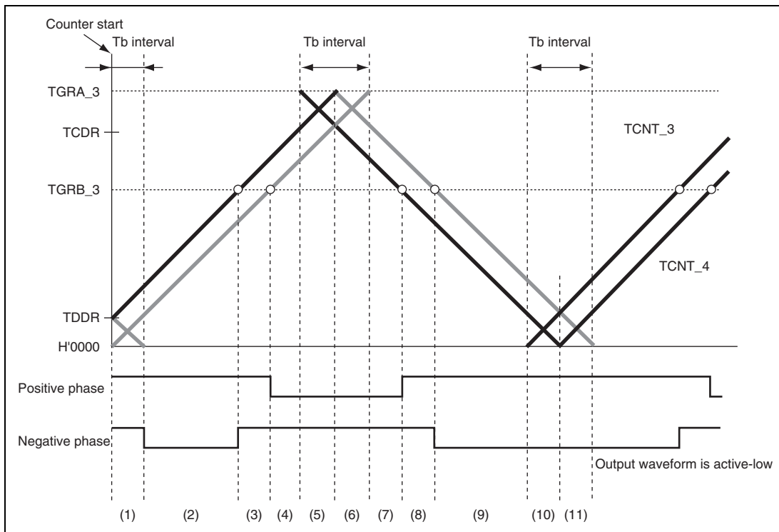
Figure 12.56 Timing for Synchronous Counter Clearing
