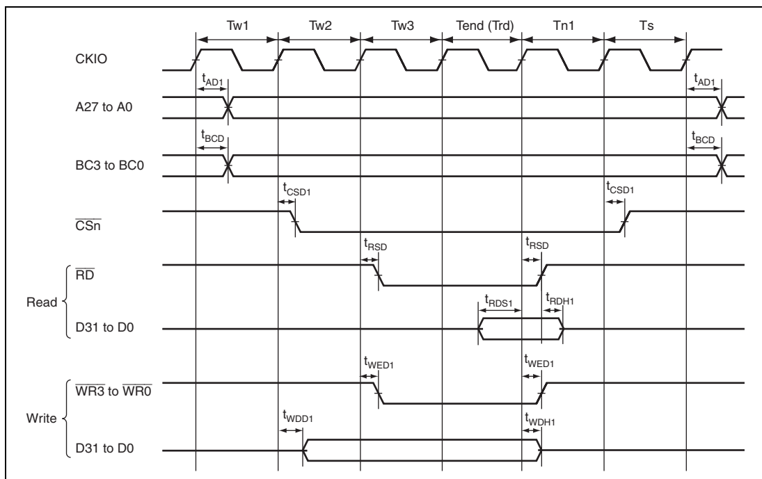
Figure 29.10 (1) External Address Space: Basic Bus Timing (Normal Access, Read/Write Cycle Wait = 3, CS Assert Wait = 1, Write Data Output Wait = 1, WR/RD Assert Wait = 2, Write Data Output Delay Cycles = 0, Read/Write CS Delay Cycles = 1)
