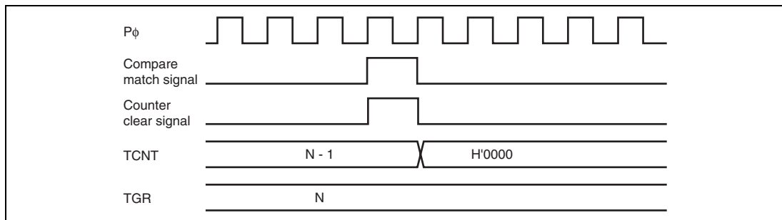
Figure 12.91 Counter Clear Timing (Compare Match) (Channel 5)
