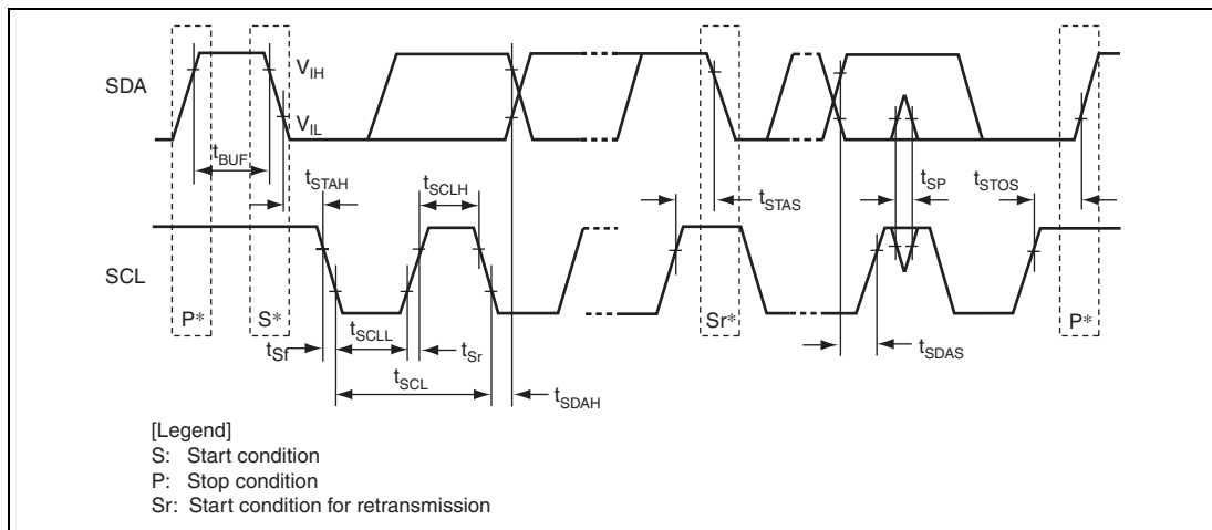
Figure 29.33 I²C Bus Interface 3 Input/Output Timing
