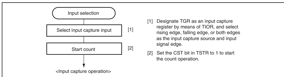
Figure 12.10 Example of Input Capture Operation Setting Procedure
