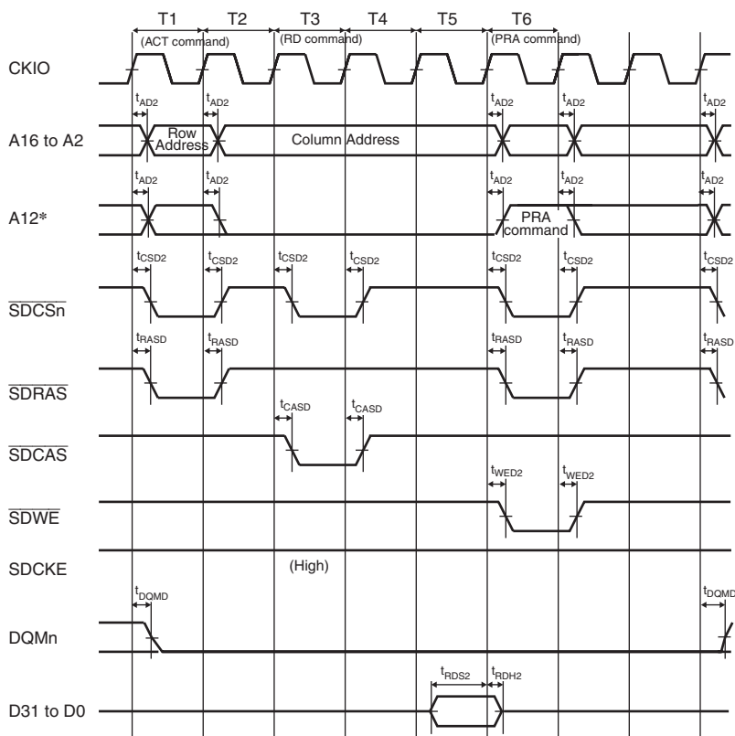
Figure 29.15 Single Read Bus Timing for SDRAM Space (DCL = 2 (Two Cycles), DRCD = 1 (Two Cycles), DPCG = 1 (Two Cycles))
