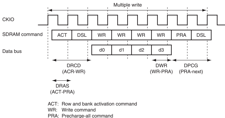
Figure 9.34 Multiple Write Timing Example 2
