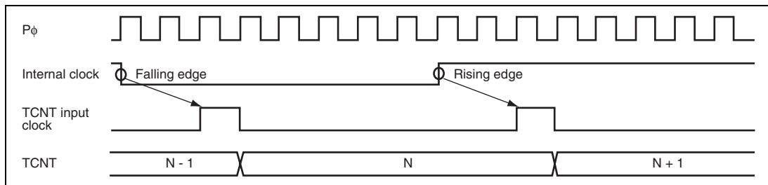
Figure 12.83 Count Timing in Internal Clock Operation (Channels 0 to 4)
