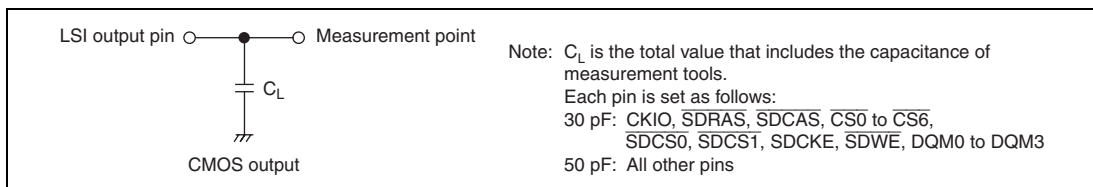
Figure 29.48 Measurement Circuit
