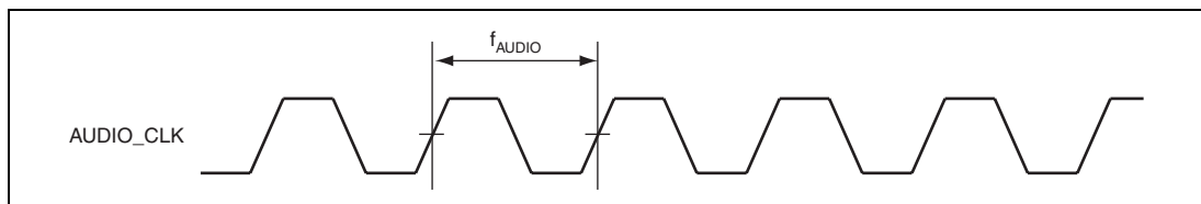
Figure 29.39 AUDIO_CLK Input Timing
