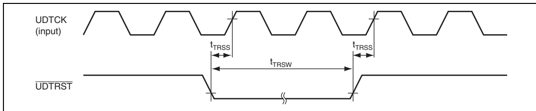
Figure 29.44 UDTRST Input Timing
