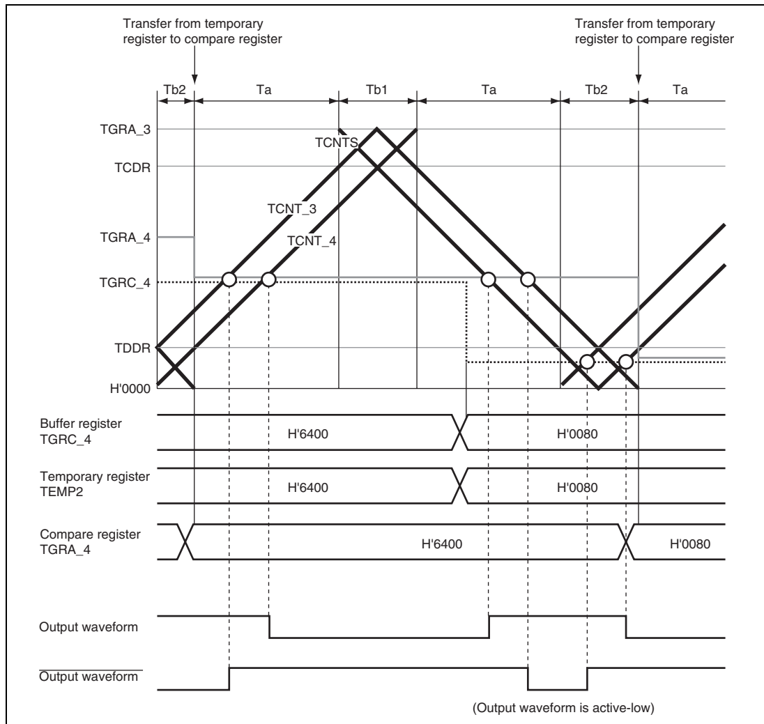
Figure 12.40 Example of Complementary PWM Mode Operation
