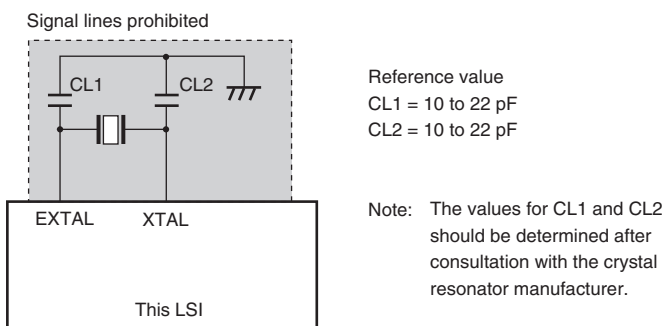
Figure 4.3 Note on Using Crystal Resonator
