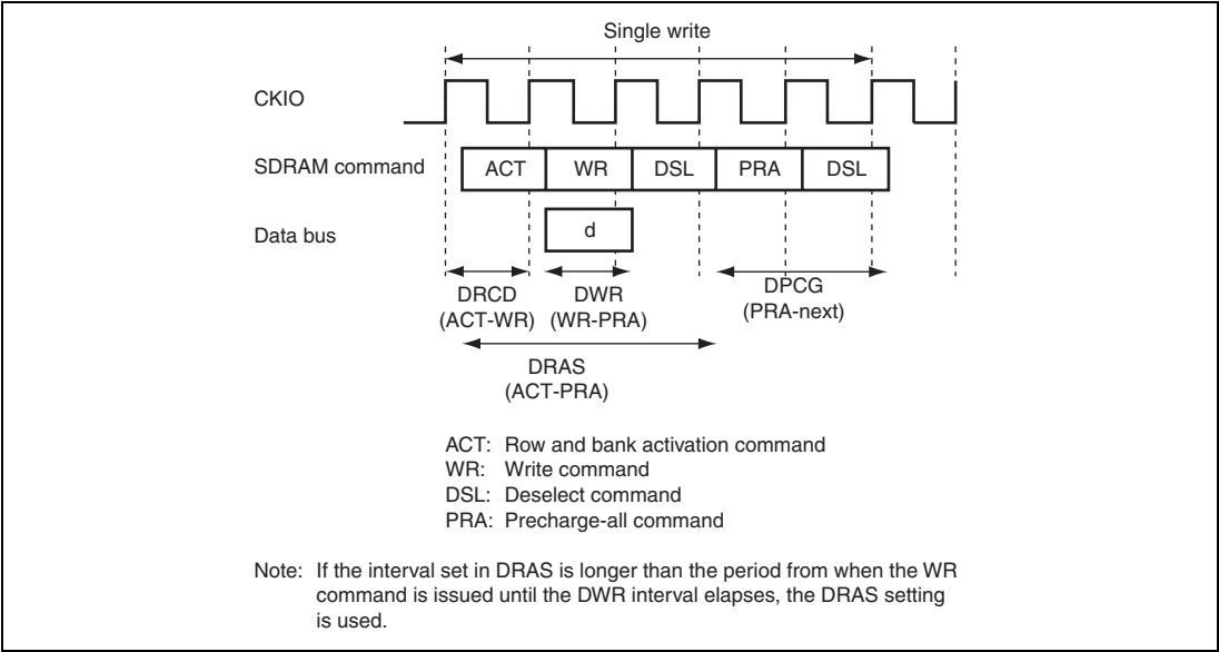
Figure 9.39 Single Write Timing Example 1
