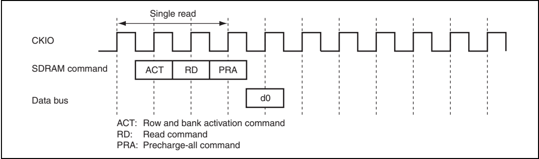
Figure 9.19 Single Read Timing Example (Shortest Timing Settings)
