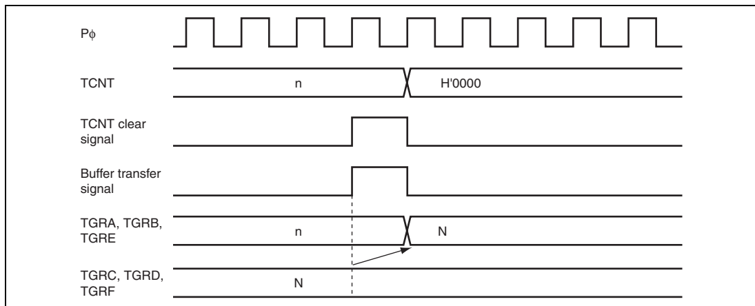
Figure 12.95 Buffer Transfer Timing (when TCNT Cleared)
