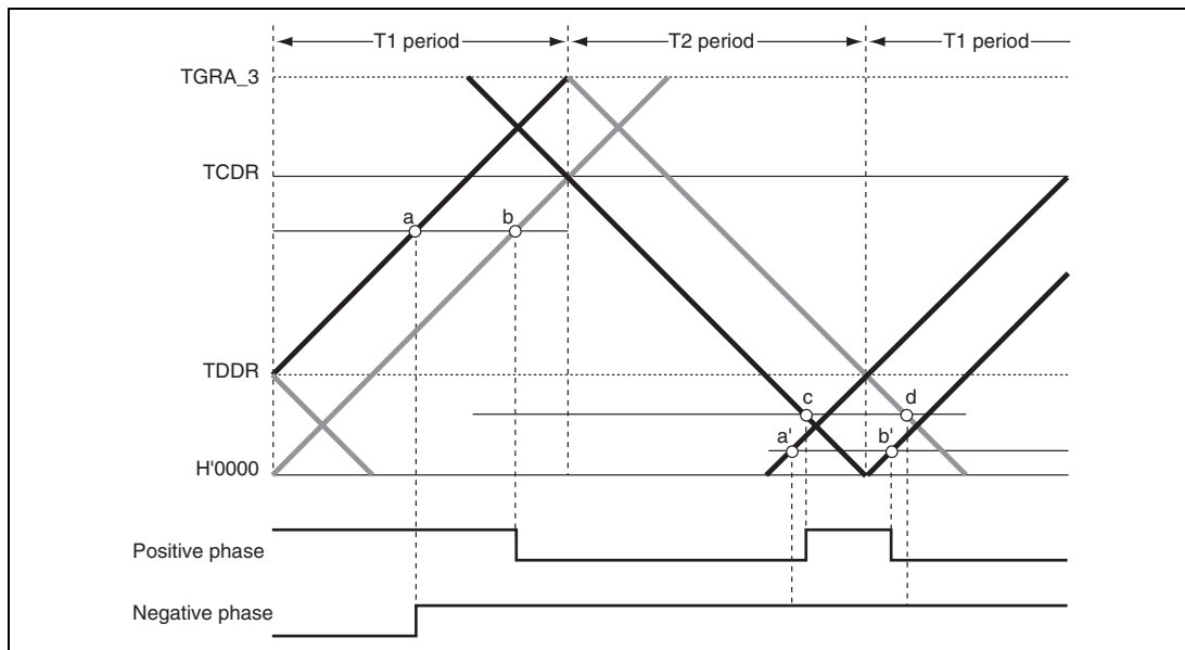
Figure 12.48 Example of Complementary PWM Mode Waveform Output (3)
