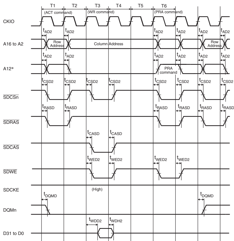
Figure 29.16 Single Write Bus Timing for SDRAM Space (DCL = 2 (Two Cycles), DRCD = 1 (Two Cycles), DPCG = 1 (Two Cycles))
