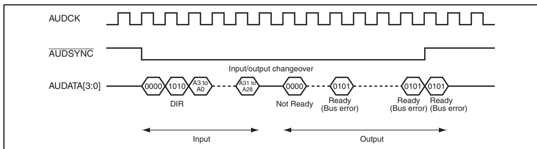
Figure 27.4 Example of Error Occurrence (Longword Read)
