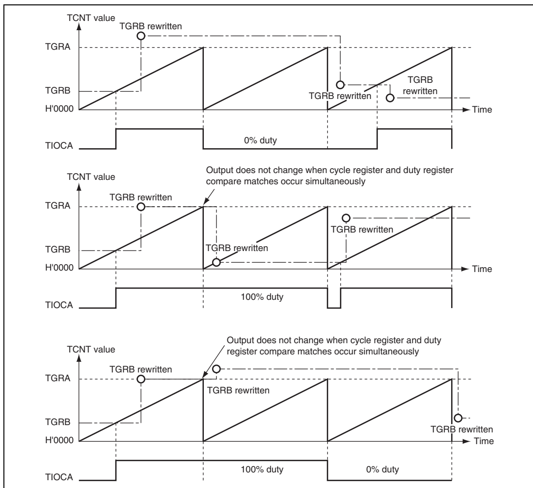
Figure 12.28 Example of PWM Mode Operation (3)
