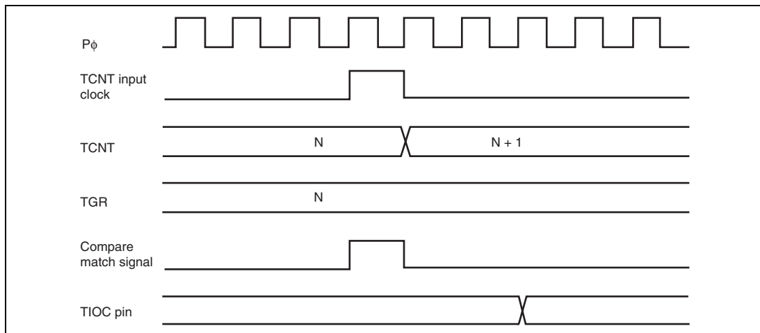
Figure 12.88 Output Compare Output Timing (Complementary PWM Mode/Reset Synchronous PWM Mode)
