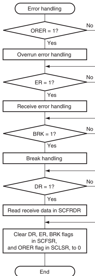
Figure 16.7 Sample Flowchart for Receiving Serial Data (cont)
