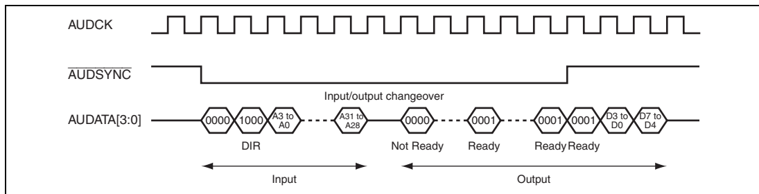
Figure 27.2 Example of Read Operation (Byte Read)
