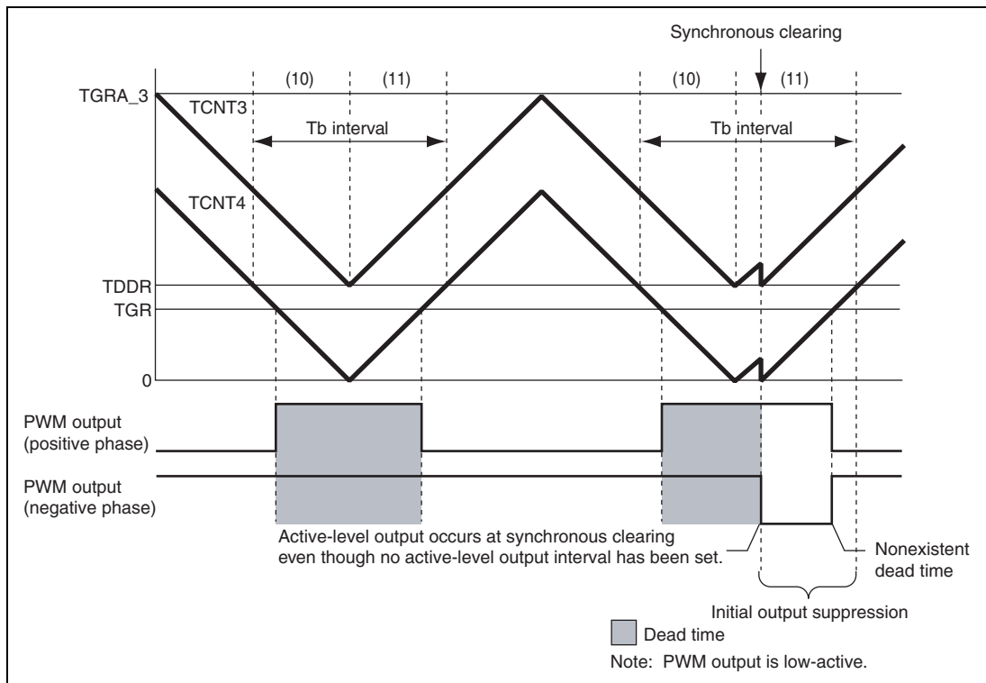
Figure 12.126 Condition (2) Synchronous Clearing Example
