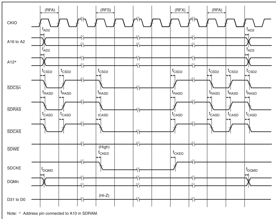
Figure 29.21 Bus Timing for SDRAM Space Self Refresh
