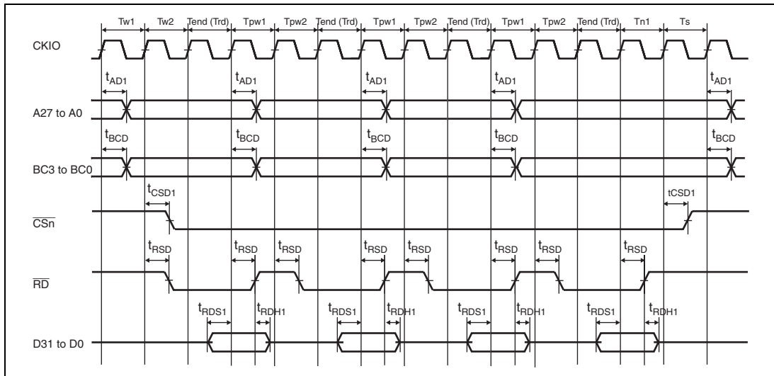
Figure 29.11 External Address Space: Basic Bus Timing
