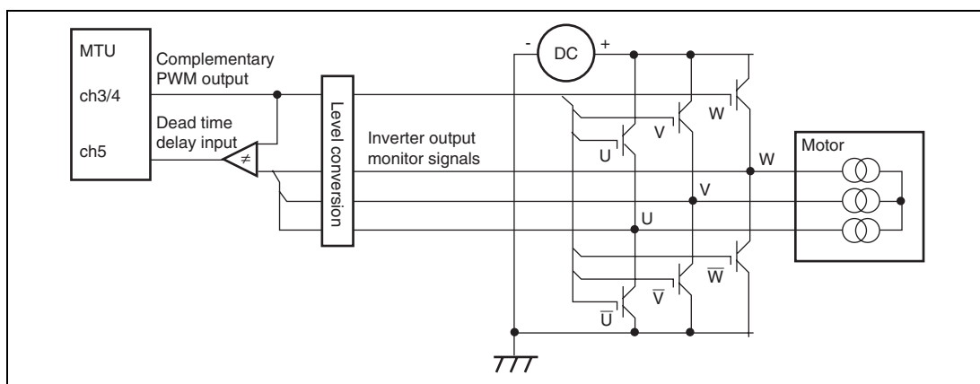
Figure 12.81 Example of Motor Control Circuit Configuration
