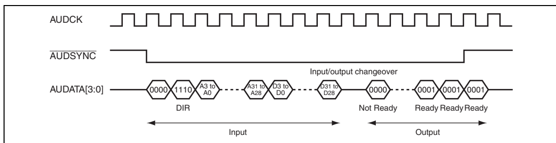
Figure 27.3 Example of Write Operation (Longword Write)
