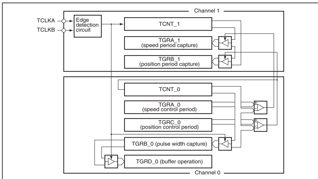
Figure 12.34 Phase Counting Mode Application Example
