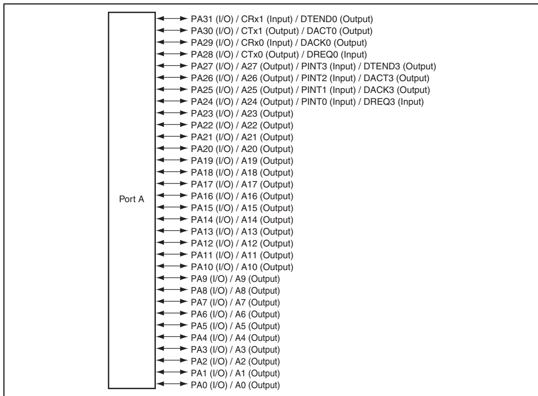
Figure 22.1 Port A
