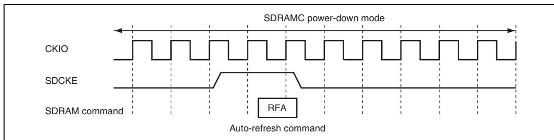
Figure 9.12 Auto-Refresh Operation in SDRAMC Power-Down Mode
