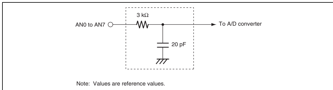
Figure 20.9 Analog Input Pin Equivalent Circuit
