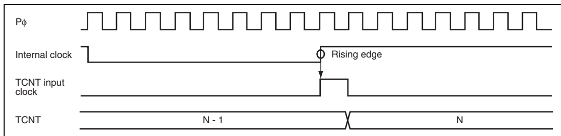
Figure 12.84 Count Timing in Internal Clock Operation (Channel 5)
