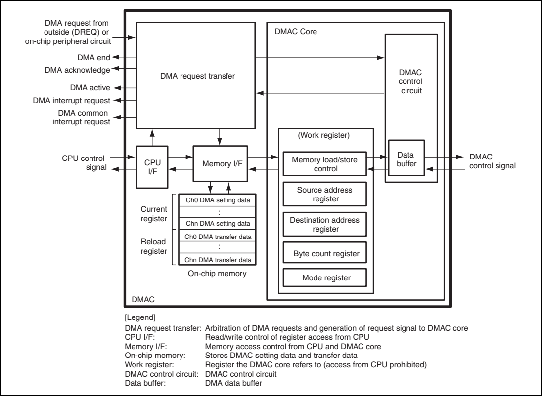
Figure 11.1 DMAC Block Diagram
