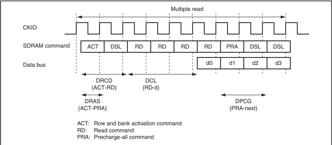
Figure 9.32 Multiple Read Timing Example 3
