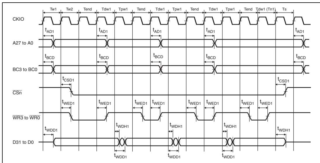
Figure 29.13 External Address Space: Basic Bus Timing
