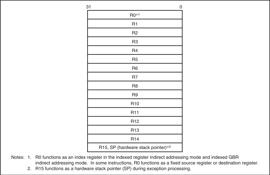
Figure 2.1 General Registers
