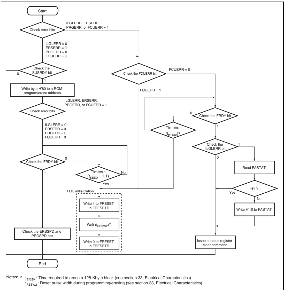
Figure 27.24 Procedure for Programming/Erase Suspension
