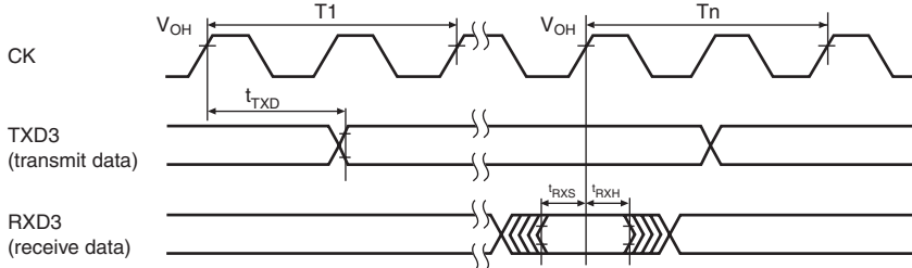
Figure 33.48 SCIF Input/Output Timing
