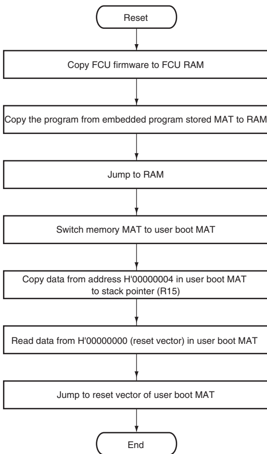
Figure 27.34 Overview of Boot Sequence in User Boot Mode
